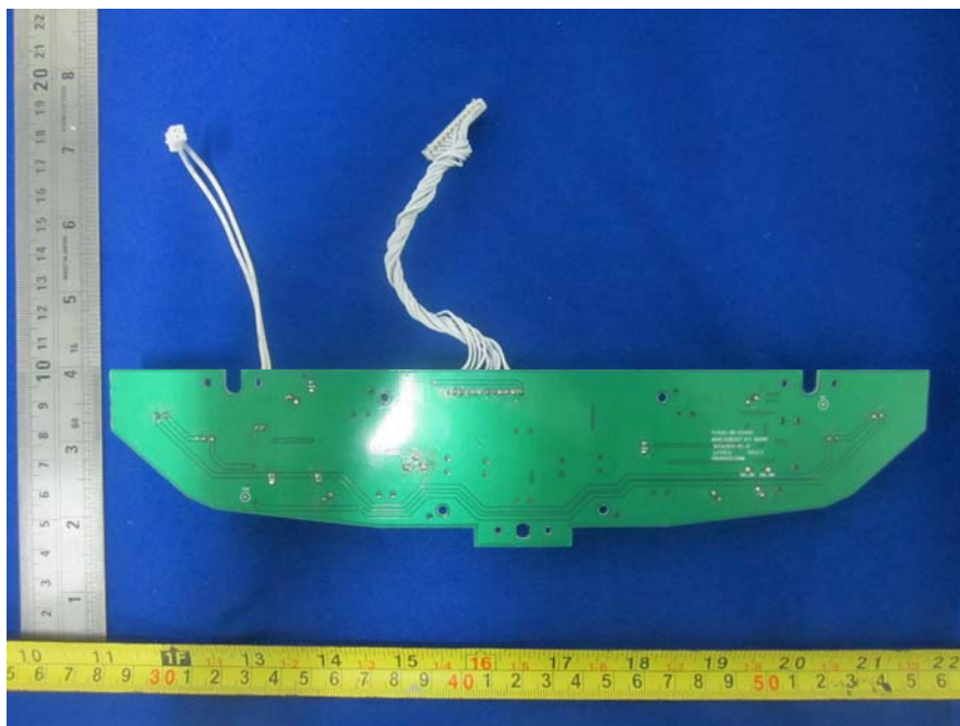
EUT – Botton Board Bottom View
