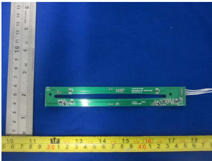
EUT – DVD Sensor Board Top View
