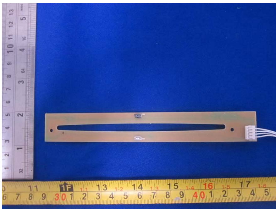
EUT – DVD Sensor Board Bottom View
