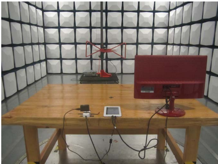
Radiated Emission Below 1GHz - Rear View (HDMI Playing)
