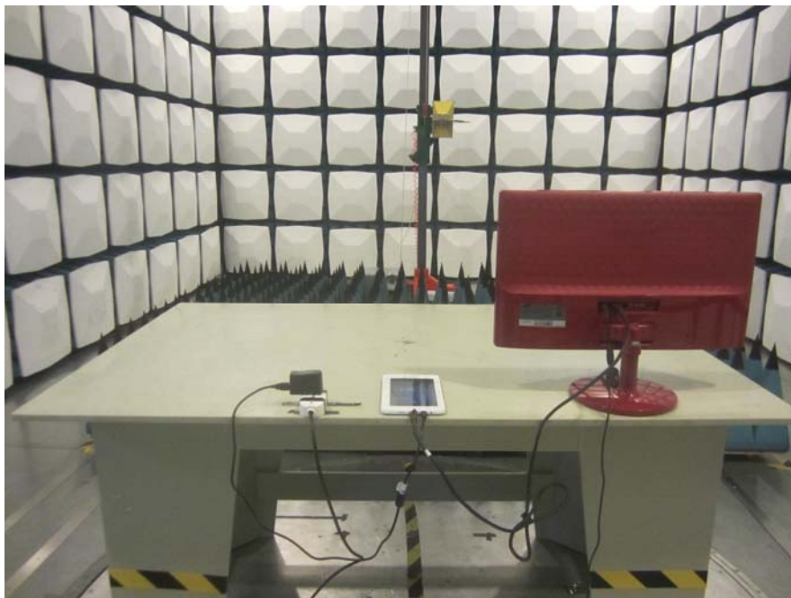
Radiated Emission Above 1GHz - Rear View (HDMI Playing)
