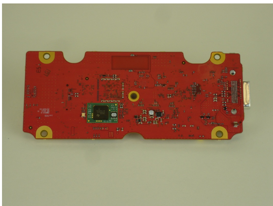
Logic Board Bottom
