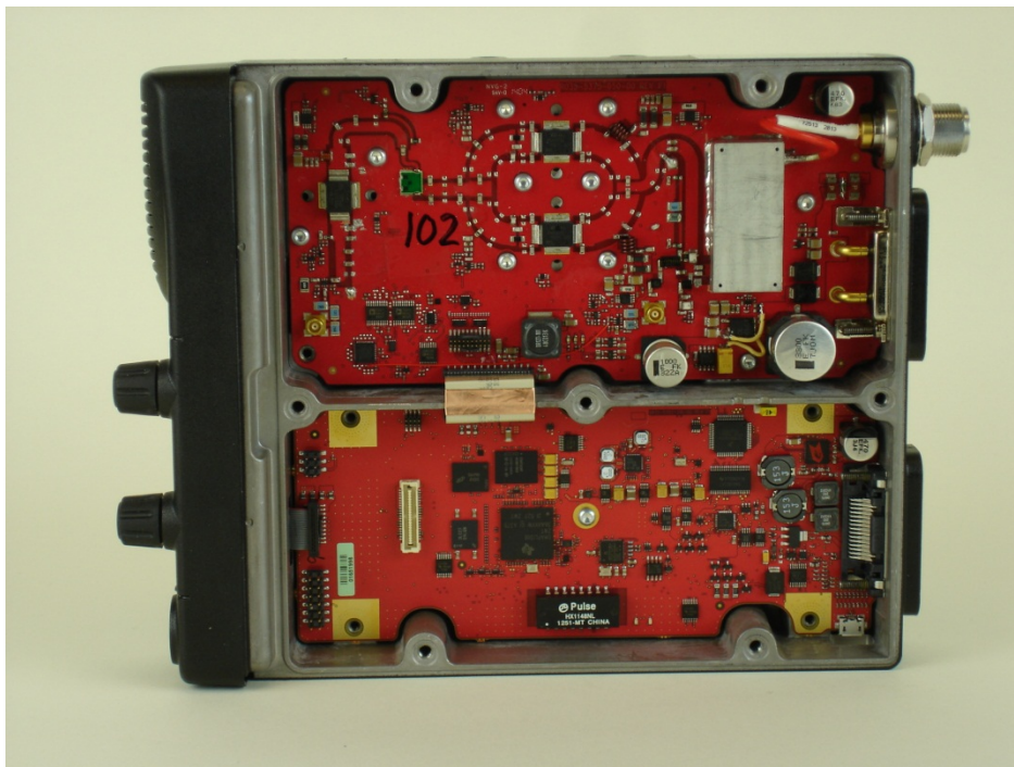
Radio with RF Module Removed
