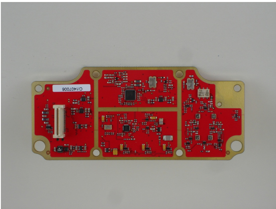
RF Board Bottom
