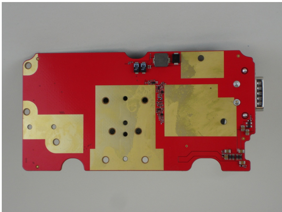
Transmitter Power Amplifier Board Bottom
