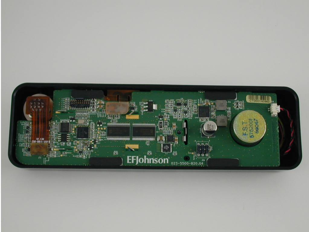
Front Panel with Display Board Installed
