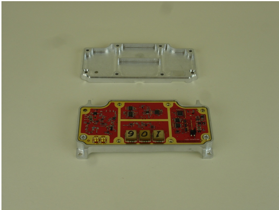
RF Board in Chassis with Cover Removed
