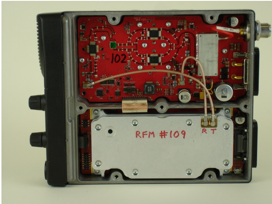
Radio with Bottom Cover Removed
