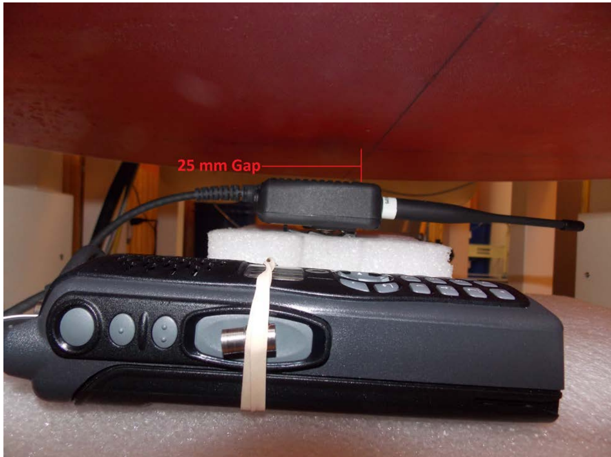
Audio Accessory B Face Configuration
