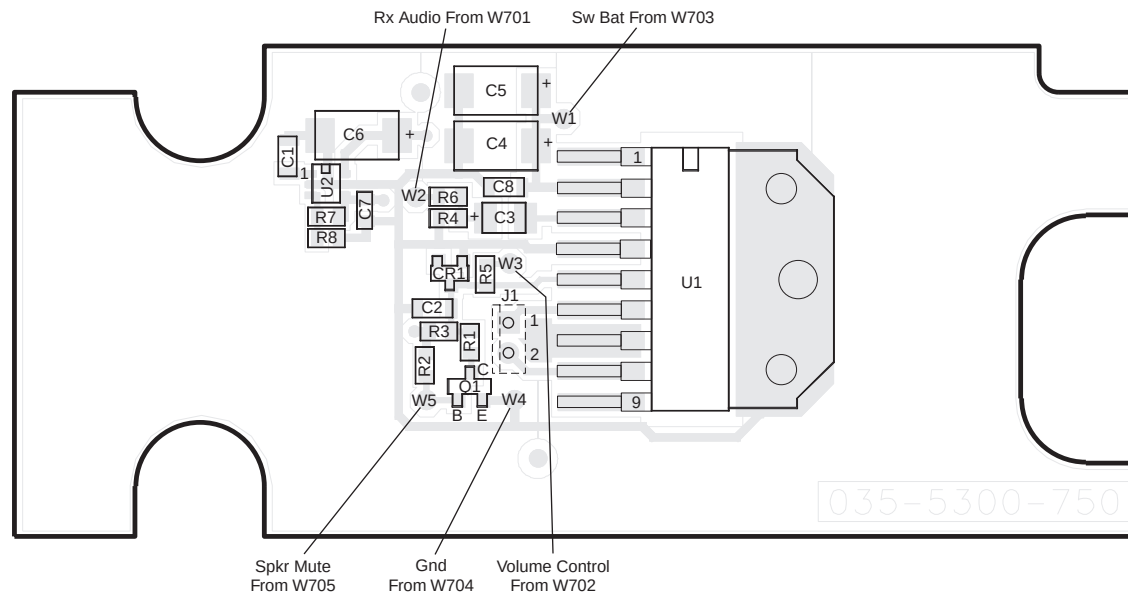
REMOTE CONTROL UNIT AUDIO PA BOARD LAYOUT
