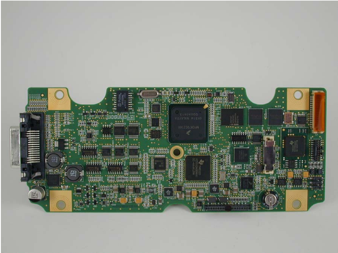
Logic board front
