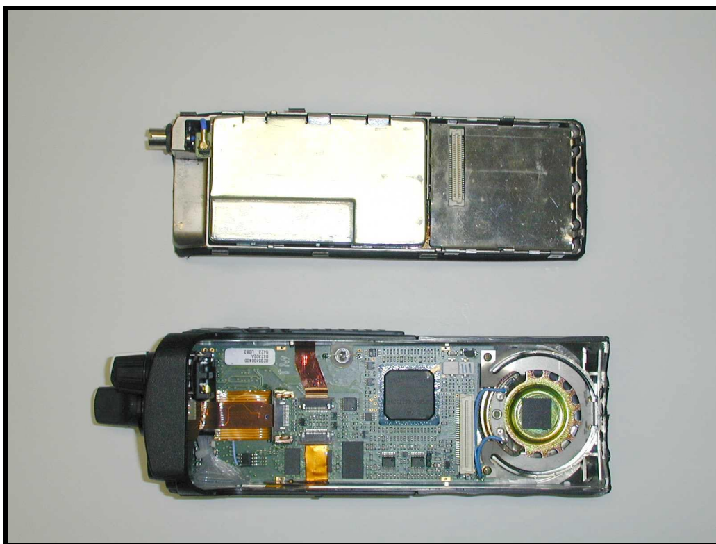
PHOTOGRAPH 13: OPEN SHIELDS VIEW
