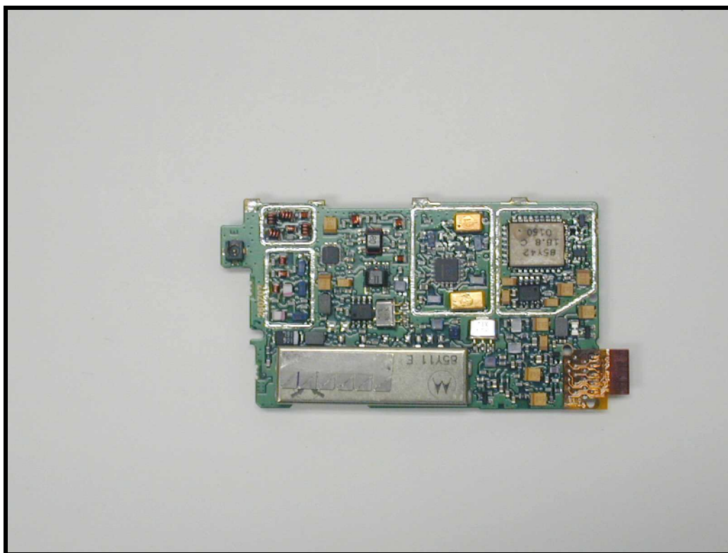
PHOTOGRAPH 14: RF TOP VIEW
