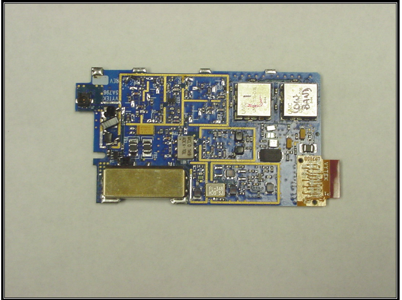
PHOTOGRAPH 19: RF BOARD TOP
