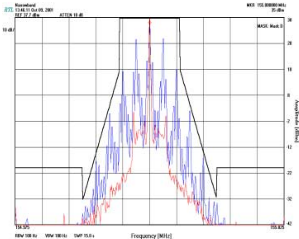
PLOT 5-3: OCCUPIED BANDWIDTH – NARROWBAND: CHANNEL 5: 5W, 12.5 KHZ CHANNEL BANDWIDTH: MASK D (AUDIO MODULATION: 2,500 HZ)
