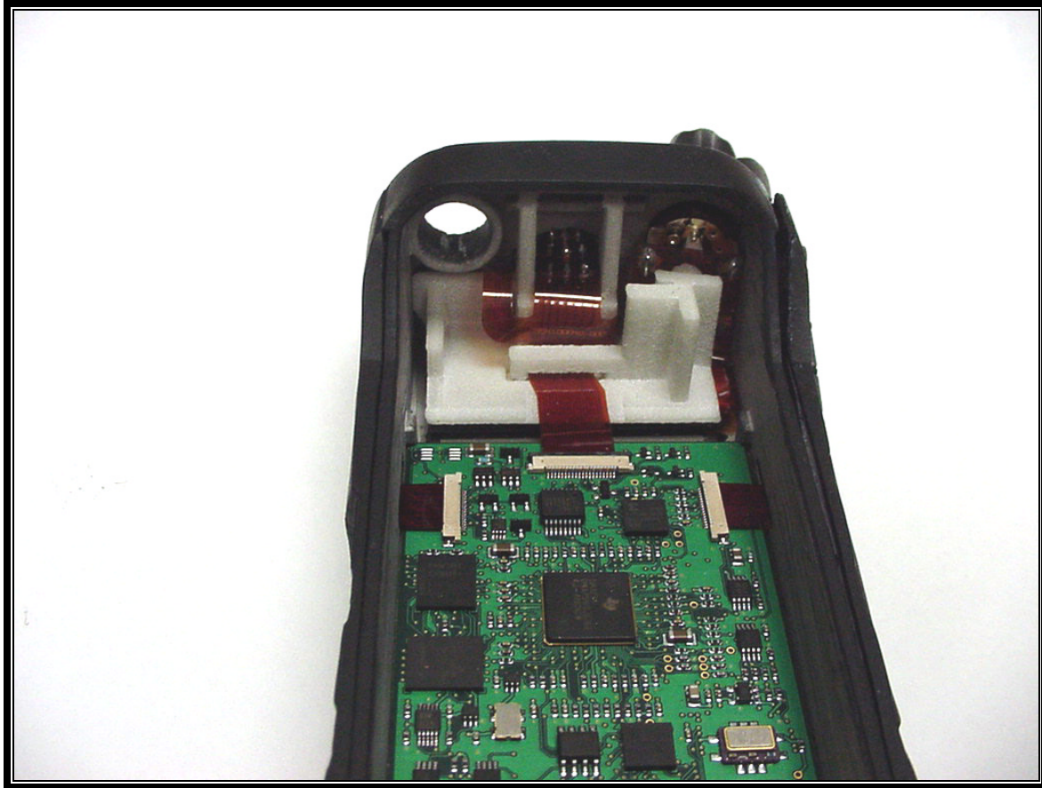
PHOTOGRAPH 17: FRONT COVER WITH DIGITAL BOARD AND CONTROL ASSEMBLY
