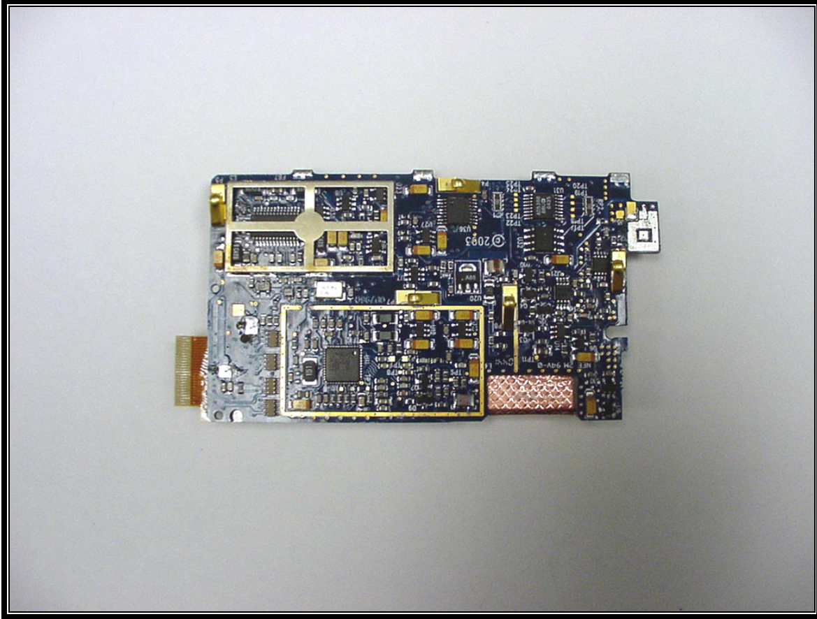
PHOTOGRAPH 14: RF BOARD BOTTOM
