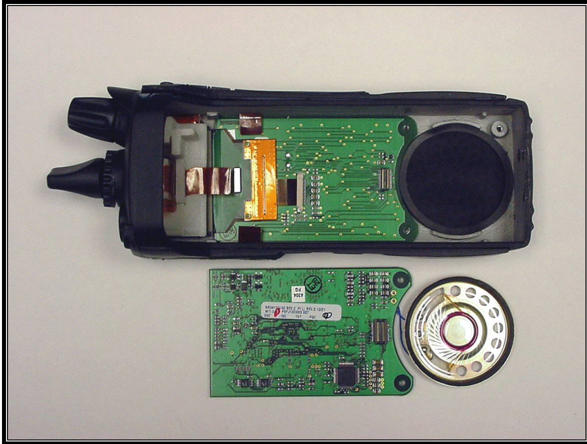
PHOTOGRAPH 18: FRONT COVER WITH DIGITAL BOARD REMOVED
