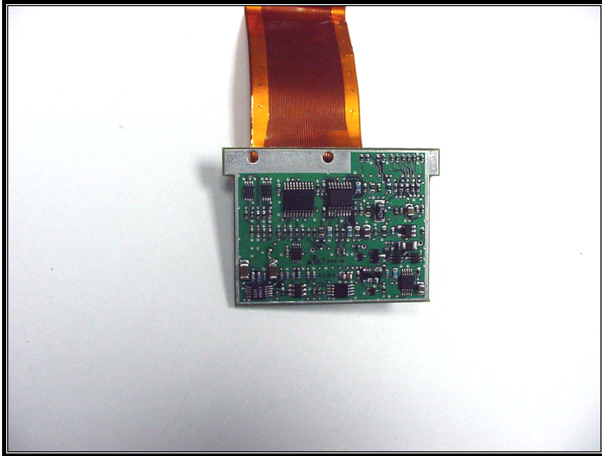
PHOTOGRAPH 13: POWER SUPPLY BOARD BOTTOM
