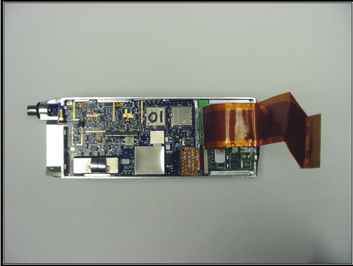
PHOTOGRAPH 11: CHASSIS WITH SHIELDS REMOVED
