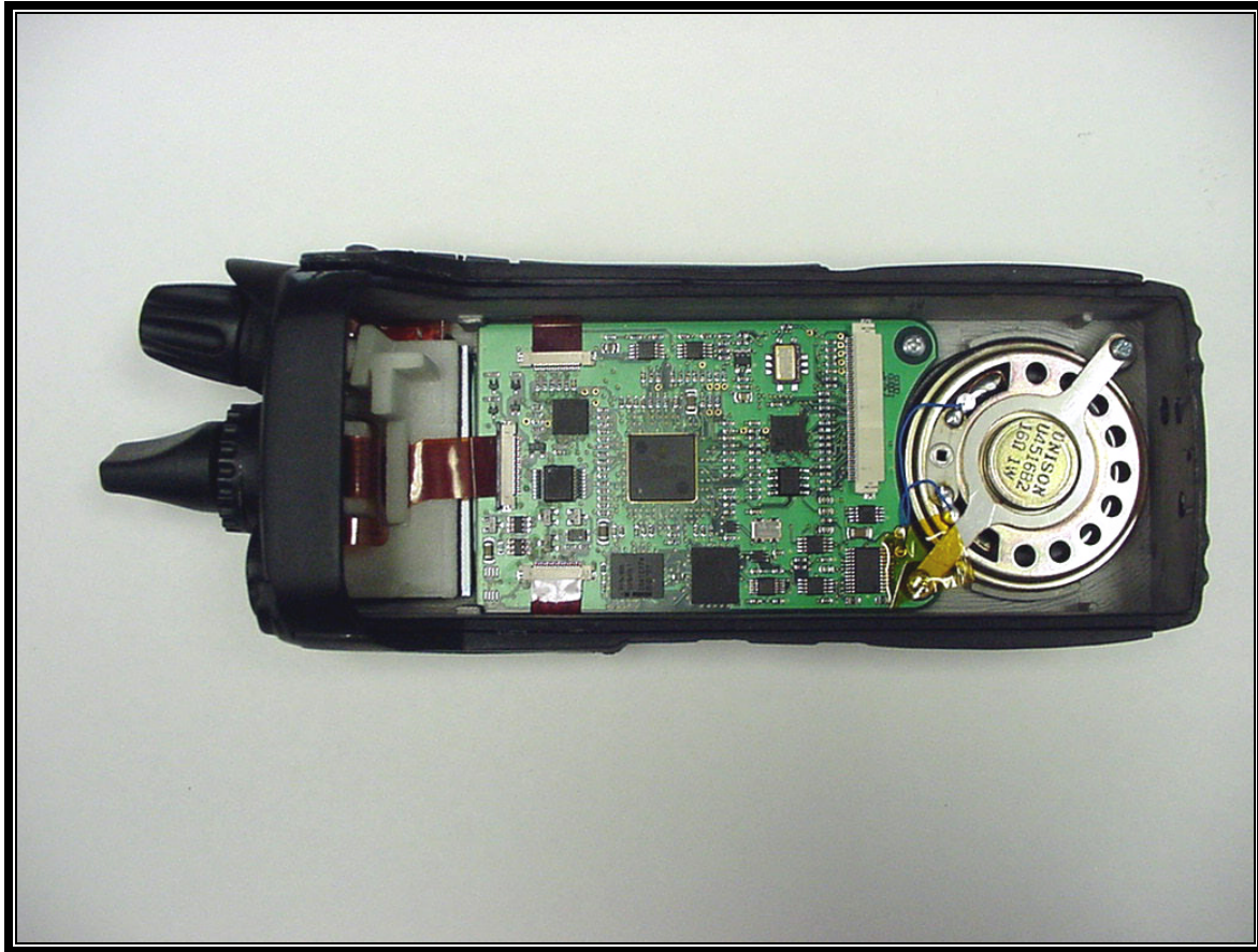
PHOTOGRAPH 16: DIGITAL BOARD IN FRONT COVER
