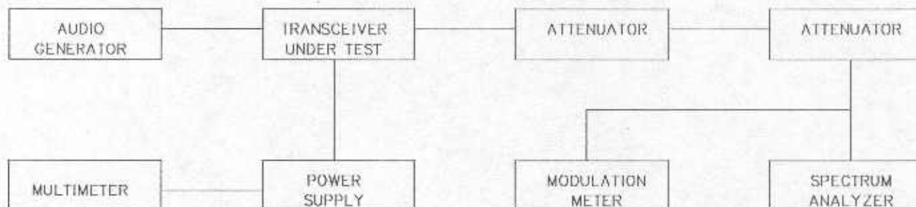
TEST SET-UP
