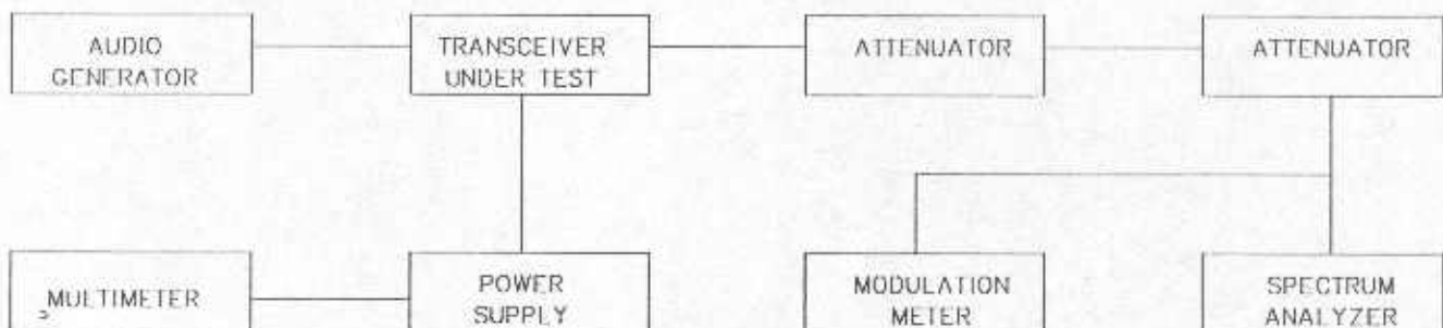
TEST SET-UP
