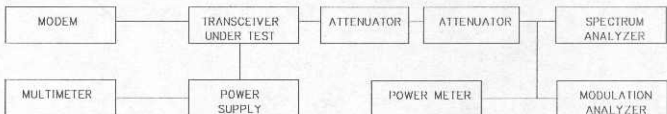
TEST SET-UP
