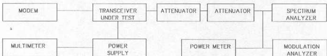
TEST SET-UP
