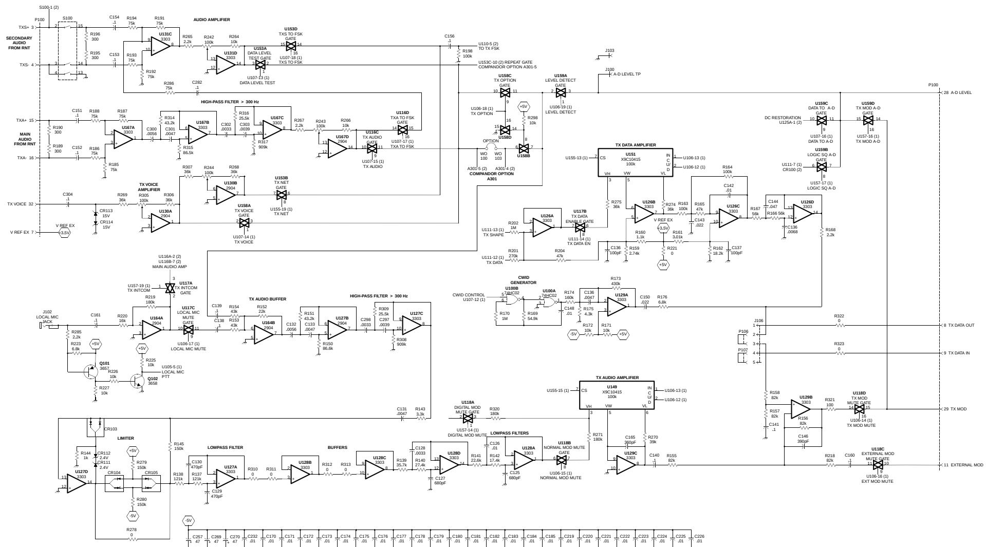
MAIN AUDIO CARD (MAC) SCHEMATIC (3 OF 3)
