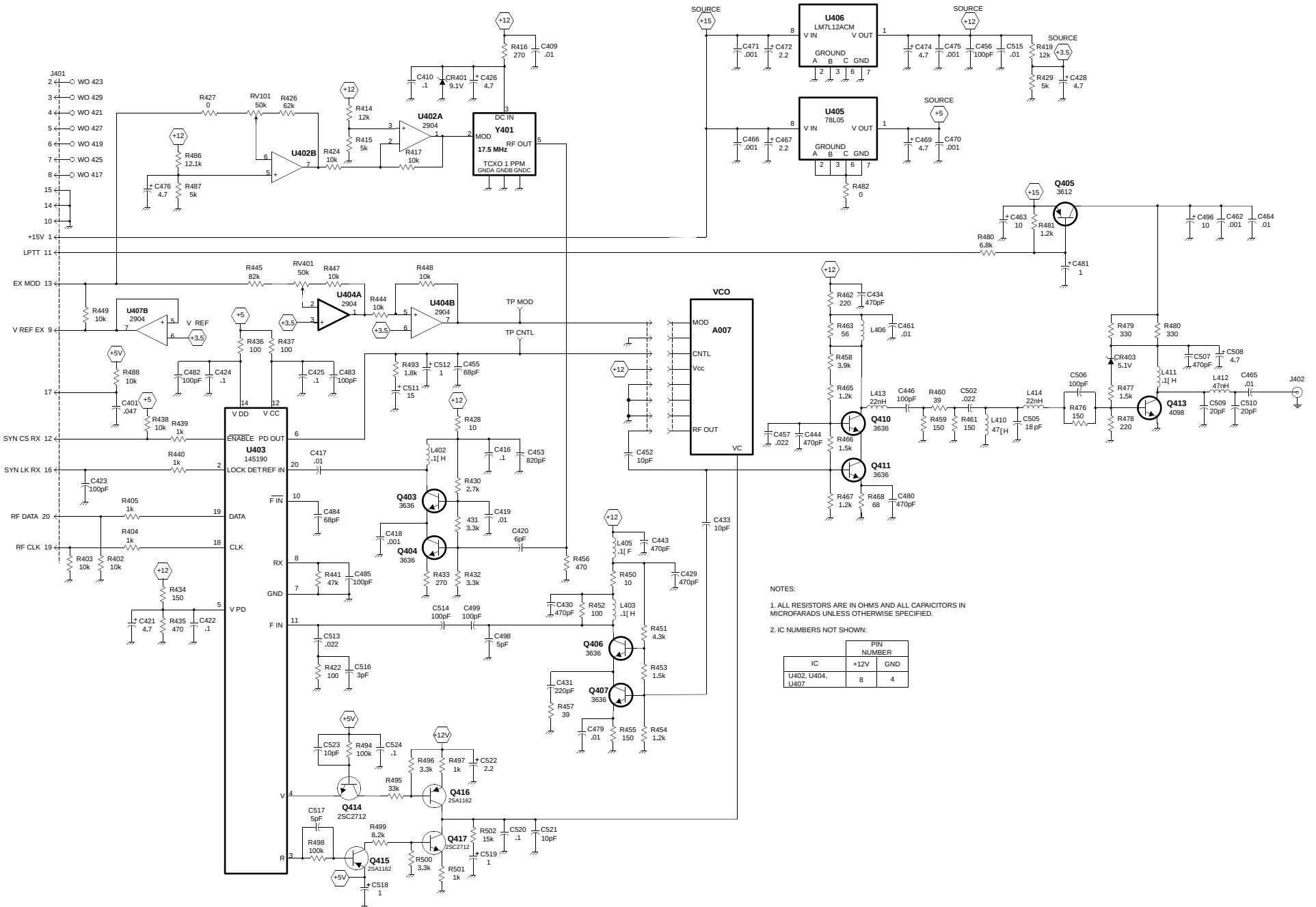
EXCITER SCHEMATIC
