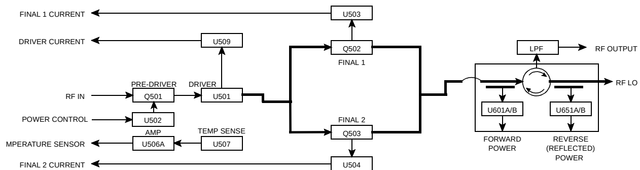
POWER AMPLIFIER BLOCK DIAGRAM
