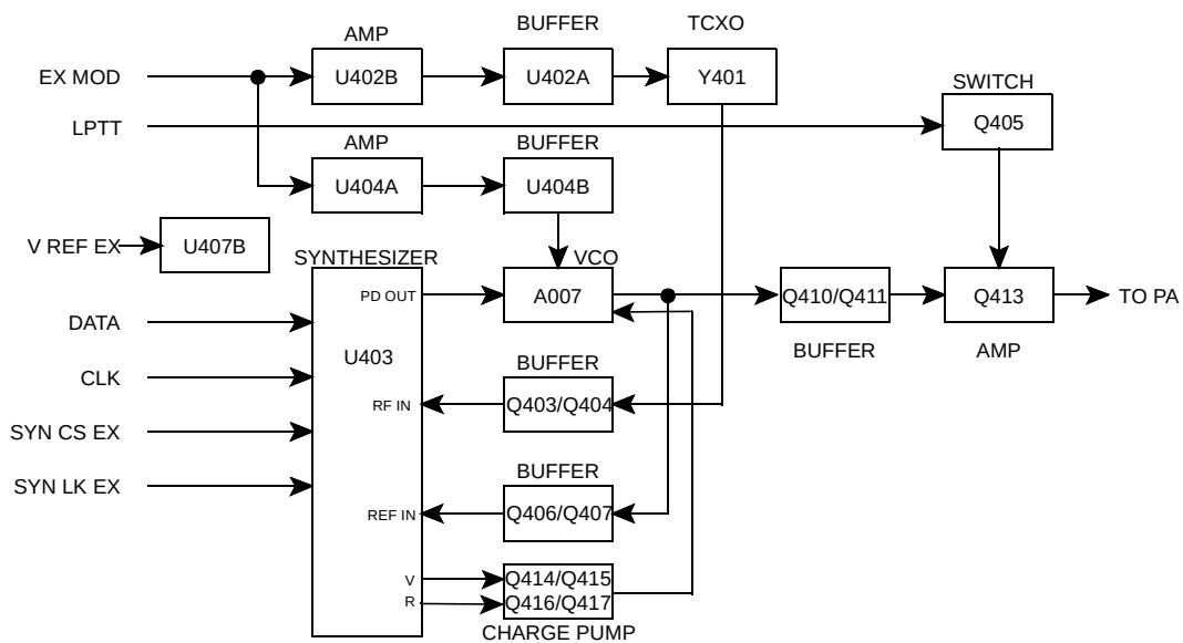
EXCITER BLOCK DIAGRAM
