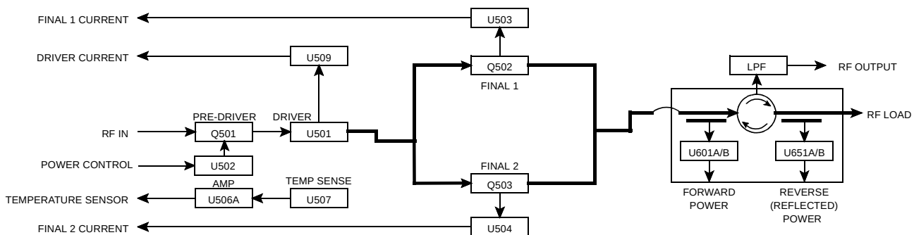
Figure 2 125W POWER AMPLIFIER BLOCK DIAGRAM
