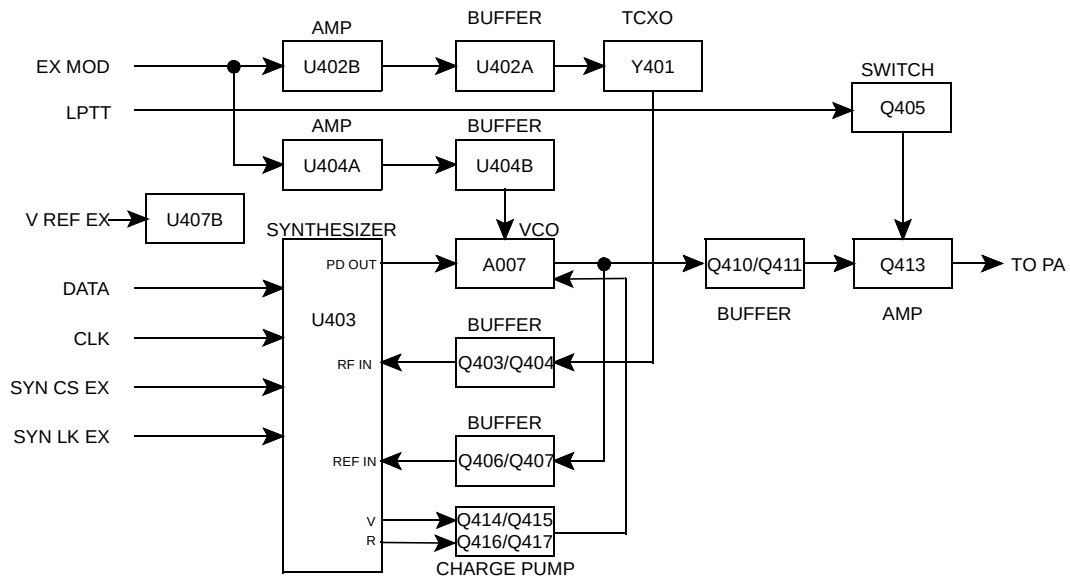
Figure 1 EXCITER BLOCK DIAGRAM
