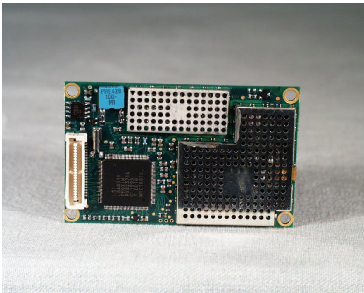
Component side of the RF Module (Rev C)
