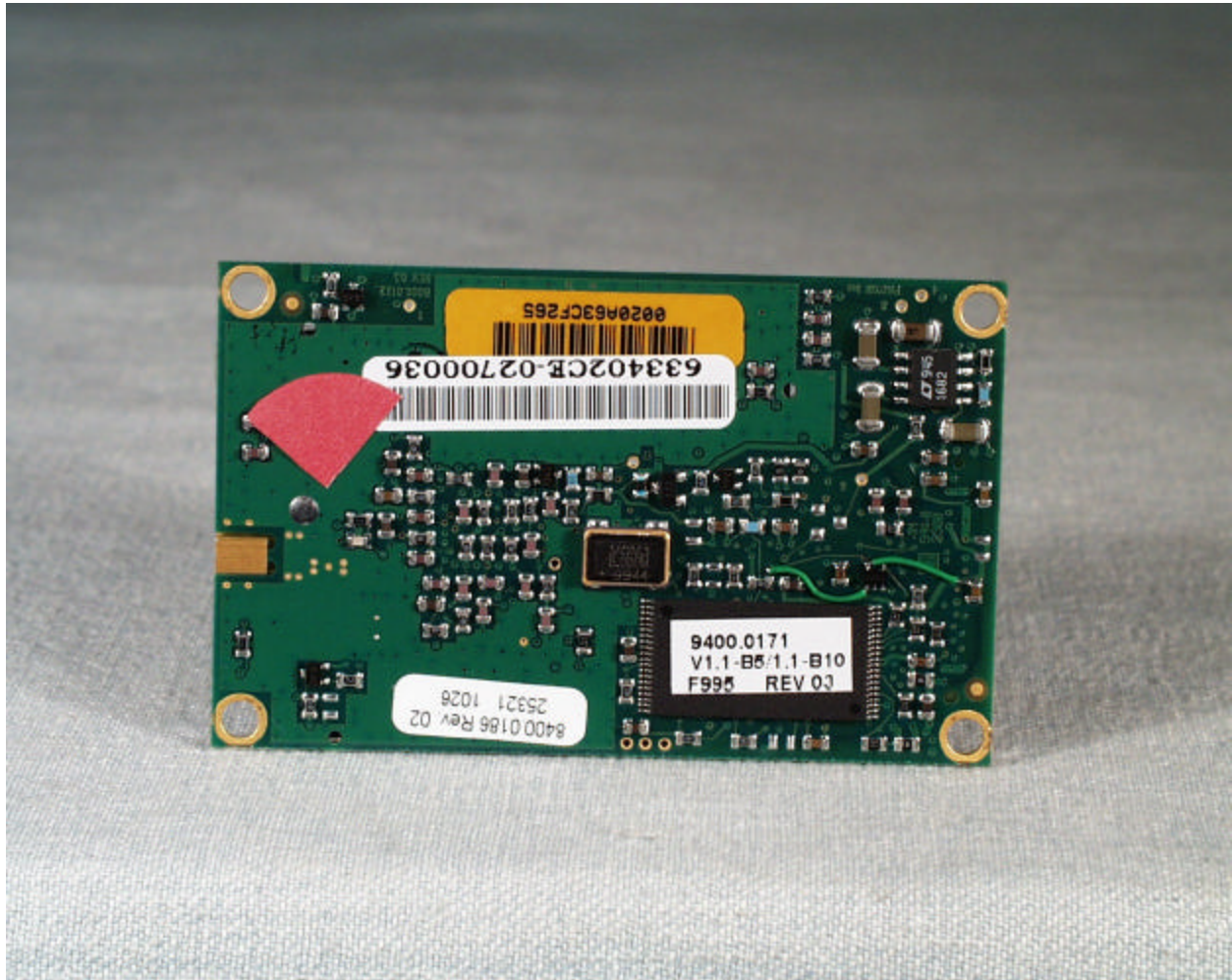
Solder side of RF Module (Rev C)
