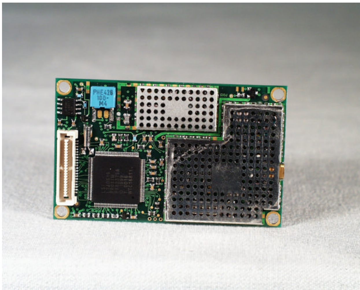
Component side of the RF Module (Rev D)
