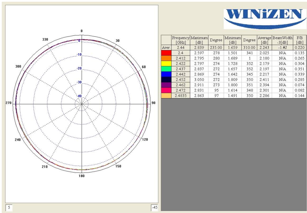
Fig 6. Gain Patterns
