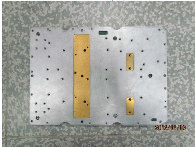
POWER AMPLIFIER (PA) - TOP with COVER REMOVED
