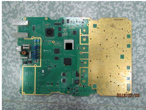
TRANSCIEVER (TRX) - BOTTOM with COVER REMOVED
