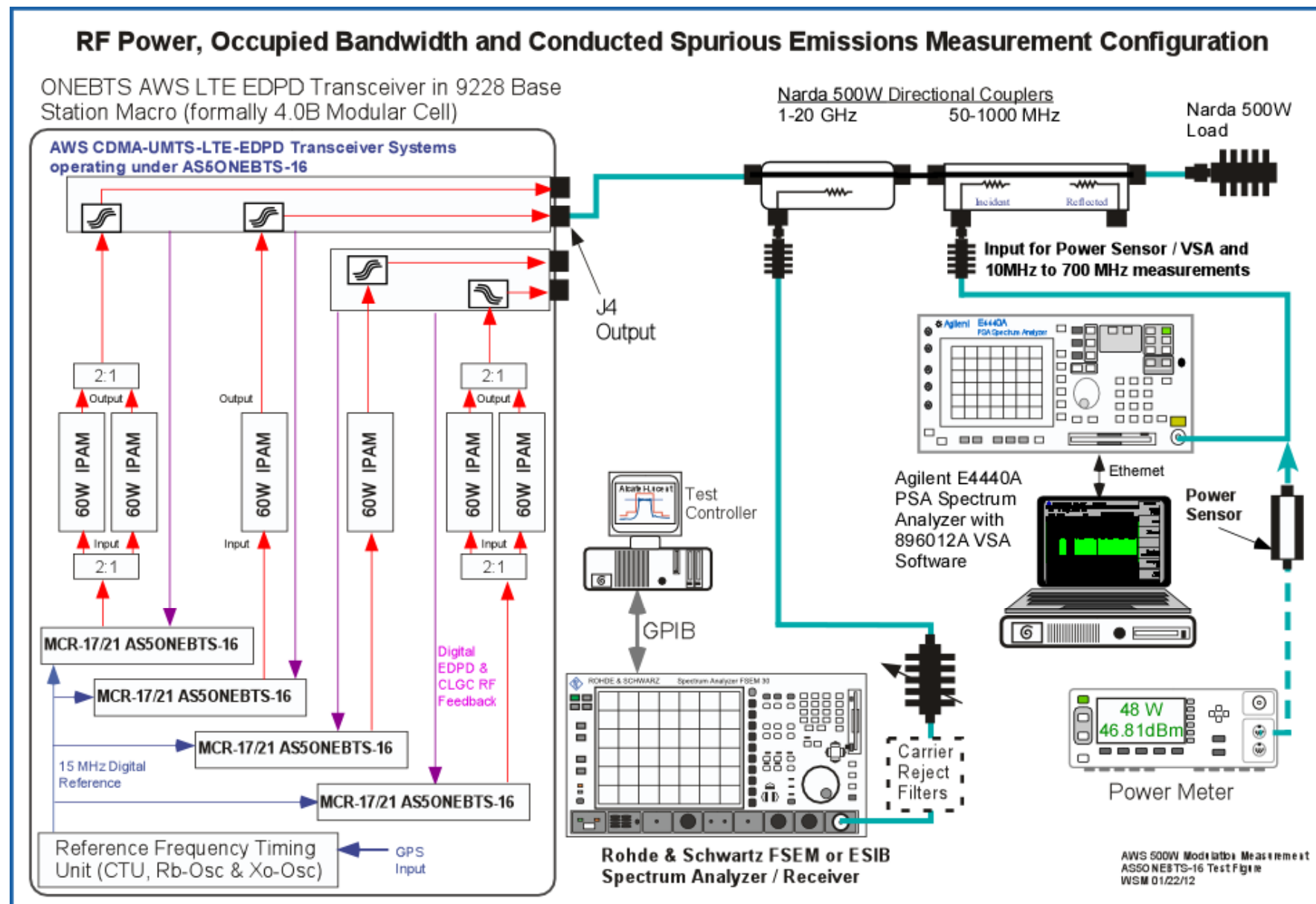
Figure 13A; Test Setup for Antenna Port Measurement of Modulation Characteristics and Code Domain
