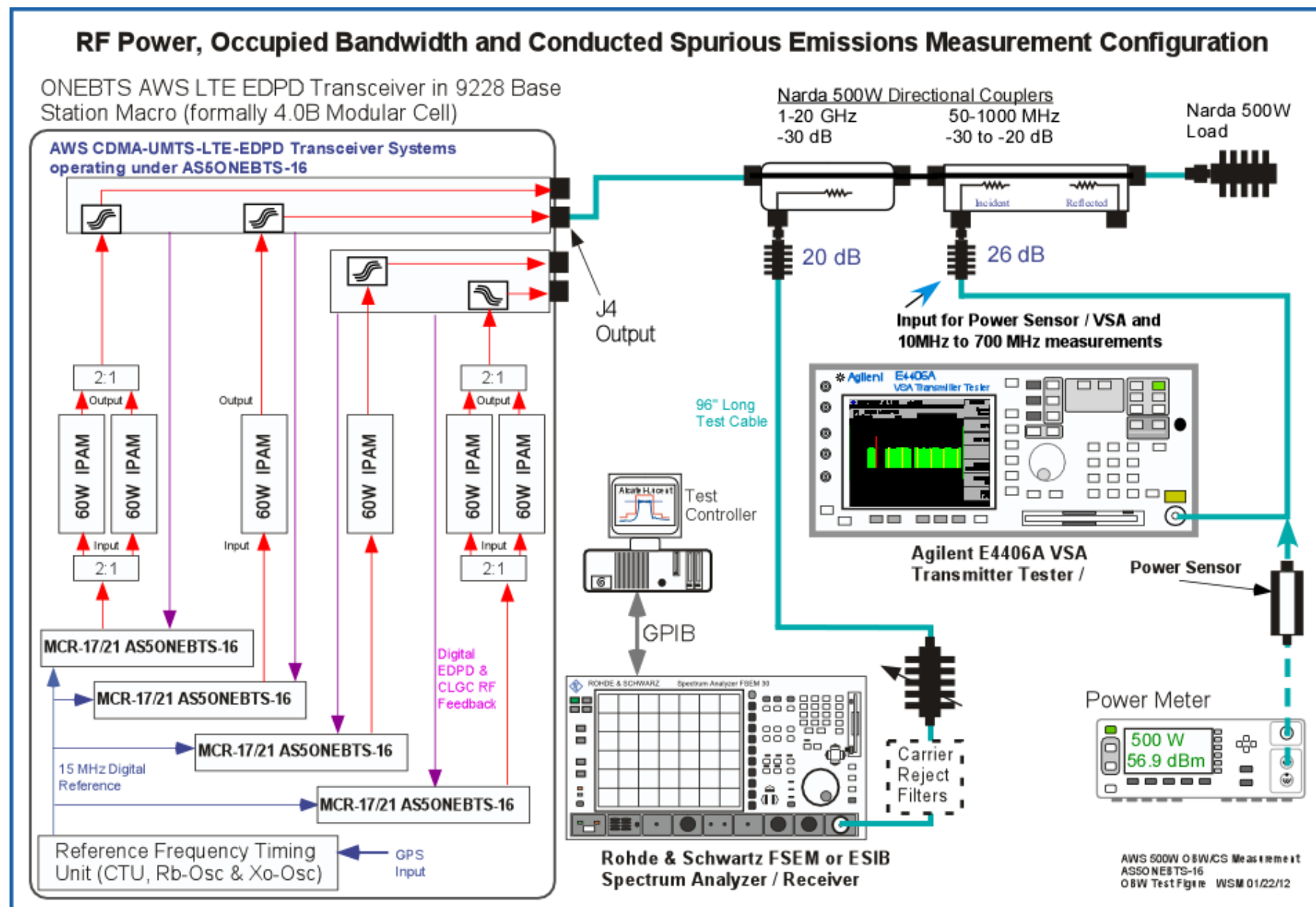
Figure 14A Test Setup for Antenna Port Measurement of Transmit Power, Occupied Bandwidth and Conducted Spurious Emissions
