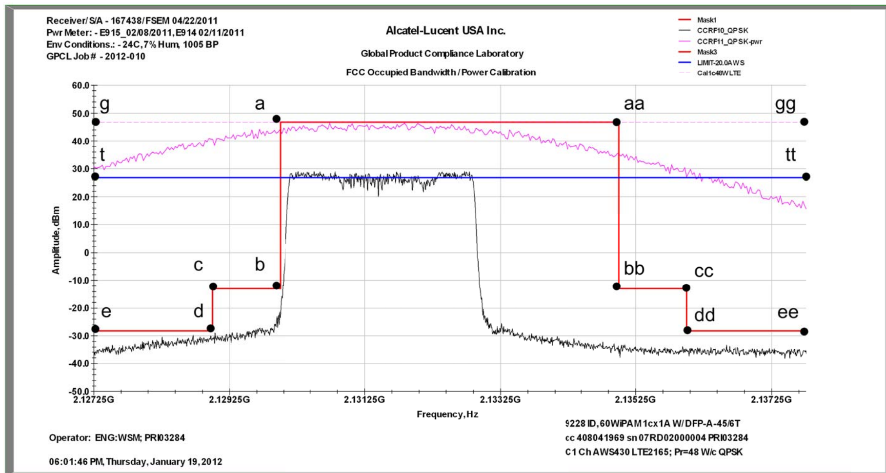
Figure 14B Occupied Bandwidth Mask for AWS Block Operation at 48 W with Power Calibration (AWS C Block is depicted with a single 3 MHz LTE carrier signal showing use of the Power Calibration Trace)
