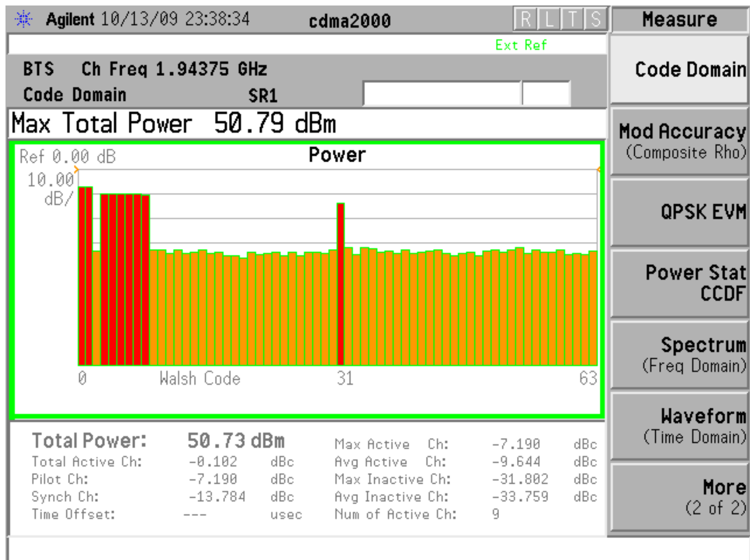
Figure 13B Code Domain 1c A Block, Channel 275 Tx Output 1 Amplifier
