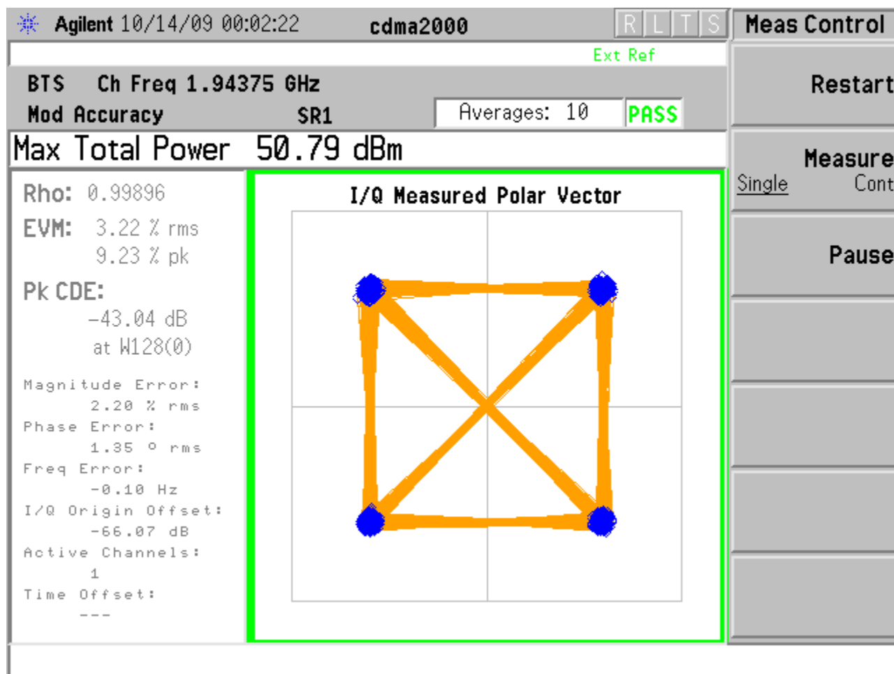
Figure 13C Rho 1c A Block, Channel 275 Tx Output 1 Amplifier
