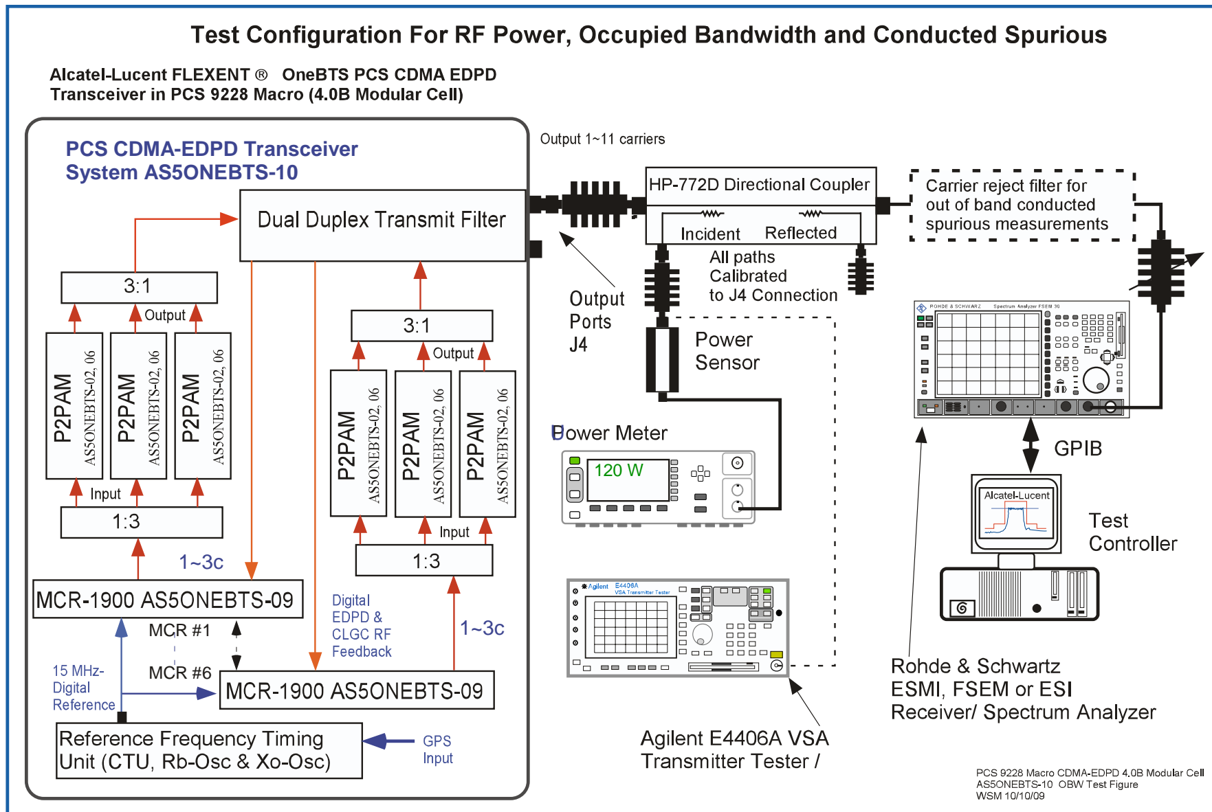
Figure 15A Test Setup for Antenna Port Measurement of Transmit Power, Occupied Bandwidth and Conducted Spurious Emission
