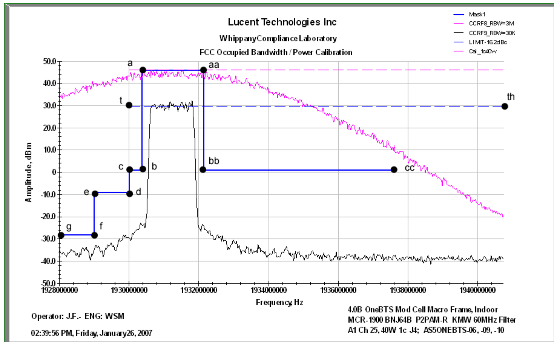
Figure 14B Occupied Bandwidth Mask for PCS Block Operation at 40 W with Power Calibration (PCS A Block is depicted with a single carrier signal showing use of the Power Calibration Trace )
