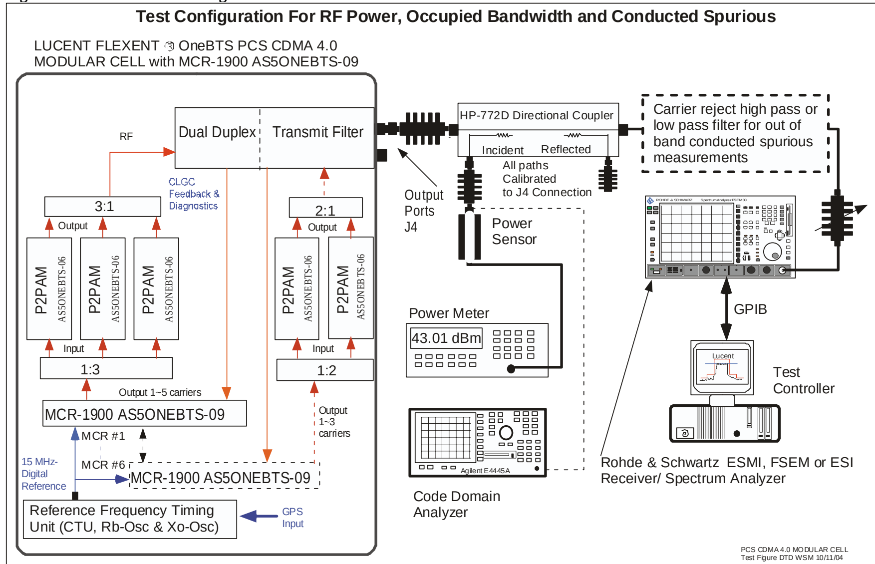
Figure 12 RF Power Test Configuration
