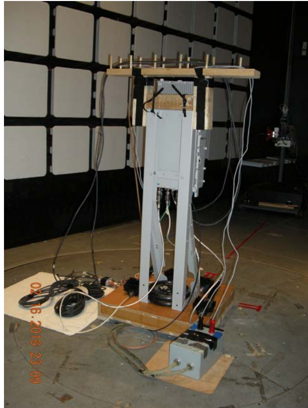
Rear
