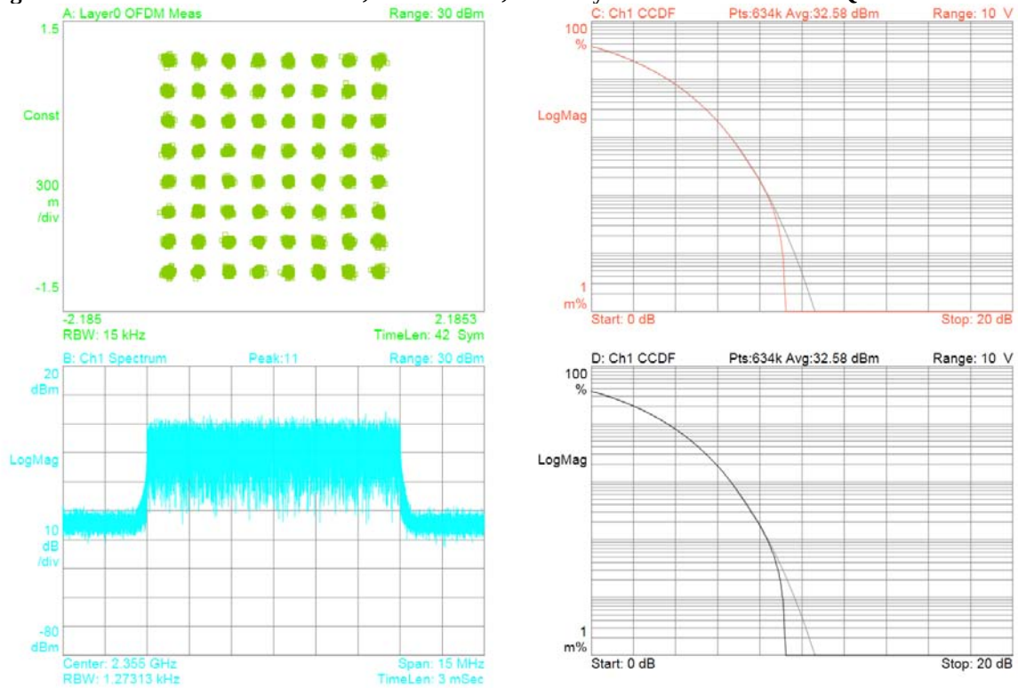
13.3. Figure 13A of Modulation AB Block, Channel 100, Primary Transmit Path Tx1 64QAM
