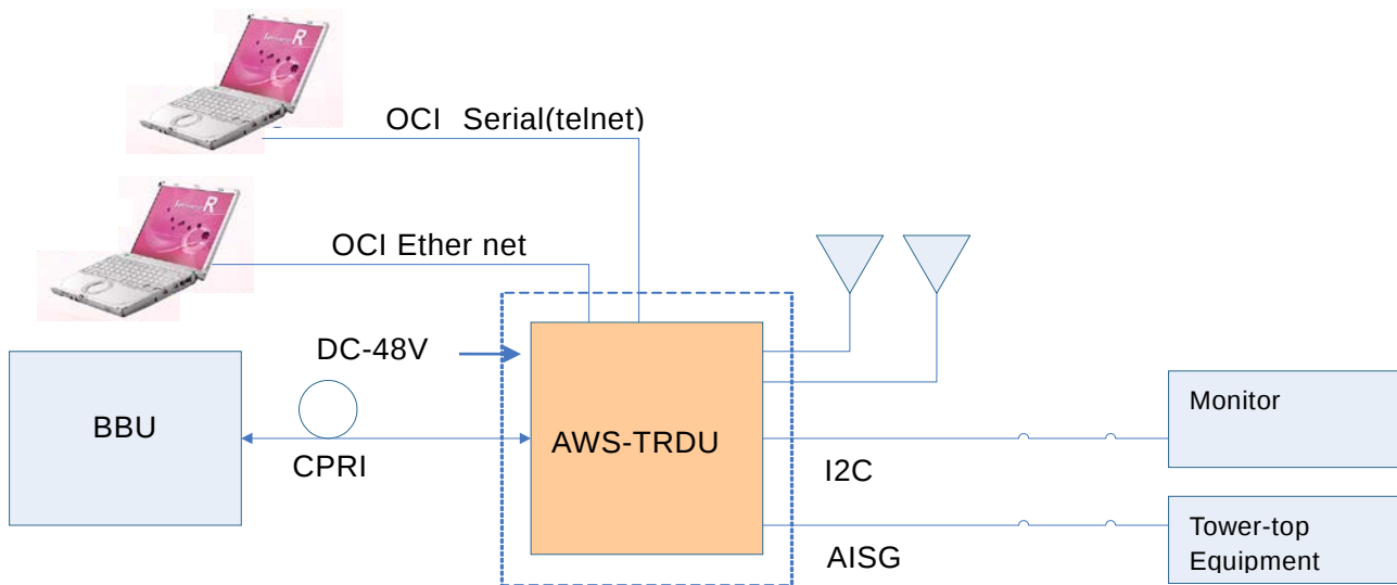
Figure 1-2 Equipment Outline
