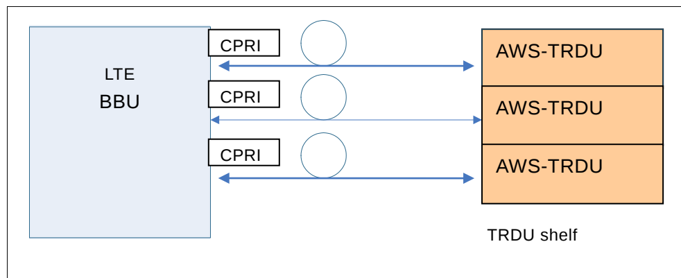
Figure 1-1 System Overview
