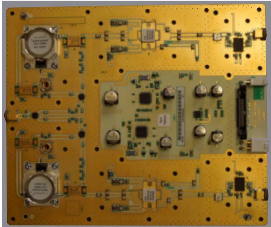
Front and Rear Views of PA Board with Shielding Cover Removed
