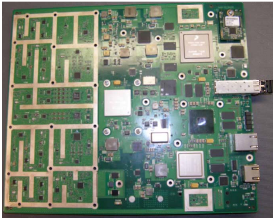
Front and Rear Views of D/A Board
