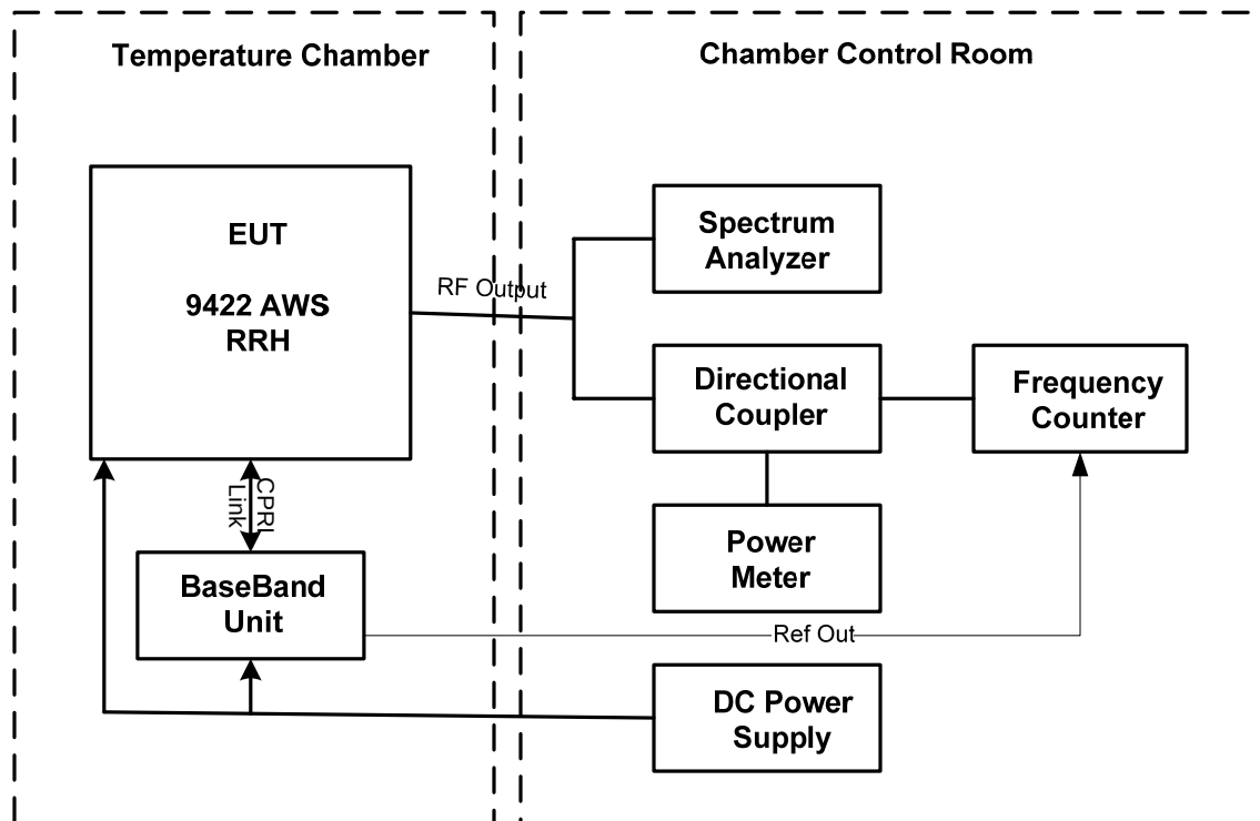
Frequency Stability Test Set-up Block Diagram 9442 AWS RRH
