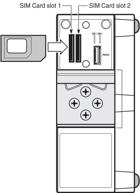
Figure 12 SIM slots and orientation on the 7705 SAR-Hm
