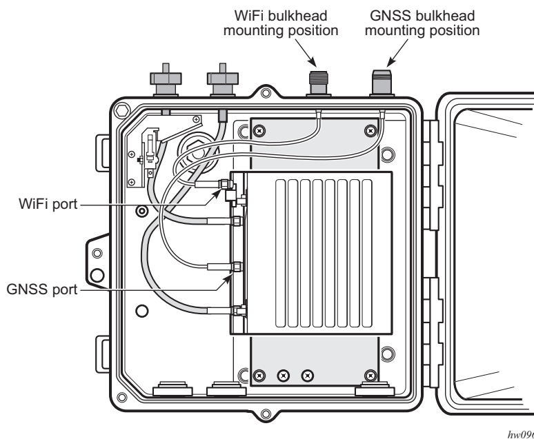
Figure 41 Connecting the WiFi and GNSS cables on the 7705 SAR-Hm
