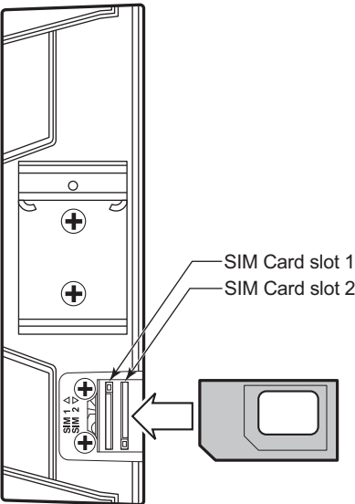
Figure 13 SIM slots and orientation on the 7705 SAR-Hmc
