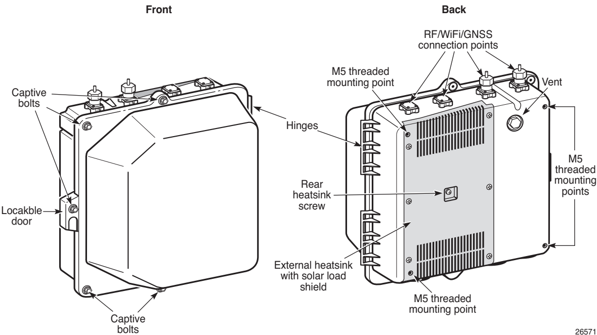
Figure 29 7705 Outdoor Enclosure front and back
