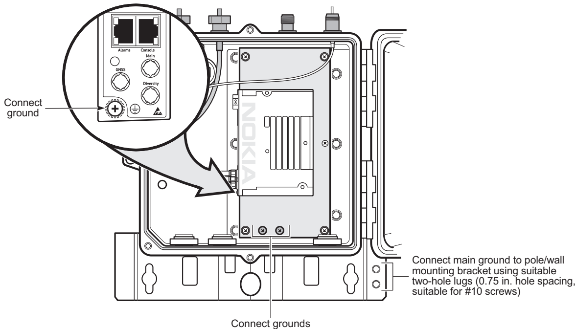
Figure 53 Performing the grounding on the 7705 SAR-Hmc
