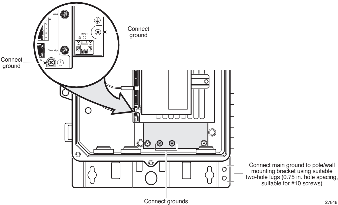
Figure 52 Performing the grounding on the 7705 SAR-Hm
