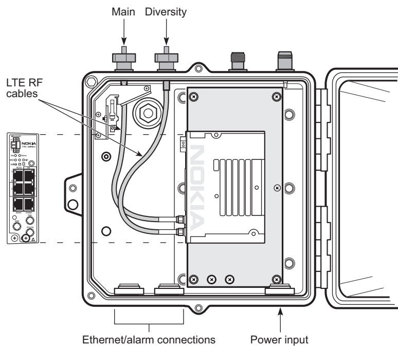
Figure 46 Connecting the LTE RF cables on the 7705 SAR-Hmc
