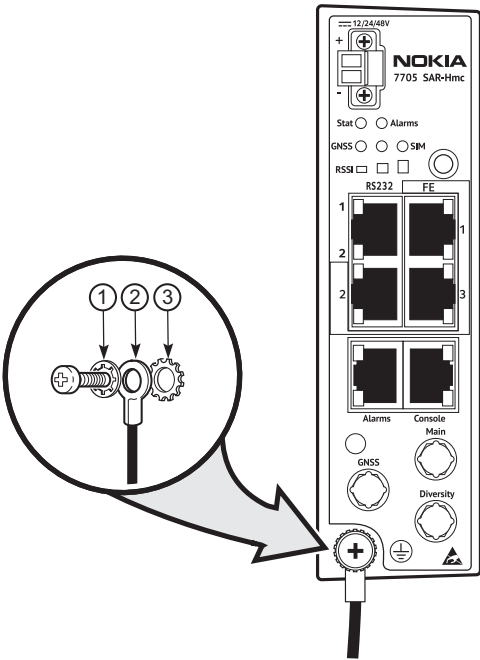
Figure 24 Attaching a ground connector on the 7705 SAR-Hmc
