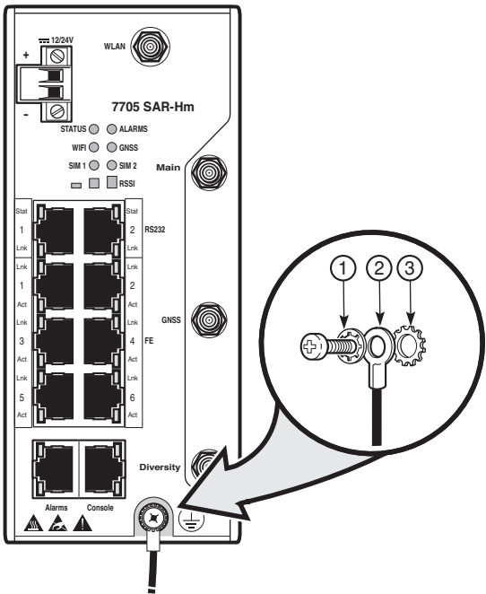
Figure 23 Attaching a ground connector on the 7705 SAR-Hm
