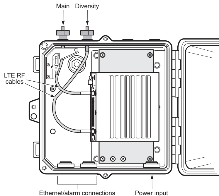
Figure 40 Connecting the LTE RF cables on the 7705 SAR-Hm
