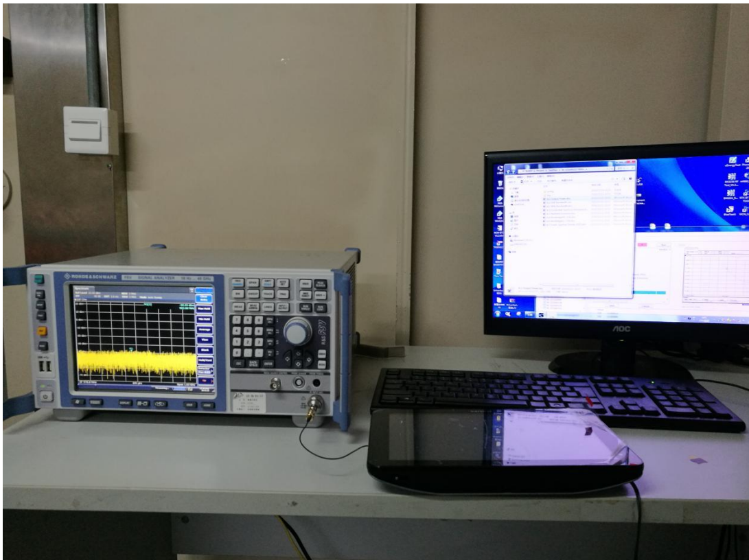
Conducted Test
