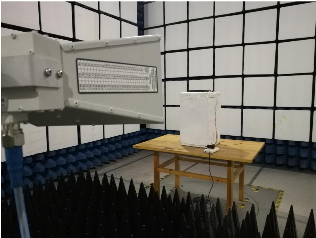
Above 1GHz
