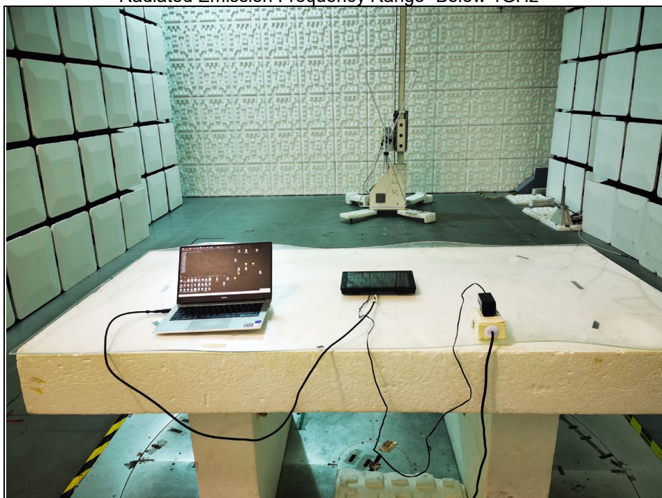
Radiated Emission Frequency Range <Below 1GHz >
