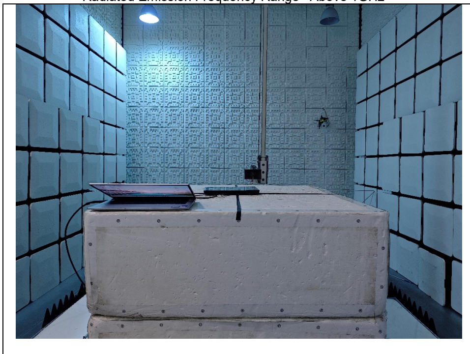
Radiated Emission Frequency Range < Above 1GHz >
