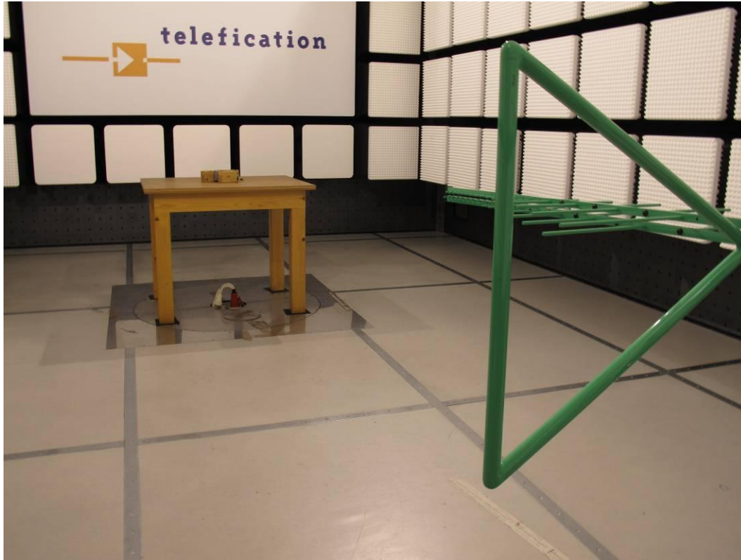
Photograph 1: Test setup radiated emissions (30 - 1000 MHz)
