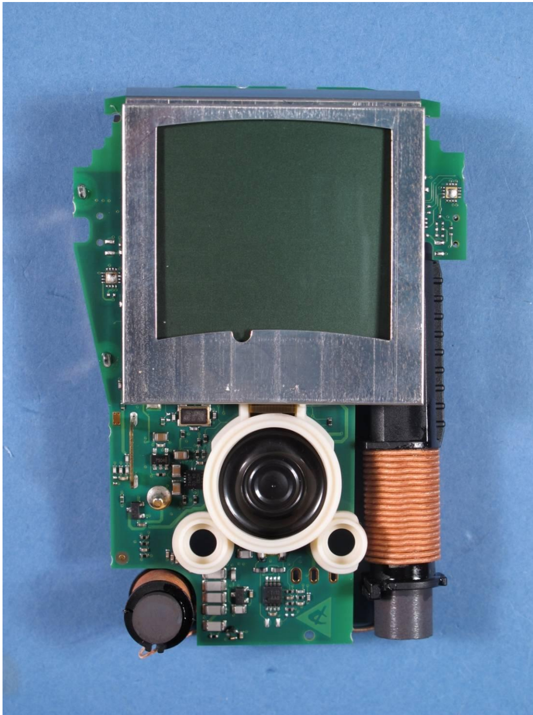
Photograph 3: - PCB of Element Barryvox, top view
