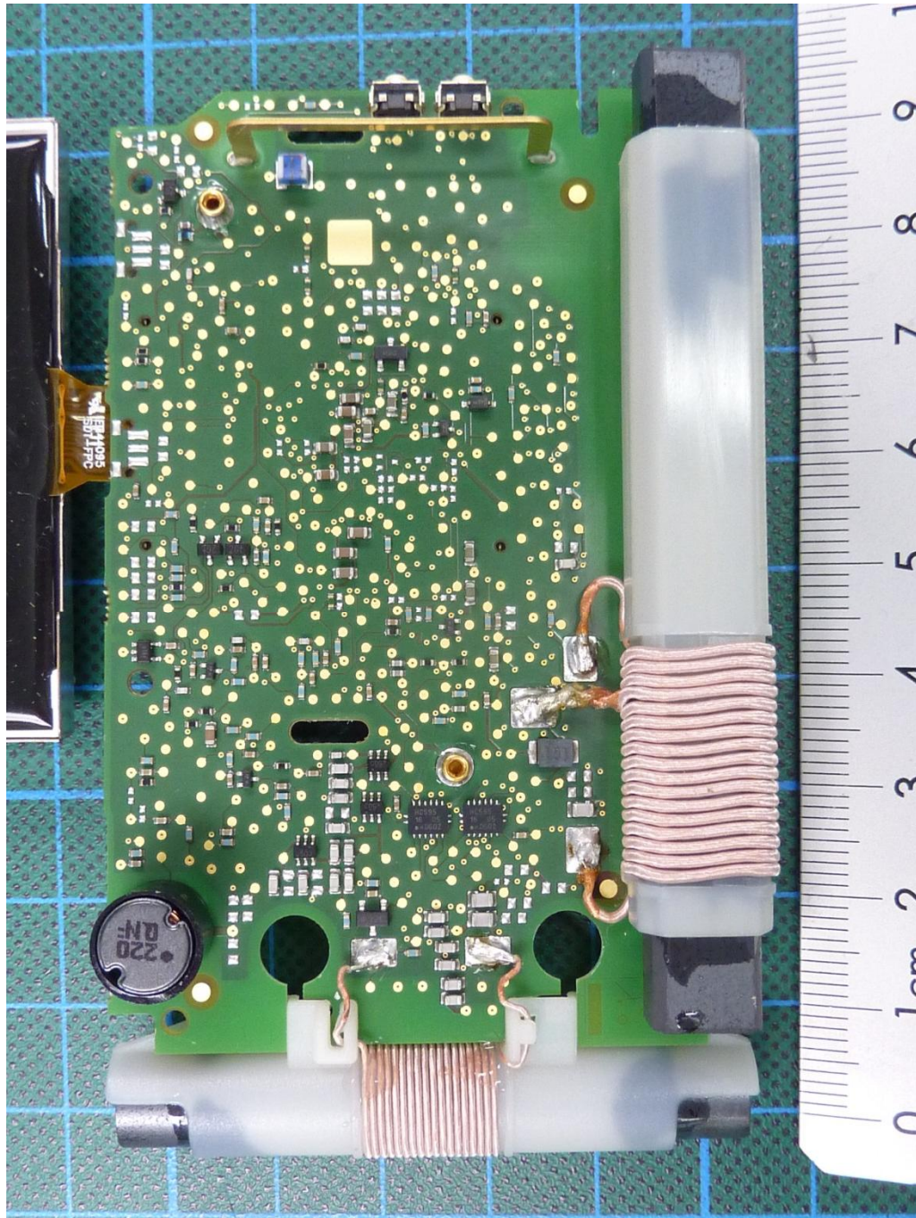
171626_24.JPG: Barryvox, PCB, bottom view
