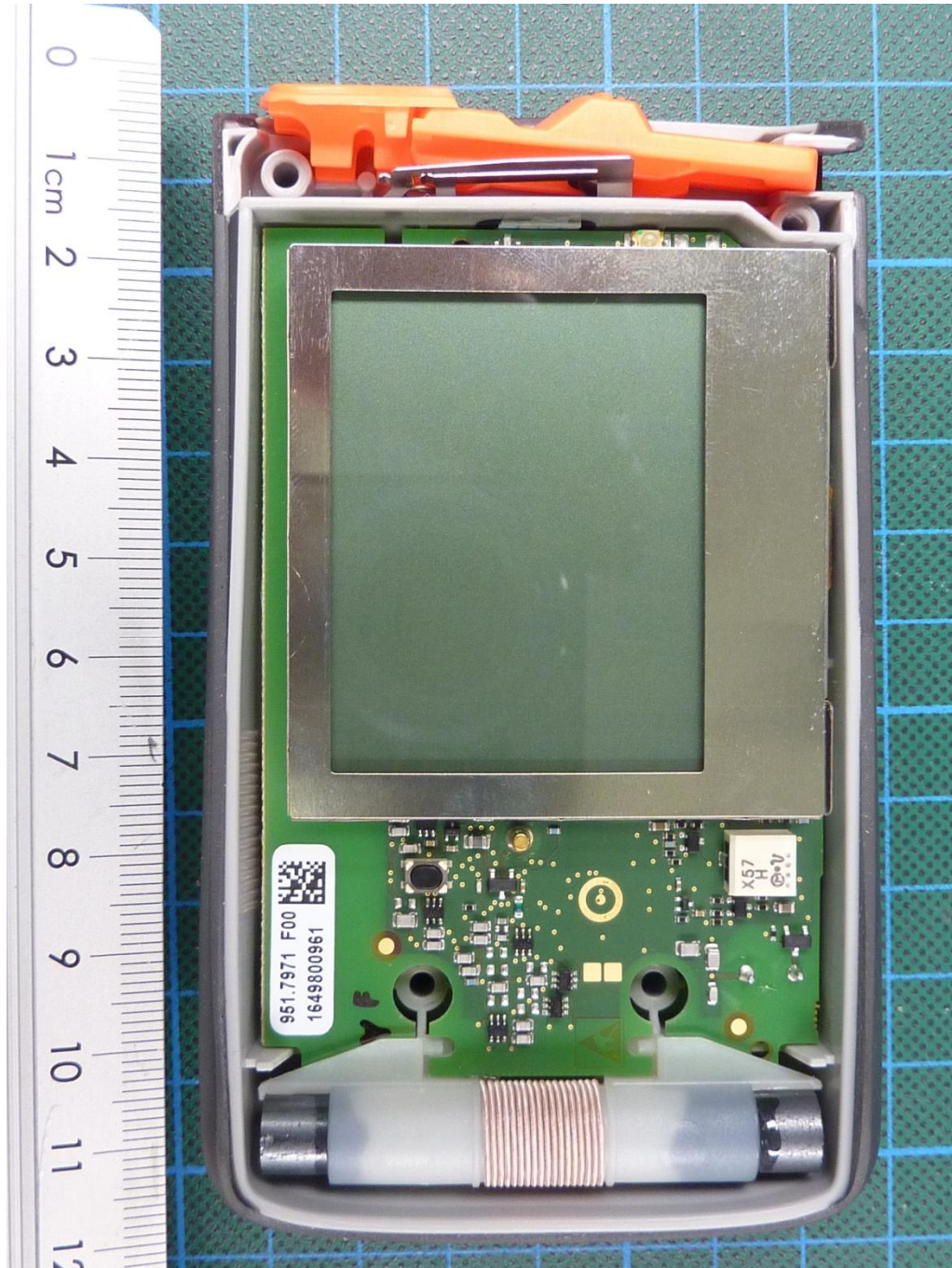
171626_19.JPG: Barryvox, internal view 2 (housing removed)
