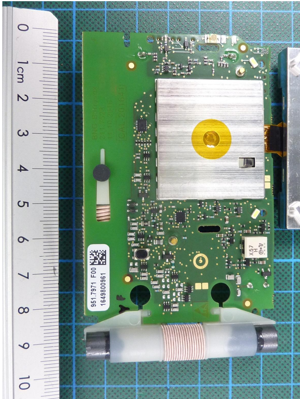
171626_22.JPG: Barryvox, PCB, top view
