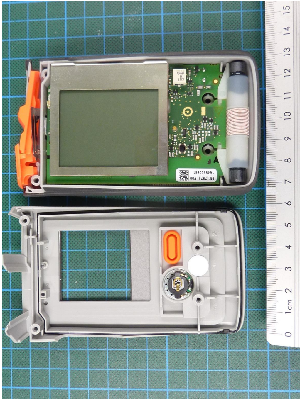
171626_18.JPG: Barryvox, internal view 1
