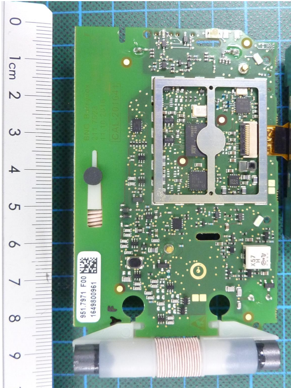
171626_23.JPG: Barryvox, PCB, top view, shielding removed
