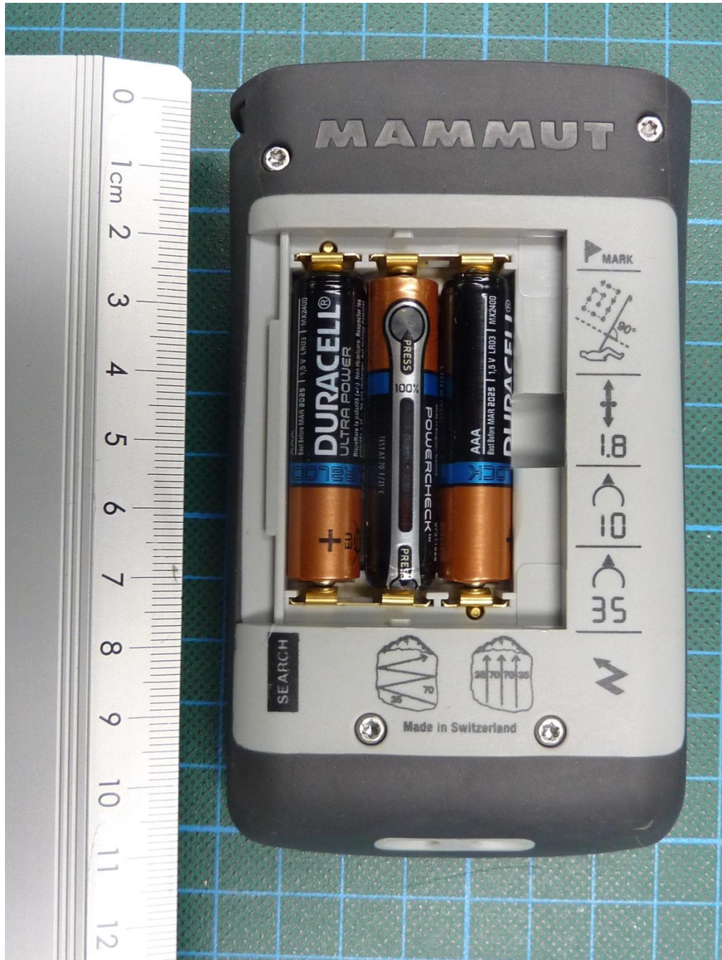
171626_15.JPG: Barryvox, rear view, battery cover removed
