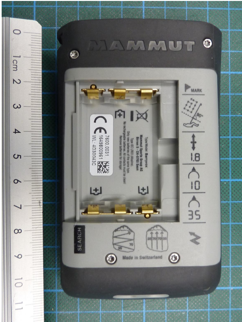
171626_16.JPG: Barryvox, rear view, batteries removed
