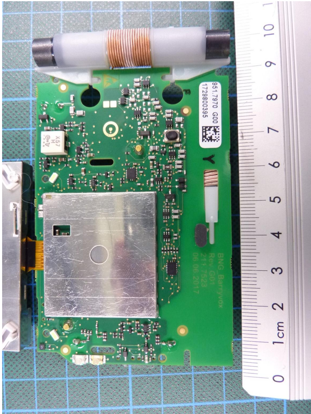
171626_9.JPG: Barryvox S, PCB, top view
