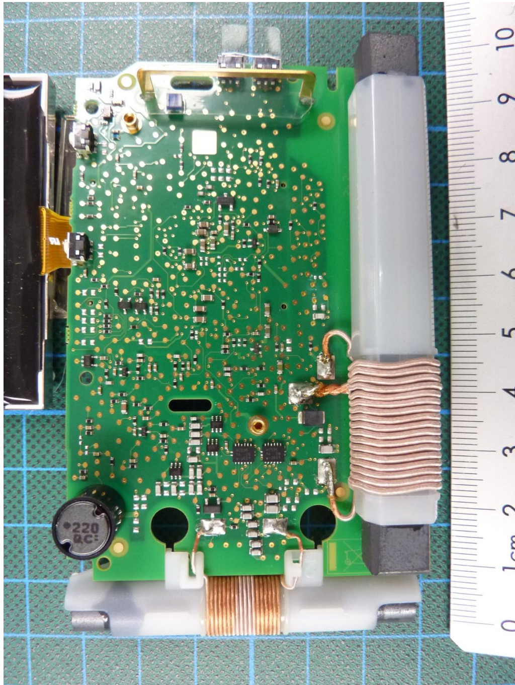
171626_11.JPG: Barryvox S, PCB, bottom view
