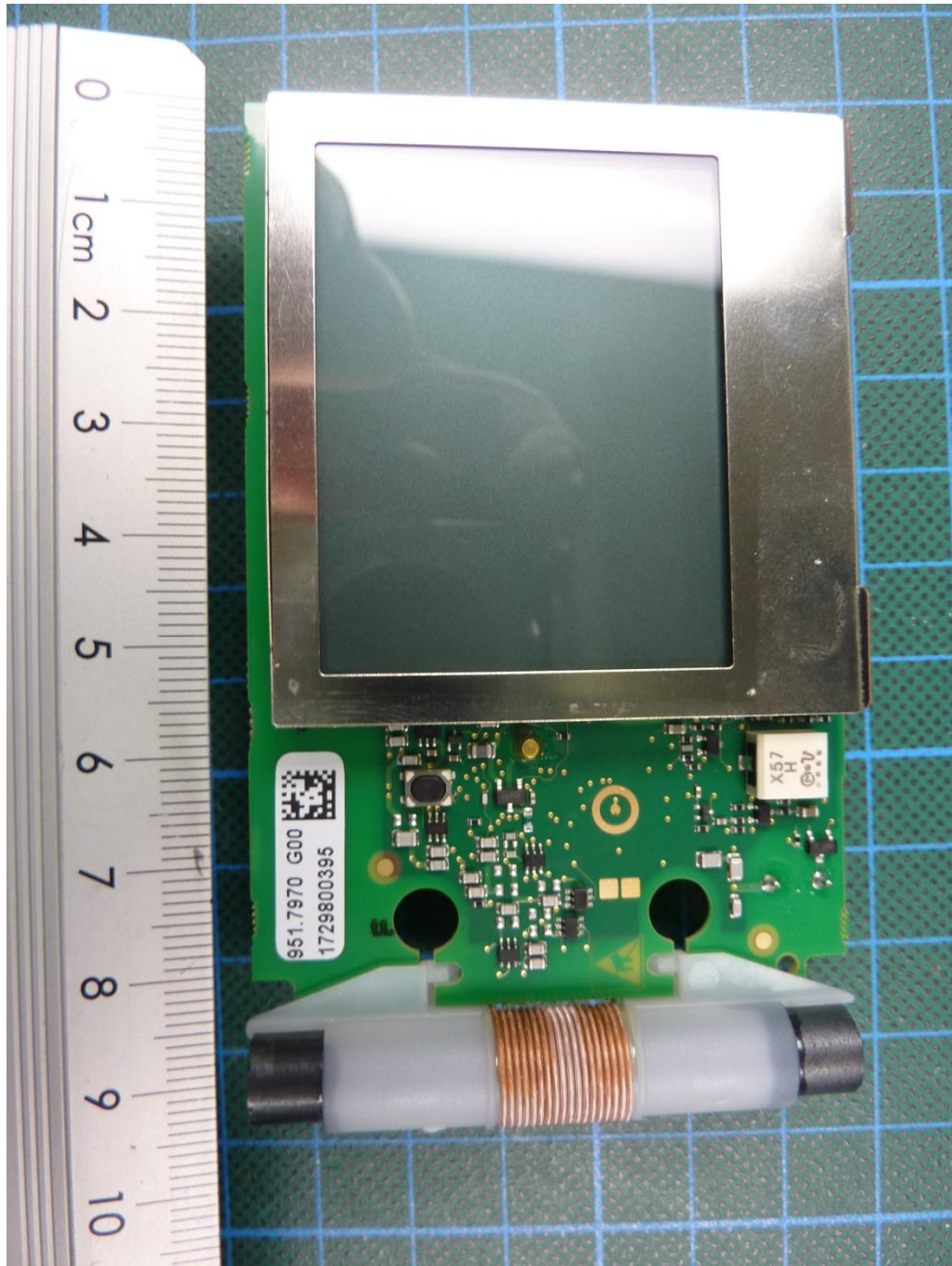
171626_7.JPG: Barryvox S, internal view 2 (housing removed)
