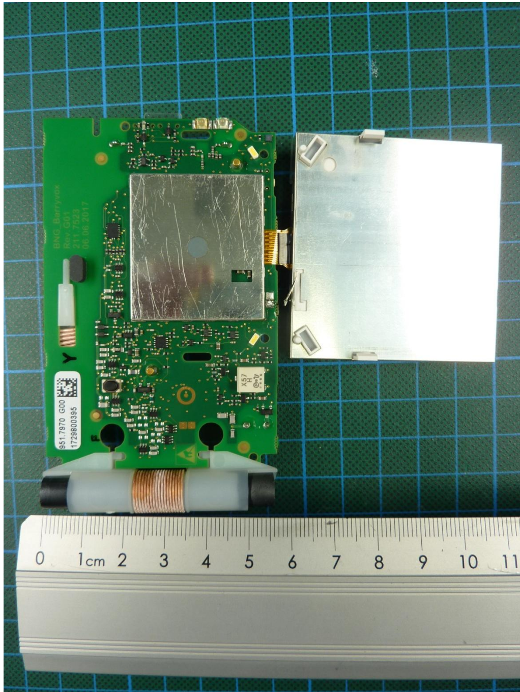
171626_8.JPG: Barryvox S, internal view 3 (display removed)
