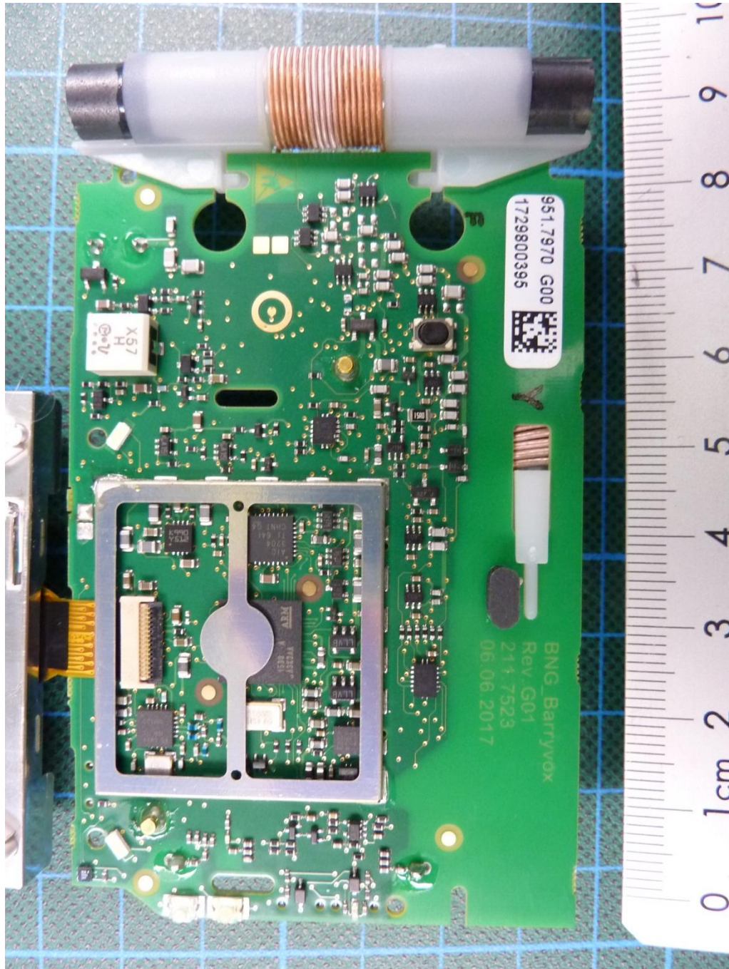
171626_10.JPG: Barryvox S, PCB, top view, shielding removed
