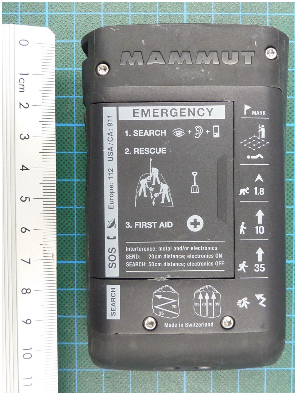
171626_3.JPG: Barryvox S, rear view
