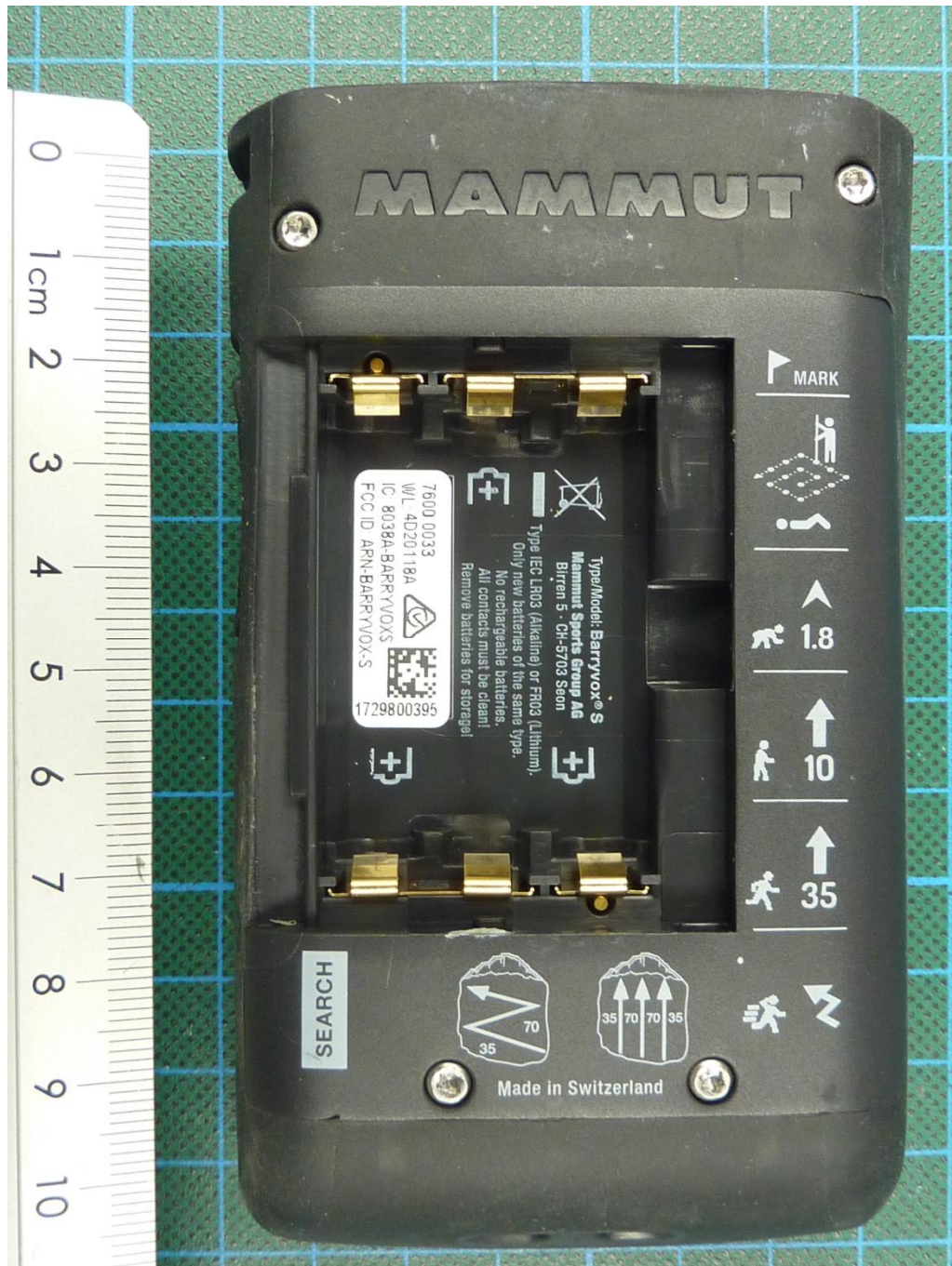
171626_5.JPG: Barryvox S, rear view, batteries removed
