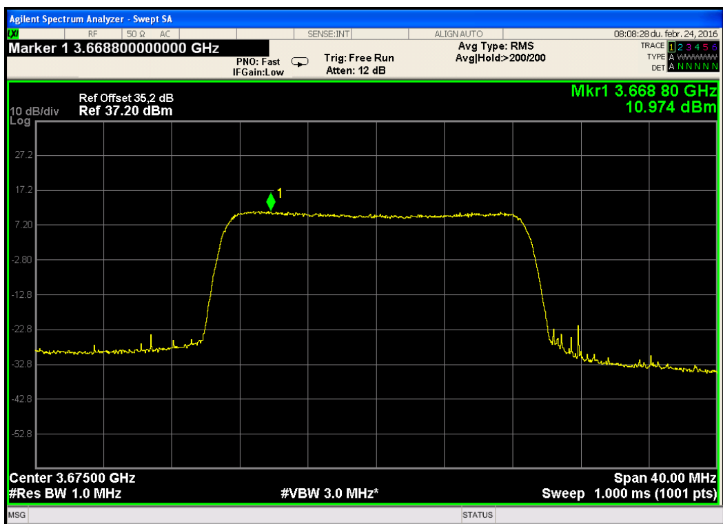
Figure 111. — 3675.0MHz 16QAM - 20MHz CBW, High Population
