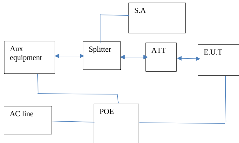
Figure 1. Conducted Emission From Antenna Ports Test Set-up
