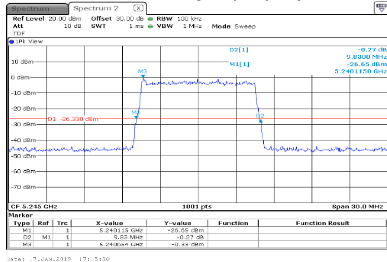
Plot 7.2.9 The 26 dB bandwidth test result at high frequency, 64QAM modulation, 10 MHz EBW
