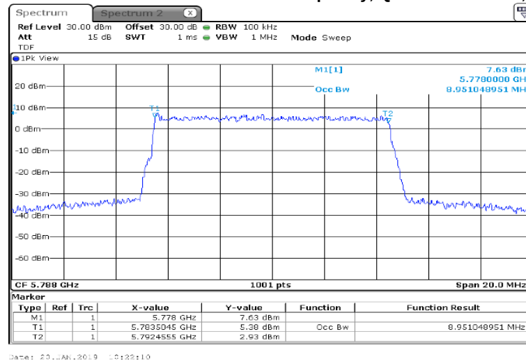
Plot 7.2.4 The 99% bandwidth test result at mid frequency, QPSK modulation, 10 MHz EBW
