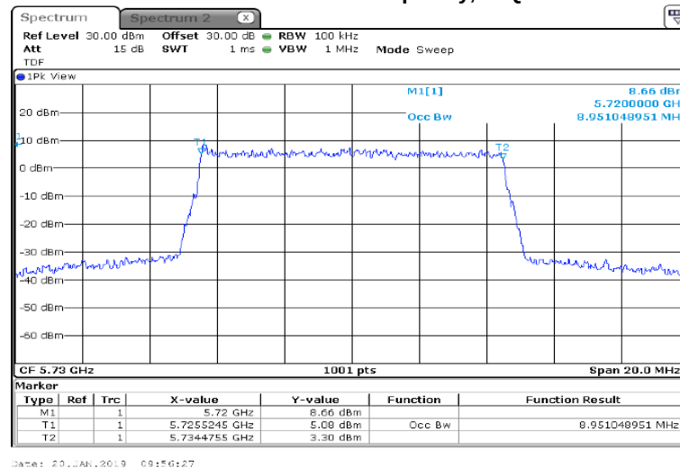
Plot 7.2.2 The 99% bandwidth test result at low frequency, 16QAM modulation, 10 MHz EBW
