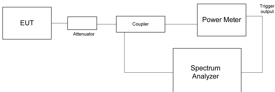
Figure 7.3.1 Occupied bandwidth test setup
