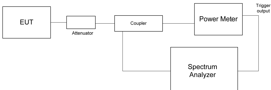
Figure 7.4.1 Emission mask test setup
