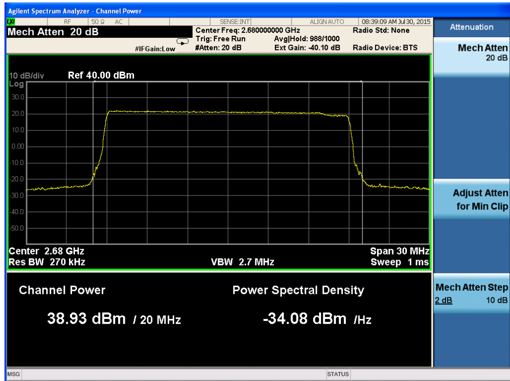
Figure 75. — 2680.0 MHz 16QAM Port 1
