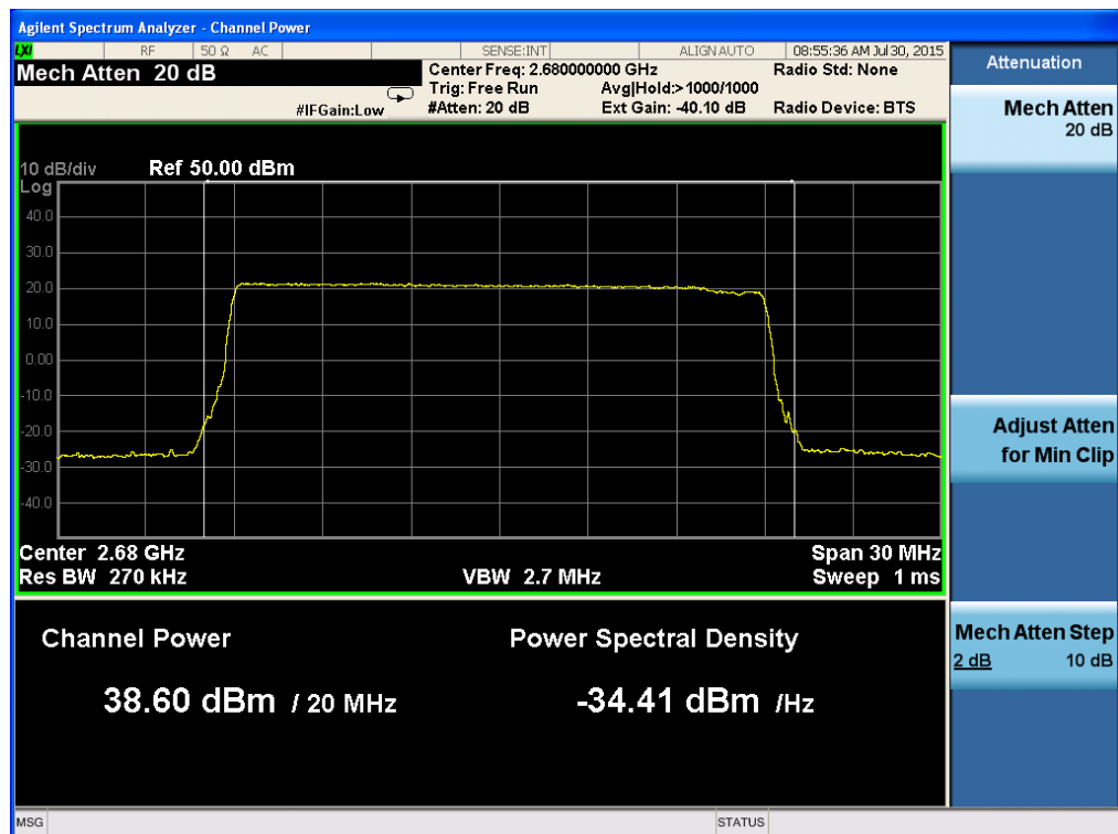
Figure 76. — 2680.0 MHz 16QAM Port 2
