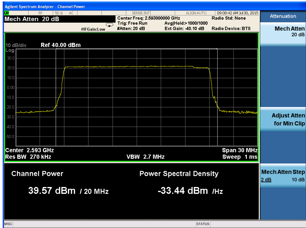
Figure 65. — 2593.0 MHz 16QAM Port 3
