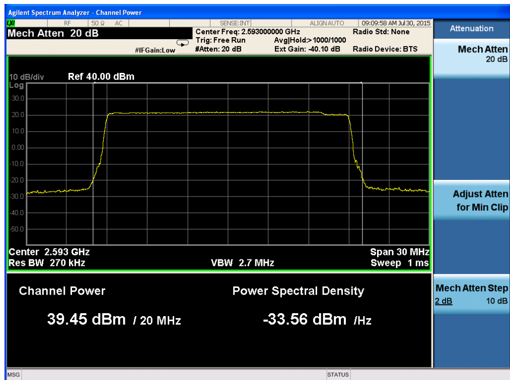
Figure 66. — 2593.0 MHz 16QAM Port 4
