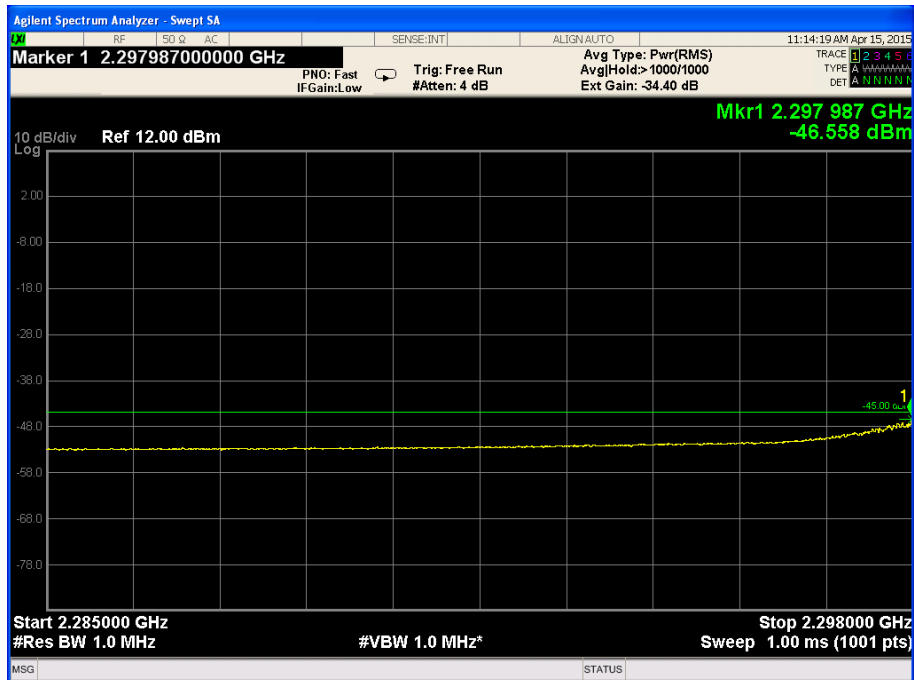
Figure 66. — 2285.0 MHz-2298.0 MHz
