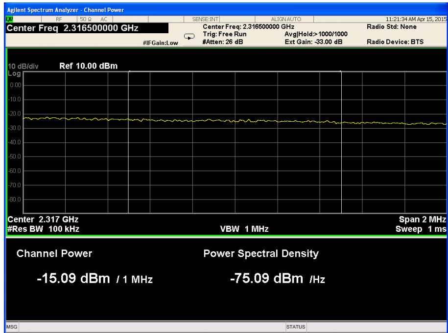
Figure 71. — 2316.0 MHz-2317.0 MHz
