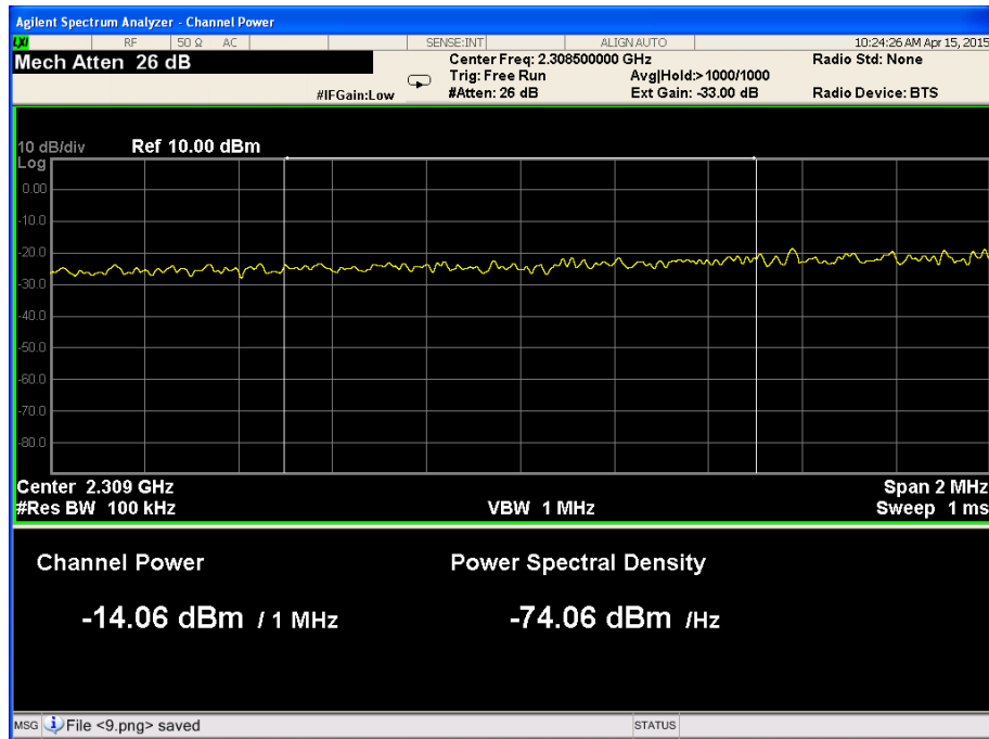
Figure 49. — 2308.0 MHz-2309.0 MHz
