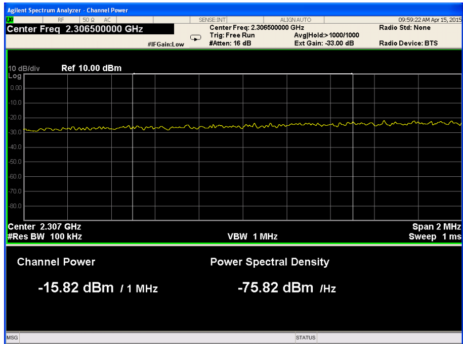
Figure 47. — 2306.0 MHz-2307.0 MHz
