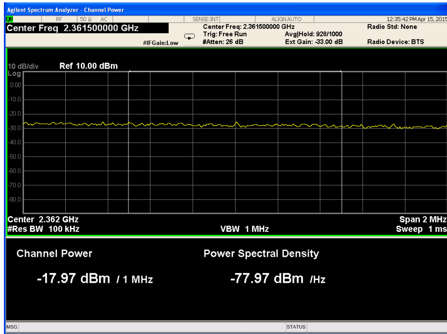
Figure 81. — 2361.0 MHz-2362.0 MHz
