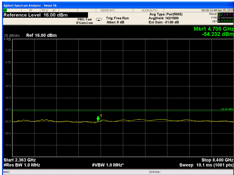
Figure 39. — 2362.5.0 MHz-8400.0 MHz
