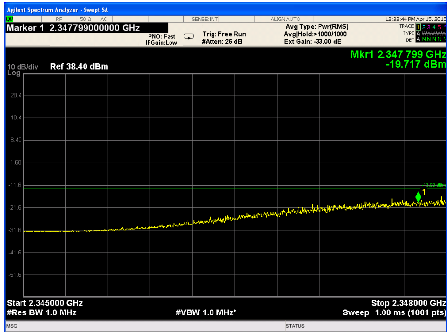
Figure 79. — 2345.0 MHz-2348.0 MHz
