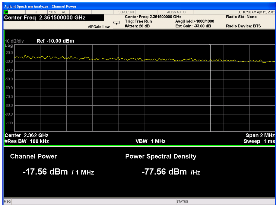
Figure 26. — 2361.0MHz-2362.0 MHz
