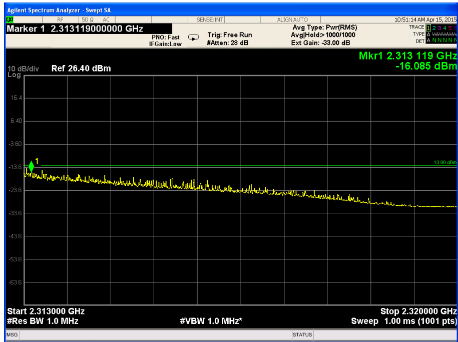
Figure 62. — 2313.0 MHz-2320.0 MHz
