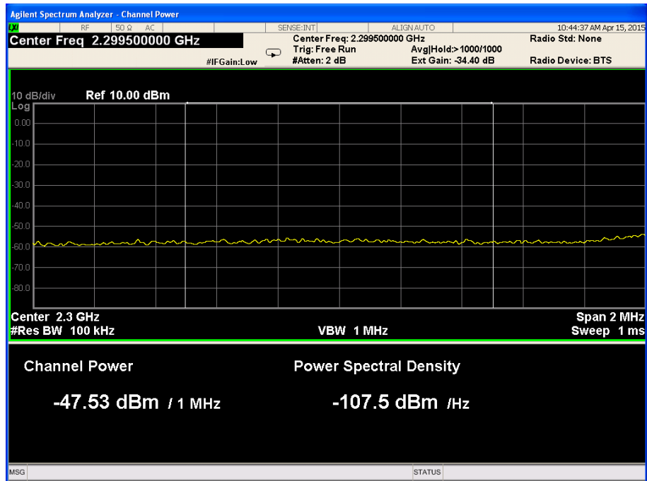
Figure 56. — 2299.0 MHz-2300.0 MHz
