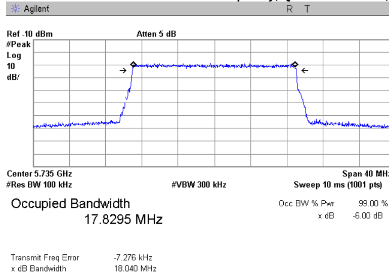
Plot 7.1.19 The 6 dB bandwidth test result at low frequency, QPSK modulation, 20 MHz EBW
