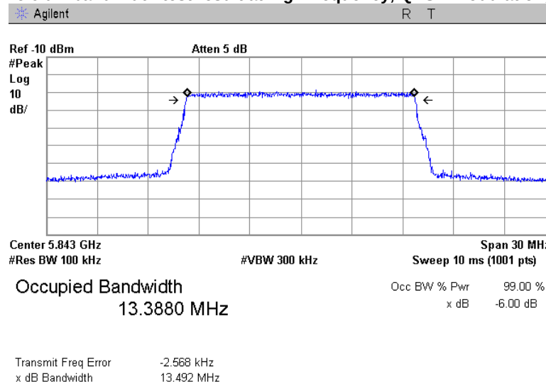
Plot 7.1.16 The 6 dB bandwidth test result at high frequency, QPSK modulation, 15 MHz EBW
