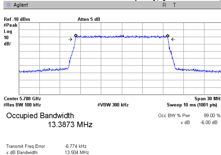
Plot 7.1.13 The 6 dB bandwidth test result at mid frequency, QPSK modulation, 15 MHz EBW
