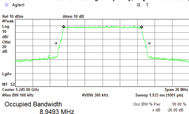
Plot 7.2.8 The 26 dB bandwidth test result at high frequency, 16QAM modulation, 10 MHz EBW
