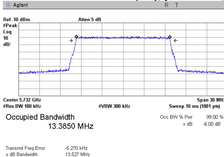
Plot 7.1.10 The 6 dB bandwidth test result at low frequency, QPSK modulation, 15 MHz EBW
