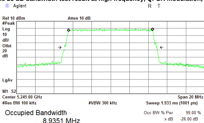
Plot 7.2.7 The 26 dB bandwidth test result at high frequency, QPSK modulation, 10 MHz EBW
