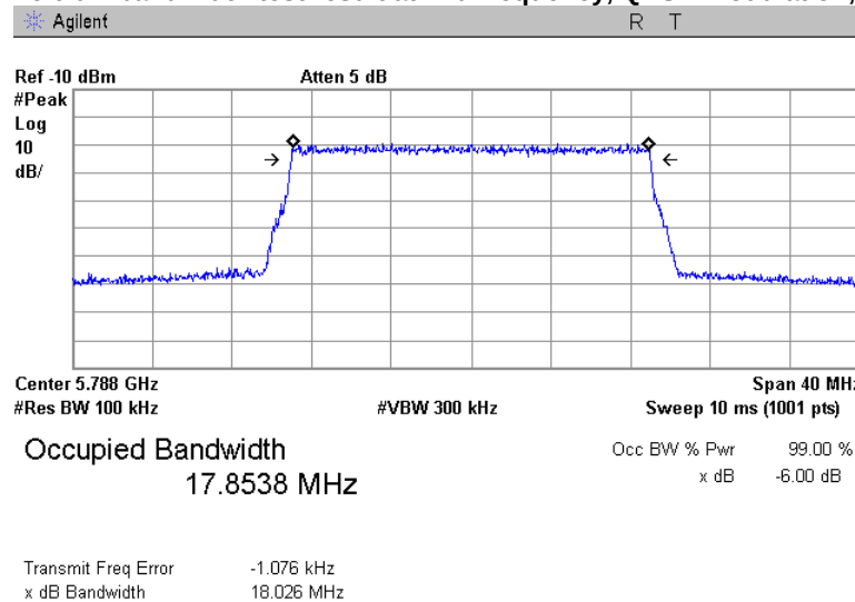
Plot 7.1.22 The 6 dB bandwidth test result at mid frequency, QPSK modulation, 20 MHz EBW
