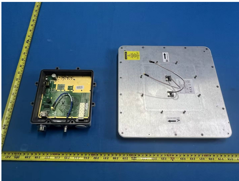
With Antenna Configuration 2
