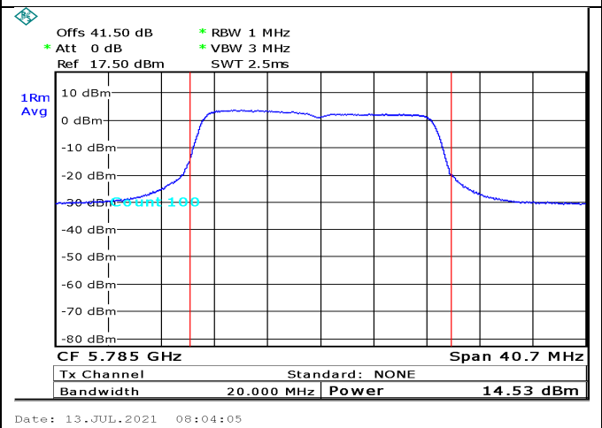
Figure 173. 5785.0MHz,20MHz BW, port2
