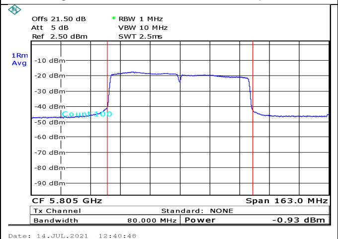
Figure 97. 5805.0MHz,80MHz BW, port2
