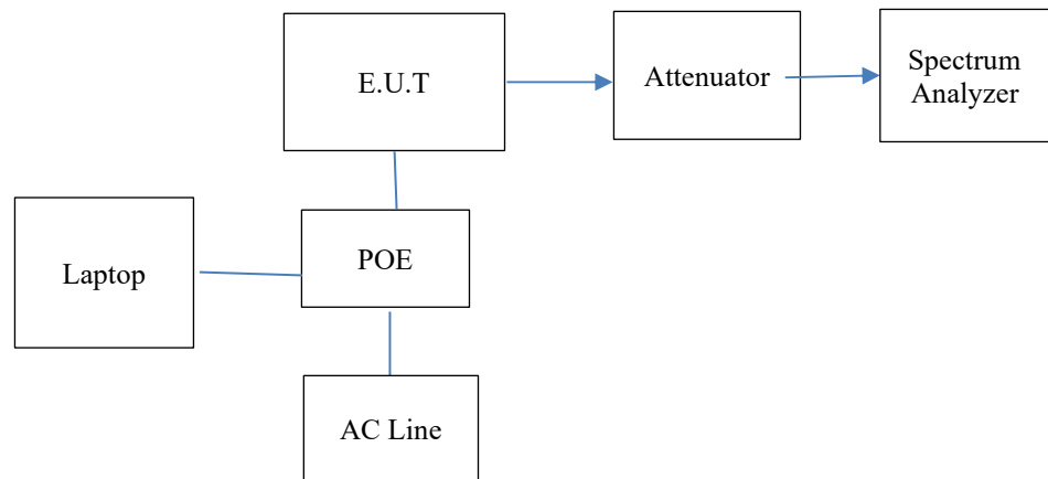
Figure 1. Configuration of Tested System - Conducted
