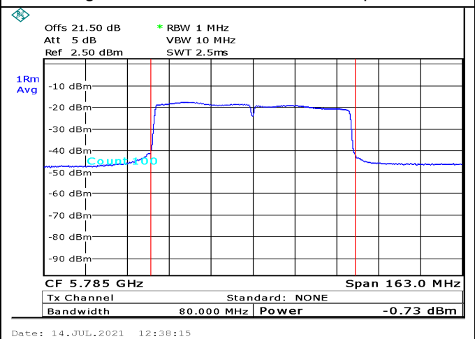
Figure 95. 5785.0MHz,80MHz BW, port2
