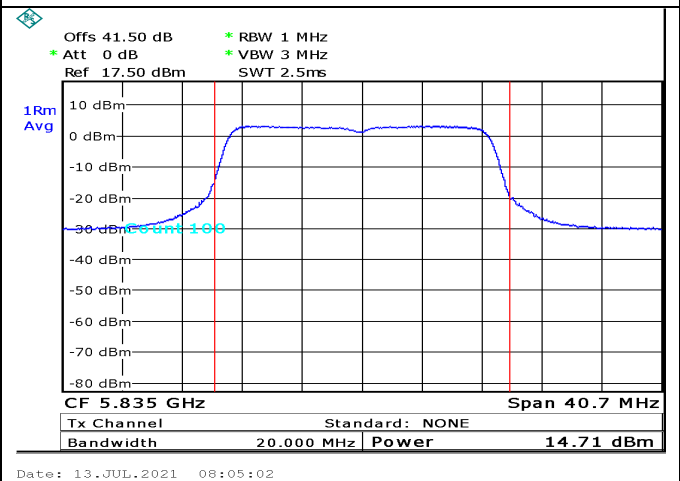
Figure 175. 5835.0MHz,20MHz BW, port2
