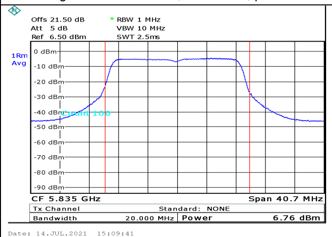
Figure 67. 5835.0MHz,20MHz BW, port2
