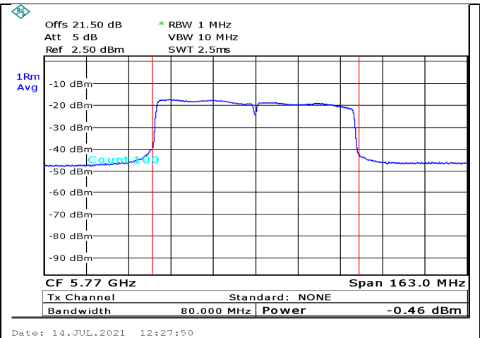
Figure 93. 5770.0MHz,80MHz BW, port2
