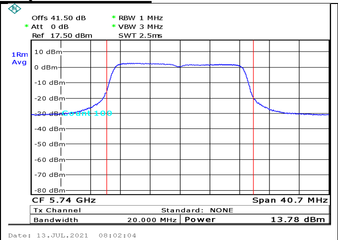
Figure 171. 5740.0MHz,20MHz BW, port2
