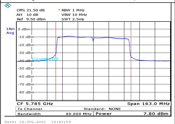
Figure 41. 5785.0MHz,80MHz BW, port2
