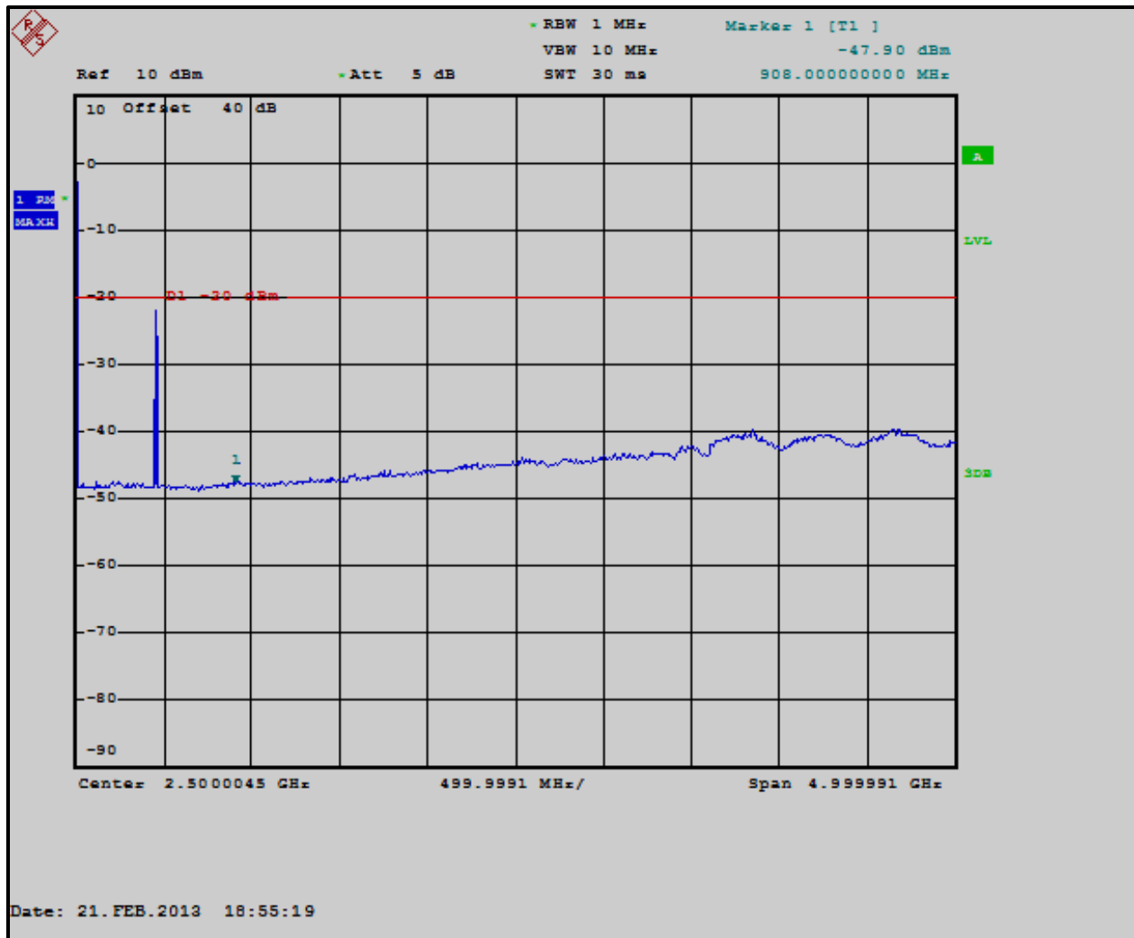
Plot 5-11: Conducted Spurious Emissions – H-CPM TDMA; 454.0000 MHz
