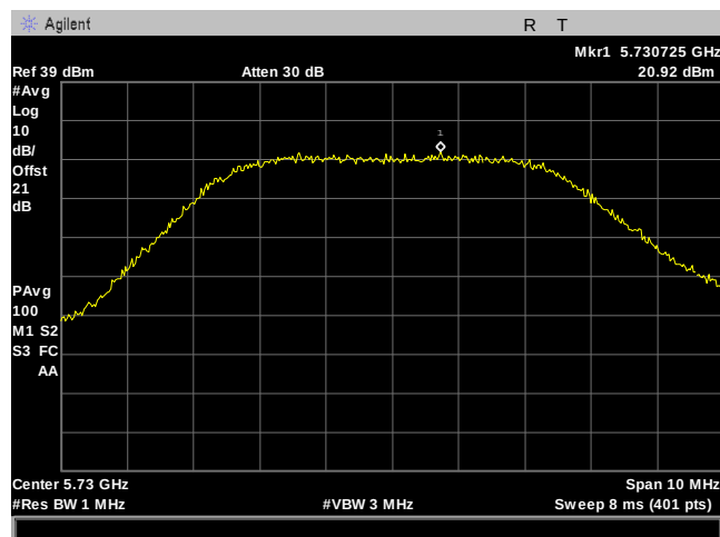
Plot 110. Power Spectral Density, 5M, 5730MHz, 8Omni, Port 2
