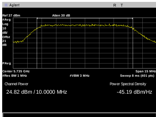
Plot 67. Maximum Conducted Output Power, 10M, 5735, 2Panel, Port 1
