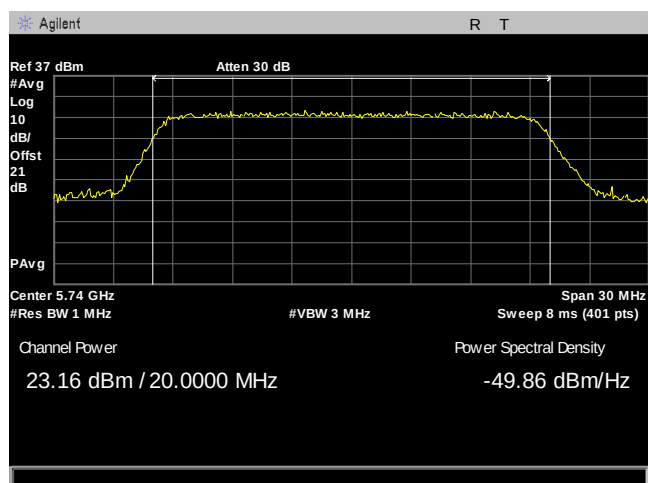
Plot 26. Maximum Conducted Output Power, 20M, 5740, 8Omni, Port 2
