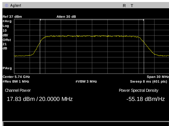
Plot 49. Maximum Conducted Output Power, 20M, 5740, 90Sector, Port 1
