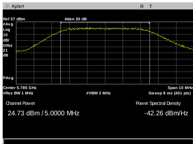
Plot 88. Maximum Conducted Output Power, 5M, 5785, 3Para, Port 2
