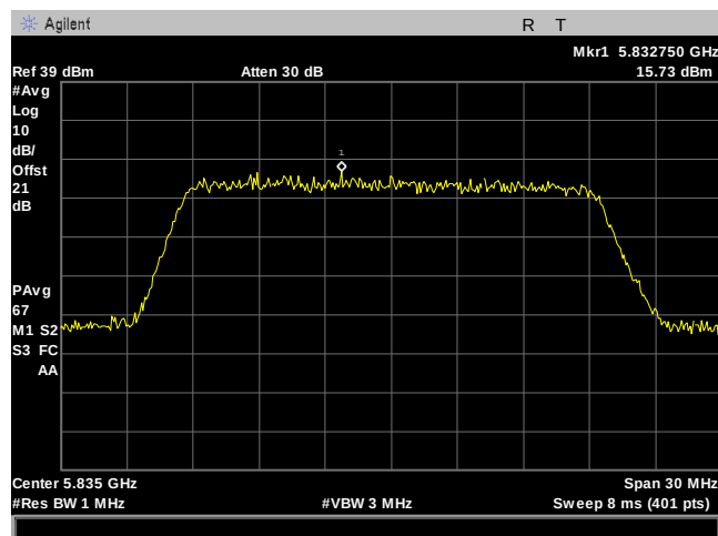
Plot 173. Power Spectral Density, 20M, 5835MHz, 2Panel, Port 1
