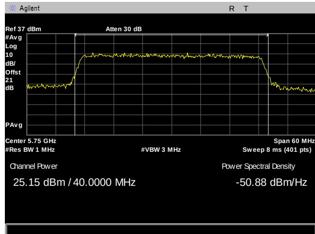
Plot 103. Maximum Conducted Output Power, 40M, 5750, 3Para, Port 1
