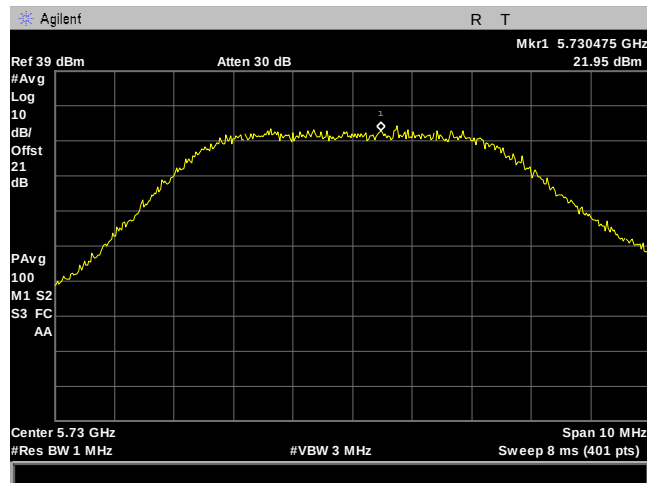
Plot 157. Power Spectral Density, 5M, 5730MHz, 2Panel, Port 1
