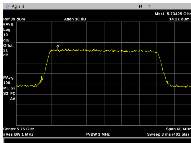
Plot 200. Power Spectral Density, 40M, 5750MHz, 2Para, Port 2
