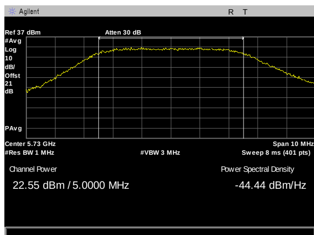
Plot 14. Maximum Conducted Output Power, 5M, 5730, 8Omni, Port 2
