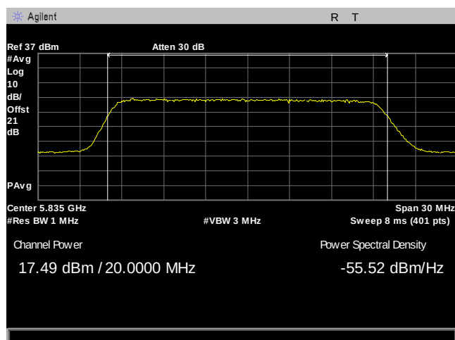
Plot 53. Maximum Conducted Output Power, 20M, 5835, 90Sector, Port 1
