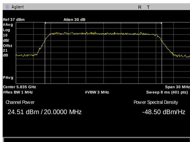
Plot 77. Maximum Conducted Output Power, 20M, 5835, 2Panel, Port 1
