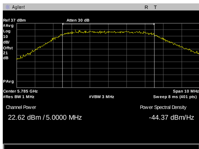
Plot 15. Maximum Conducted Output Power, 5M, 5785, 8Omni, Port 1
