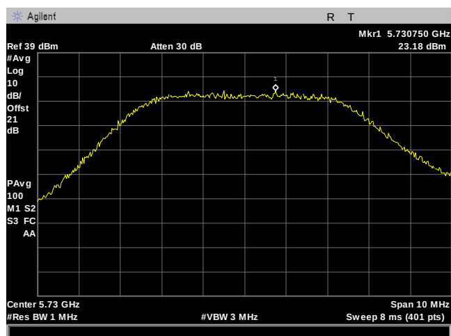
Plot 182. Power Spectral Density, 5M, 5730MHz, 2Para, Port 2
