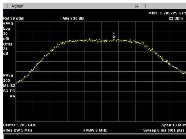
Plot 159. Power Spectral Density, 5M, 5785MHz, 2Panel, Port 1
