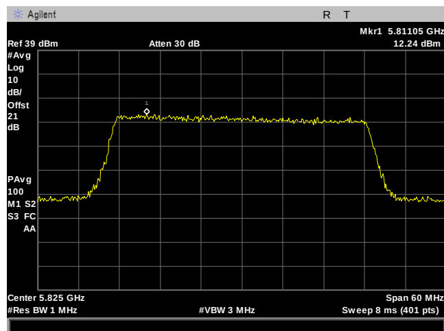
Plot 180. Power Spectral Density, 40M, 5825MHz, 2Panel, Port 2
