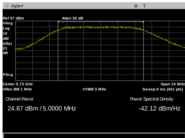
Plot 61. Maximum Conducted Output Power, 5M, 5730, 2Panel, Port 1
