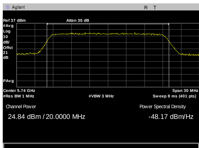
Plot 98. Maximum Conducted Output Power, 20M, 5740, 3Para, Port 2
