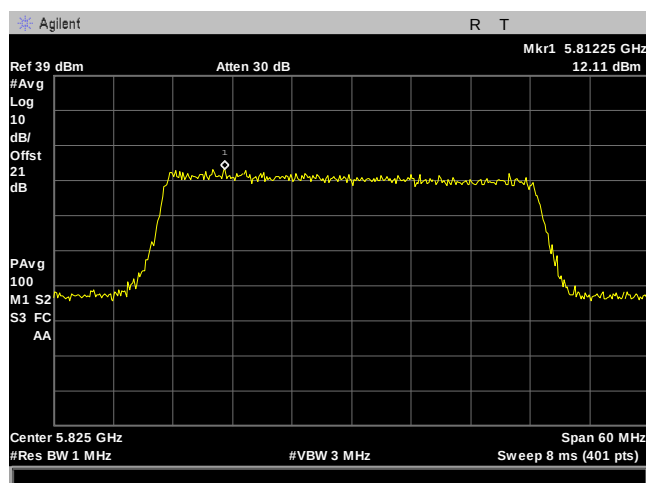
Plot 203. Power Spectral Density, 40M, 5825MHz, 2Para, Port 1
