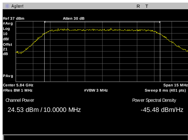
Plot 72. Maximum Conducted Output Power, 10M, 5840, 2Panel, Port 2
