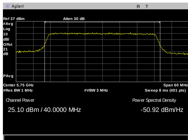
Plot 80. Maximum Conducted Output Power, 40M, 5750, 2Panel, Port 2
