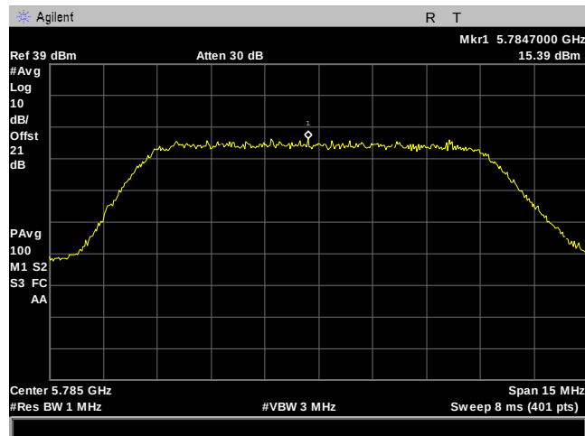
Plot 142. Power Spectral Density, 10M, 5785MHz, 90Sector, Port 2
