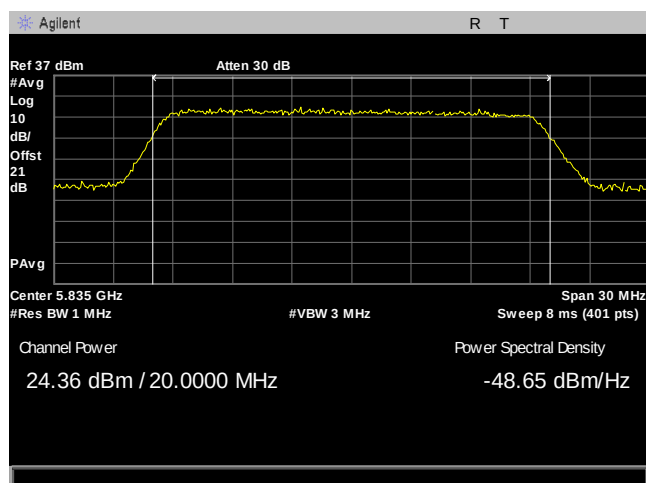
Plot 78. Maximum Conducted Output Power, 20M, 5835, 2Panel, Port 2
