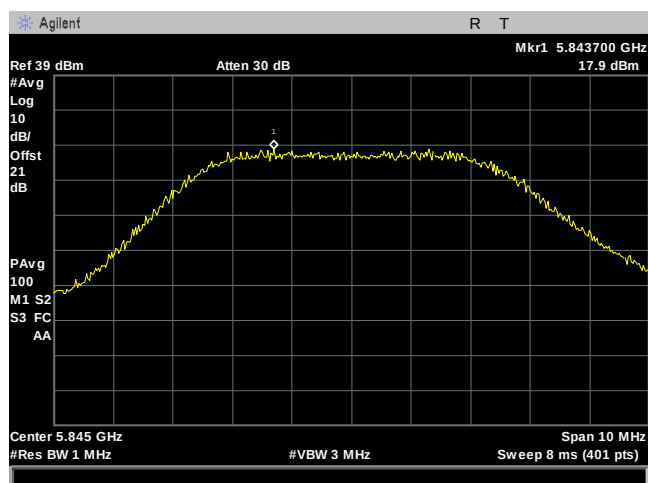
Plot 138. Power Spectral Density, 5M, 5845MHz, 90Sector, Port 2
