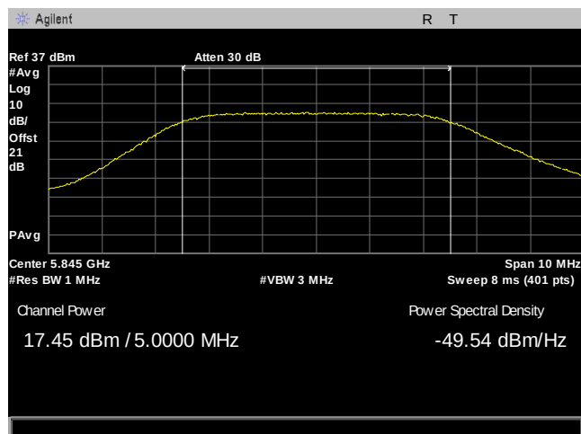
Plot 42. Maximum Conducted Output Power, 5M, 5845, 90Sector, Port 2
