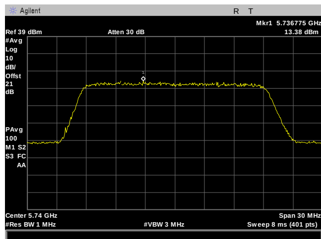
Plot 146. Power Spectral Density, 20M, 5740MHz, 90Sector, Port 2
