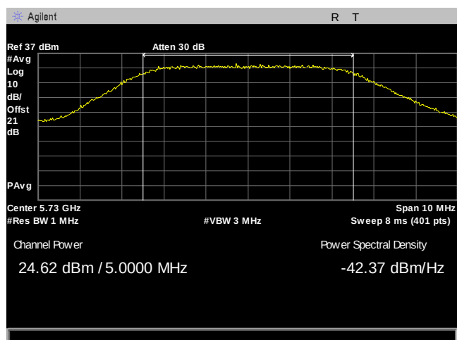
Plot 86. Maximum Conducted Output Power, 5M, 5730, 3Para, Port 2
