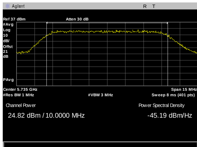
Plot 91. Maximum Conducted Output Power, 10M, 5735, 3Para, Port 1
