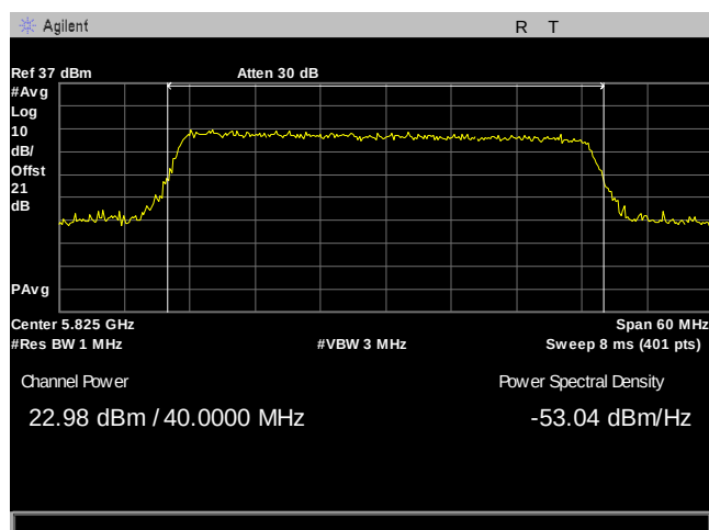
Plot 35. Maximum Conducted Output Power, 40M, 5825, 8Omni, Port 1
