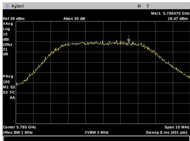
Plot 112. Power Spectral Density, 5M, 5785MHz, 8Omni, Port 2
