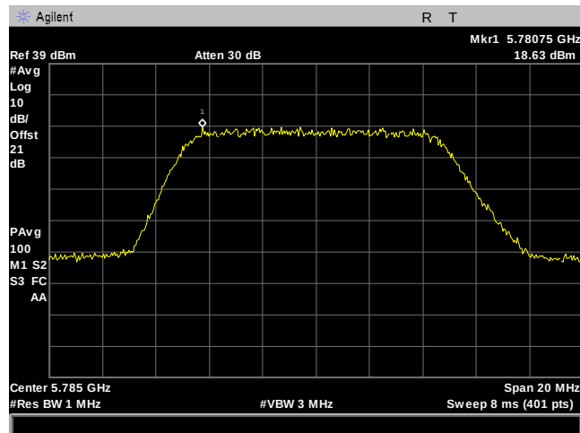
Plot 166. Power Spectral Density, 10M, 5785MHz, 2Panel, Port 2
