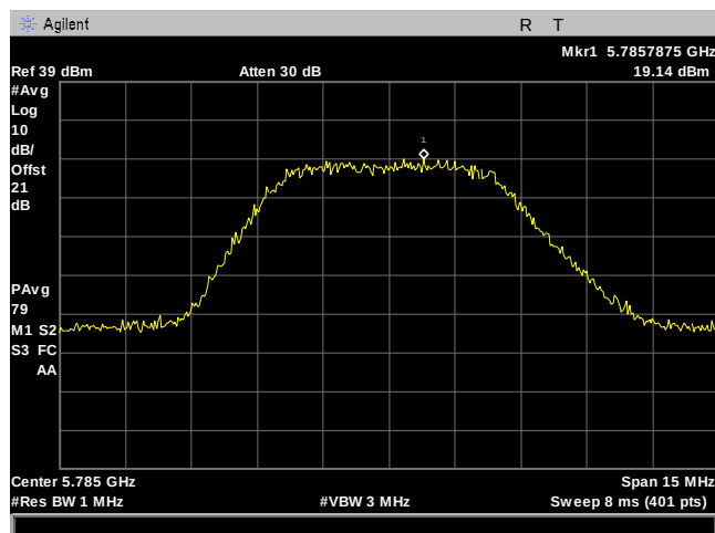
Plot 117. Power Spectral Density, 10M, 5785MHz, 8Omni, Port 1
