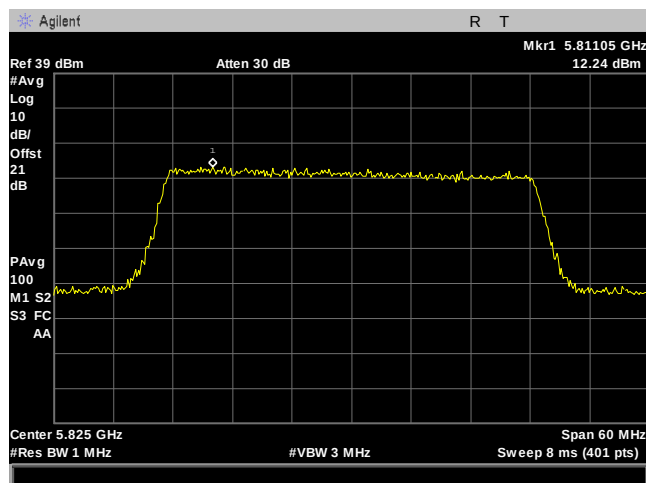
Plot 204. Power Spectral Density, 40M, 5825MHz, 2Para, Port 2
