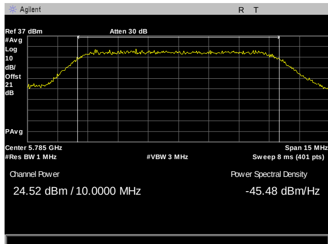
Plot 93. Maximum Conducted Output Power, 10M, 5785, 3Para, Port 1
