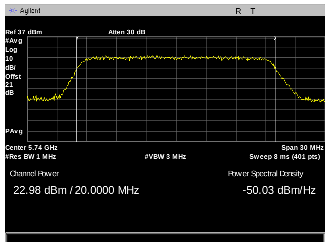
Plot 25. Maximum Conducted Output Power, 20M, 5740, 8Omni, Port 1
