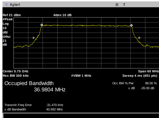
Plot 10. 26 dB Occupied Bandwidth, BW 40MHz, 5750MHz
