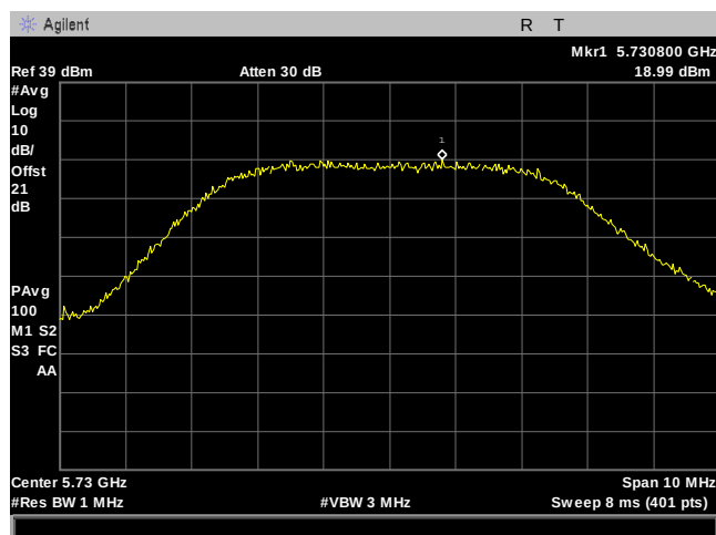
Plot 134. Power Spectral Density, 5M, 5730MHz, 90Sector, Port 2
