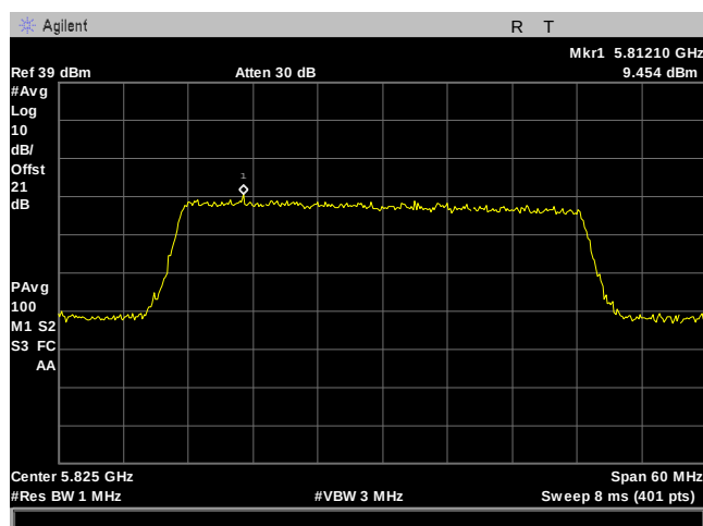
Plot 155. Power Spectral Density, 40M, 5825MHz, 90Sector, Port 1
