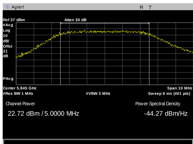
Plot 17. Maximum Conducted Output Power, 5M, 5845, 8Omni, Port 1
