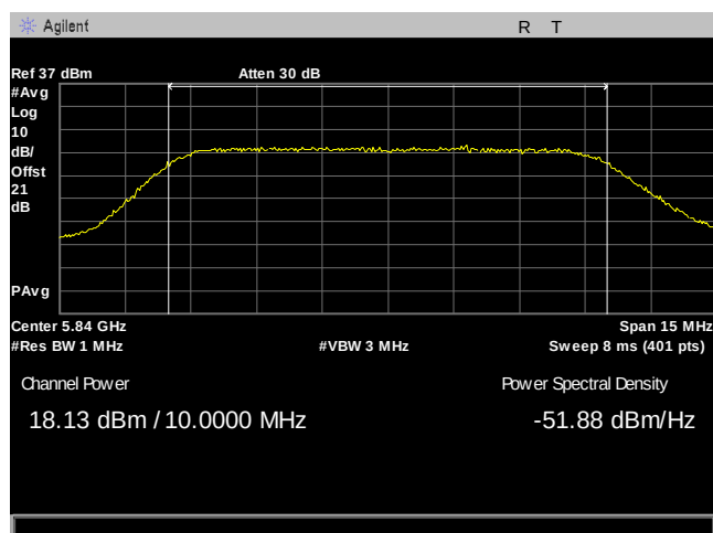
Plot 47. Maximum Conducted Output Power, 10M, 5840, 90Sector, Port 1
