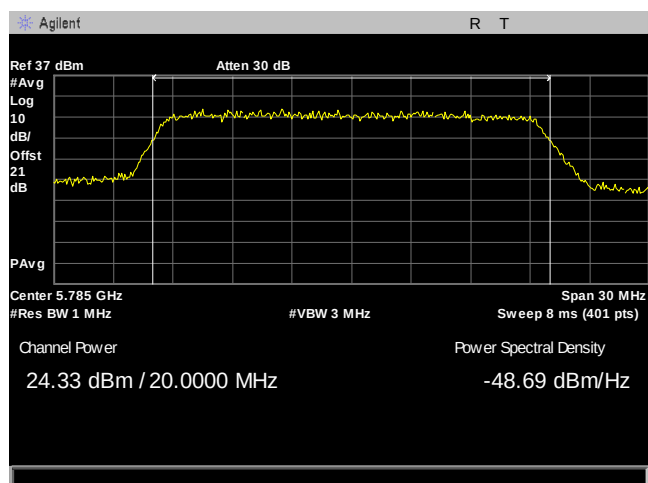
Plot 99. Maximum Conducted Output Power, 20M, 5785, 3Para, Port 1
