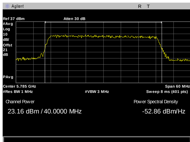
Plot 33. Maximum Conducted Output Power, 40M, 5785, 8Omni, Port 1
