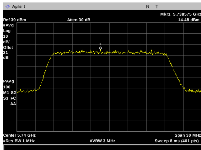
Plot 121. Power Spectral Density, 20M, 5740MHz, 8Omni, Port 1
