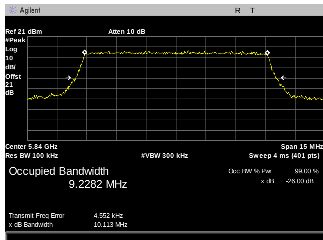
Plot 6. 26 dB Occupied Bandwidth, BW 10MHz, 5840MHz
