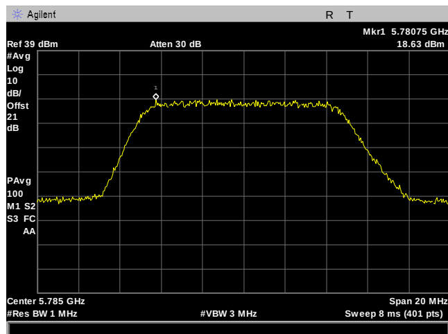
Plot 190. Power Spectral Density, 10M, 5785MHz, 2Para, Port 2
