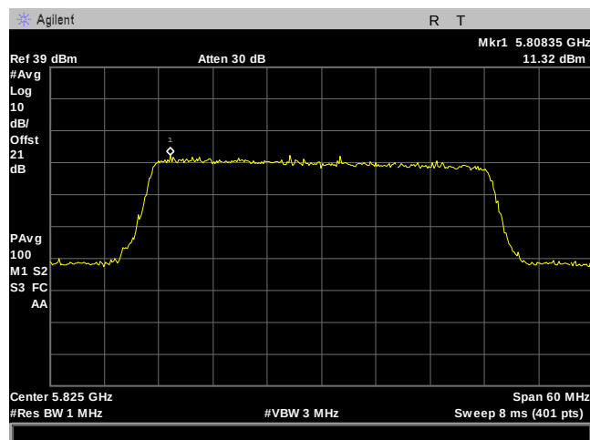
Plot 131. Power Spectral Density, 40M, 5825MHz, 8Omni, Port 1
