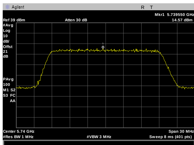
Plot 122. Power Spectral Density, 20M, 5740MHz, 8Omni, Port 2
