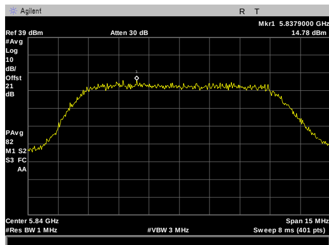
Plot 143. Power Spectral Density, 10M, 5840MHz, 90Sector, Port 1
