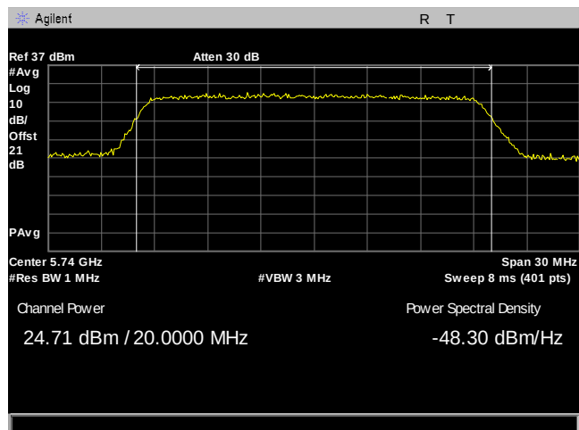
Plot 73. Maximum Conducted Output Power, 20M, 5740, 2Panel, Port 1
