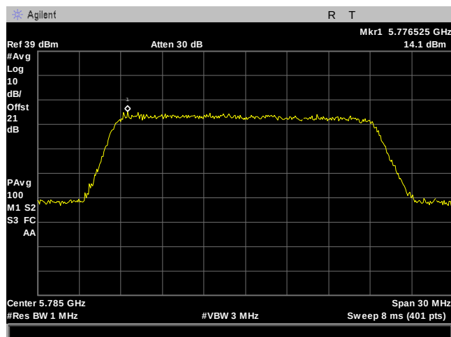
Plot 123. Power Spectral Density, 20M, 5785MHz, 8Omni, Port 1
