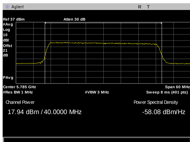
Plot 57. Maximum Conducted Output Power, 40M, 5785, 90Sector, Port 1
