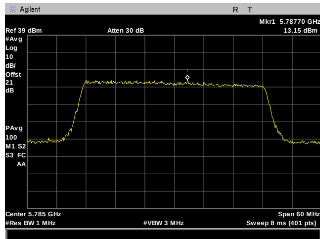
Plot 178. Power Spectral Density, 40M, 5785MHz, 2Panel, Port 2
