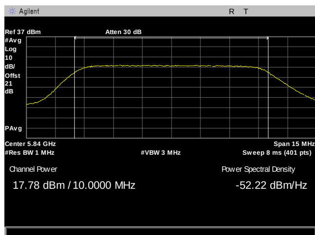
Plot 48. Maximum Conducted Output Power, 10M, 5840, 90Sector, Port 2
