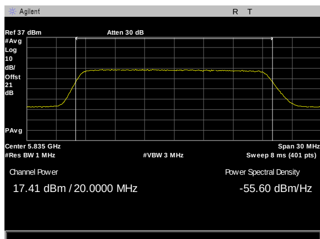
Plot 54. Maximum Conducted Output Power, 20M, 5835, 90Sector, Port 2
