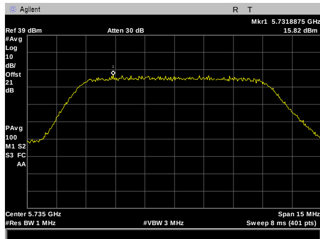
Plot 139. Power Spectral Density, 10M, 5735MHz, 90Sector, Port 1
