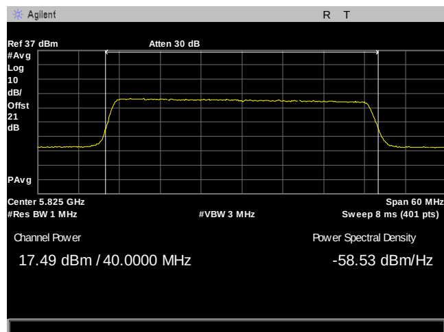
Plot 60. Maximum Conducted Output Power, 40M, 5825, 90Sector, Port 2
