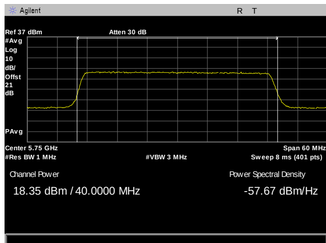
Plot 55. Maximum Conducted Output Power, 40M, 5750, 90Sector, Port 1
