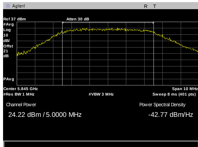
Plot 65. Maximum Conducted Output Power, 5M, 5845, 2Panel, Port 1
