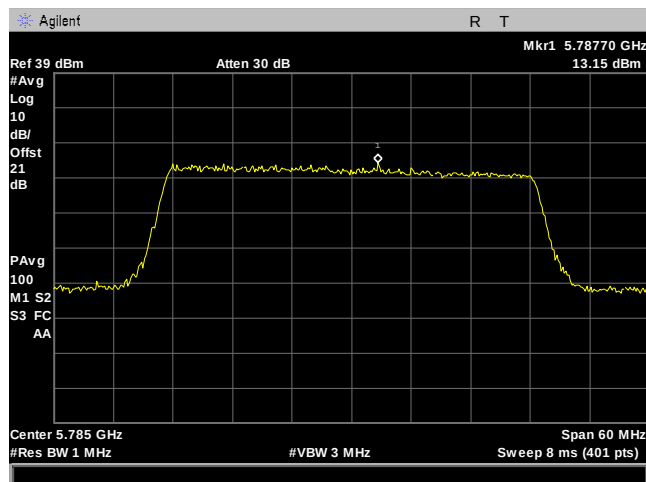
Plot 202. Power Spectral Density, 40M, 5785MHz, 2Para, Port 2
