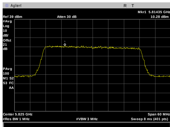
Plot 132. Power Spectral Density, 40M, 5825MHz, 8Omni, Port 2
