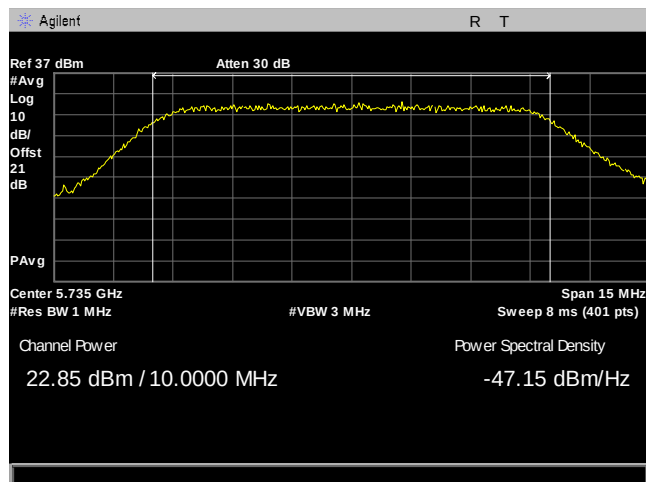
Plot 19. Maximum Conducted Output Power, 10M, 5735, 8Omni, Port 1
