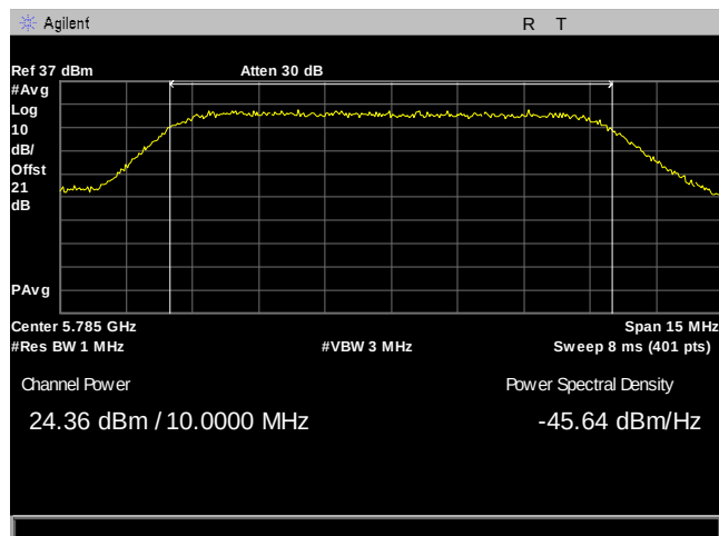
Plot 94. Maximum Conducted Output Power, 10M, 5785, 3Para, Port 2
