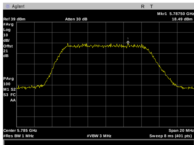
Plot 189. Power Spectral Density, 10M, 5785MHz, 2Para, Port 1
