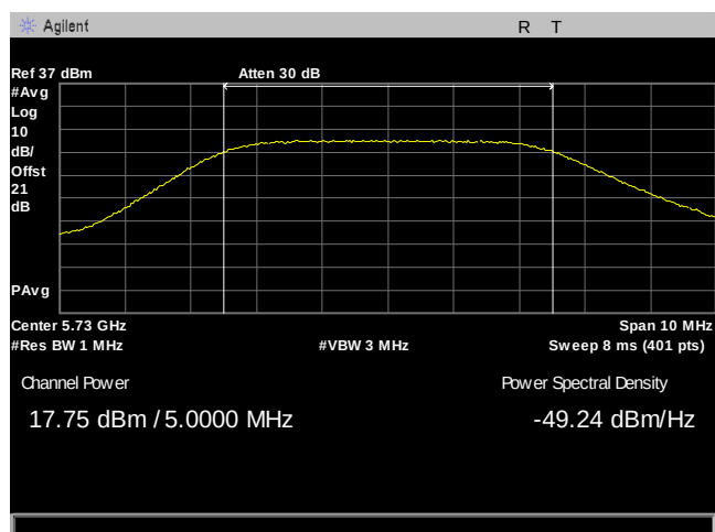
Plot 38. Maximum Conducted Output Power, 5M, 5730, 90Sector, Port 2
