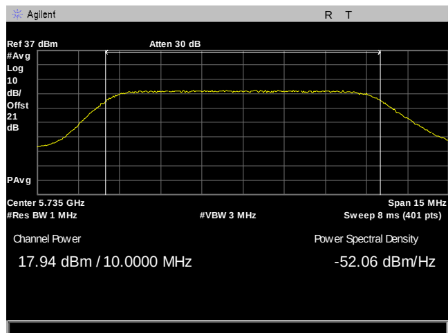
Plot 43. Maximum Conducted Output Power, 10M, 5735, 90Sector, Port 1
