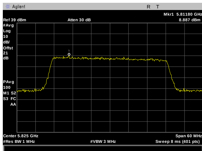
Plot 156. Power Spectral Density, 40M, 5825MHz, 90Sector, Port 2
