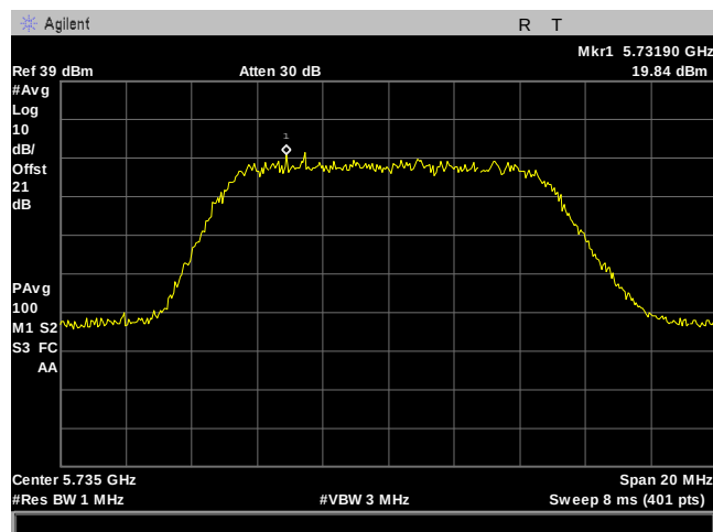
Plot 164. Power Spectral Density, 10M, 5735MHz, 2Panel, Port 2
