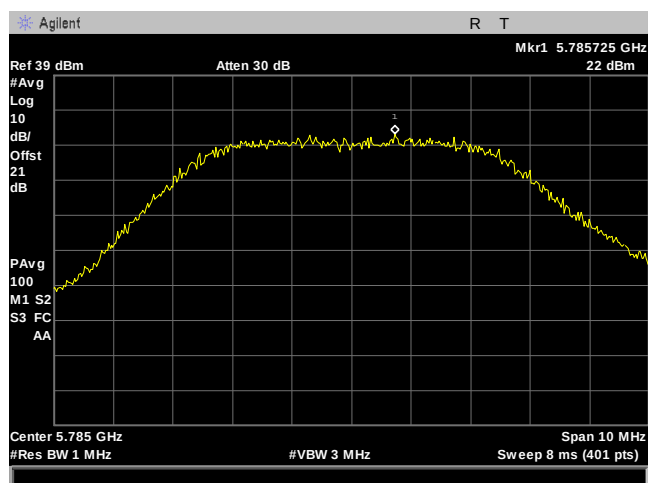
Plot 183. Power Spectral Density, 5M, 5785MHz, 2Para, Port 1
