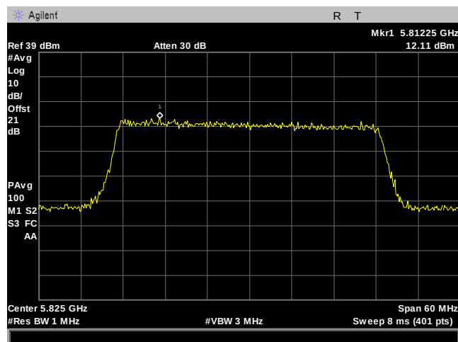
Plot 179. Power Spectral Density, 40M, 5825MHz, 2Panel, Port 1
