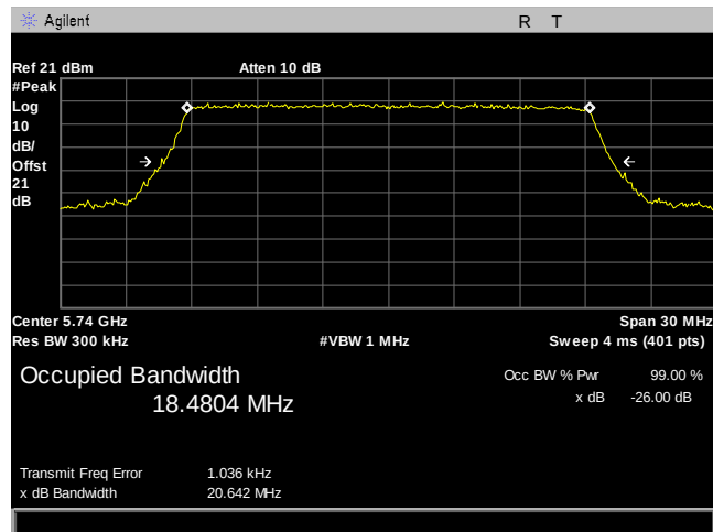
Plot 7. 26 dB Occupied Bandwidth, BW 20MHz, 5740MHz
