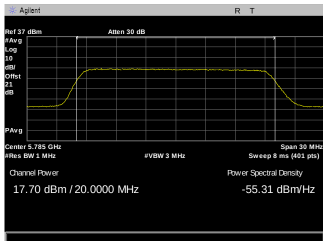
Plot 52. Maximum Conducted Output Power, 20M, 5785, 90Sector, Port 2
