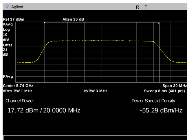
Plot 50. Maximum Conducted Output Power, 20M, 5740, 90Sector, Port 2
