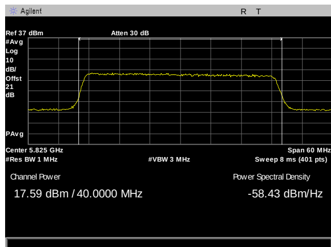
Plot 59. Maximum Conducted Output Power, 40M, 5825, 90Sector, Port 1
