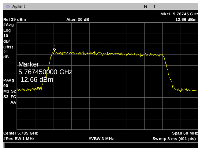
Plot 201. Power Spectral Density, 40M, 5785MHz, 2Para, Port 1
