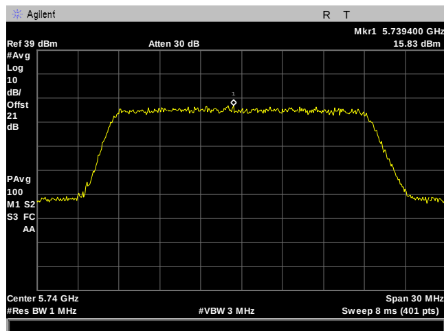
Plot 169. Power Spectral Density, 20M, 5740MHz, 2Panel, Port 1
