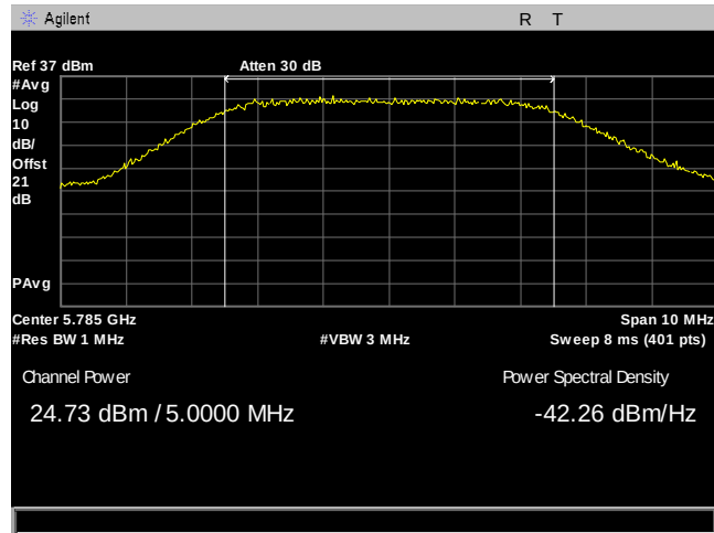
Plot 64. Maximum Conducted Output Power, 5M, 5785, 2Panel, Port 2
