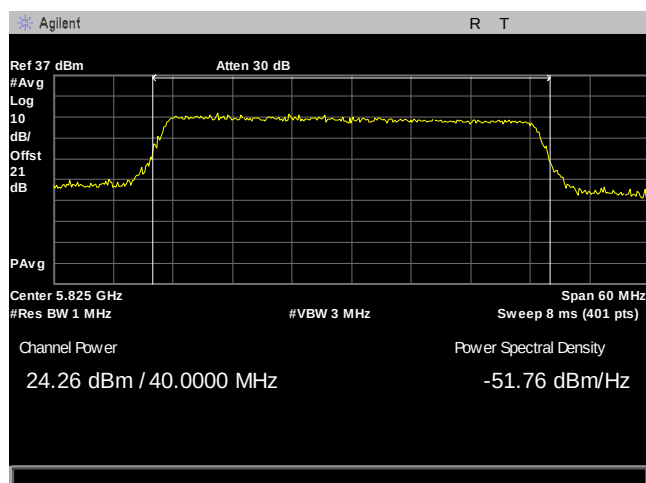
Plot 84. Maximum Conducted Output Power, 40M, 5825, 2Panel, Port 2
