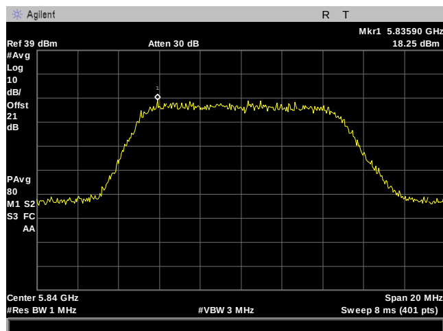
Plot 192. Power Spectral Density, 10M, 5840MHz, 2Para, Port 2
