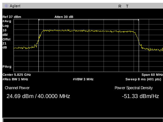
Plot 107. Maximum Conducted Output Power, 40M, 5825, 3Para, Port 1
