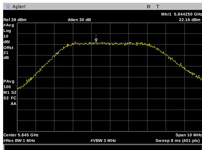
Plot 162. Power Spectral Density, 5M, 5845MHz, 2Panel, Port 2
