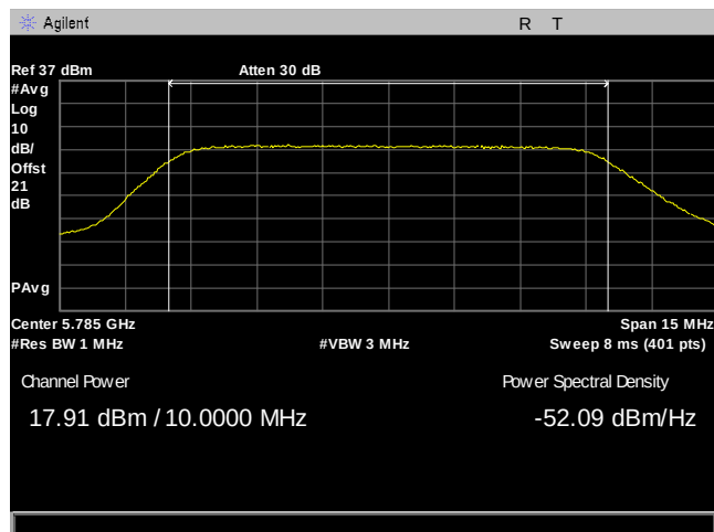
Plot 46. Maximum Conducted Output Power, 10M, 5785, 90Sector, Port 2
