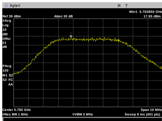
Plot 135. Power Spectral Density, 5M, 5785MHz, 90Sector, Port 1
