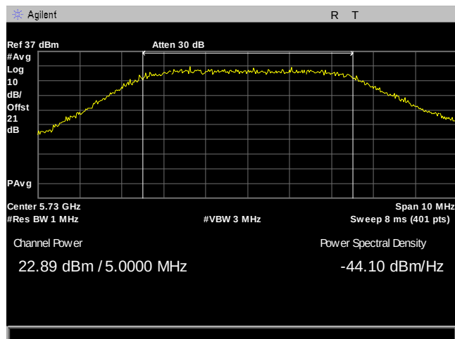
Plot 13. Maximum Conducted Output Power, 5M, 5730, 8Omni, Port 1
