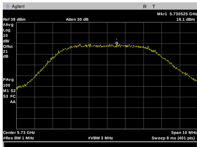
Plot 133. Power Spectral Density, 5M, 5730MHz, 90Sector, Port 1
