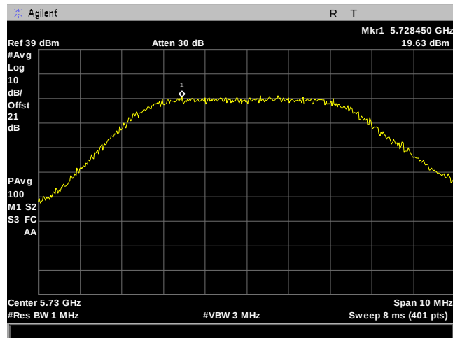
Plot 109. Power Spectral Density, 5M, 5730MHz, 8Omni, Port 1
