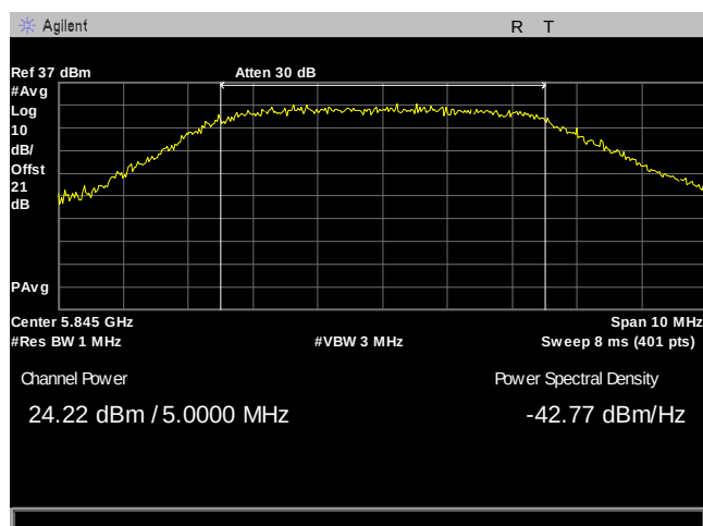
Plot 89. Maximum Conducted Output Power, 5M, 5845, 3Para, Port 1
