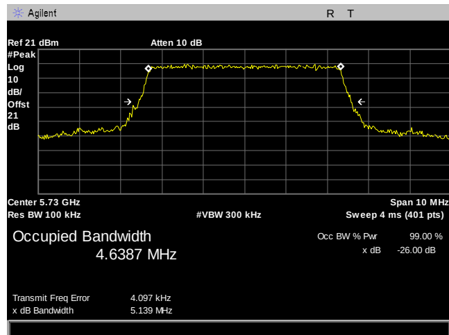
Plot 1. 26 dB Occupied Bandwidth, BW 5MHz, 5730MHz
