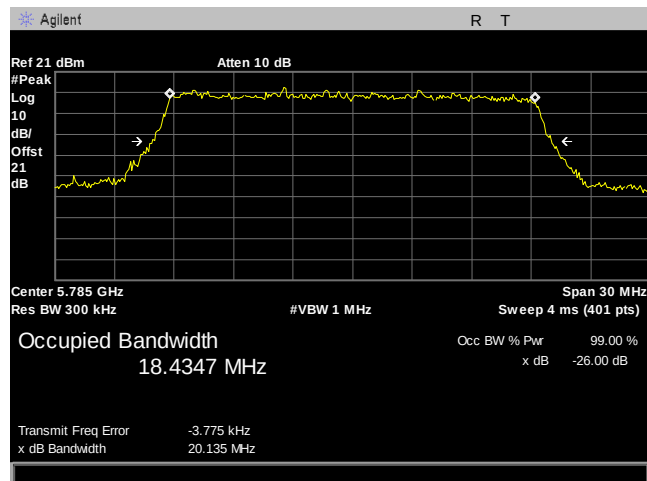
Plot 8. 26 dB Occupied Bandwidth, BW 20MHz, 5785MHz
