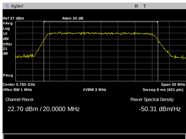
Plot 27. Maximum Conducted Output Power, 20M, 5785, 8Omni, Port 1
