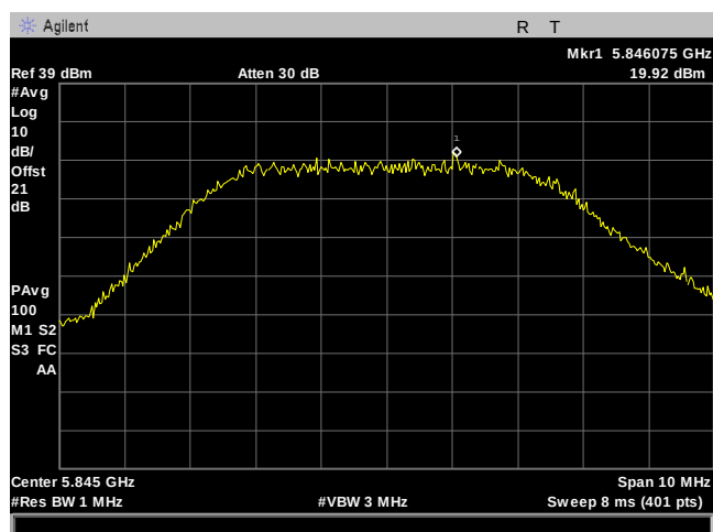
Plot 113. Power Spectral Density, 5M, 5845MHz, 8Omni, Port 1
