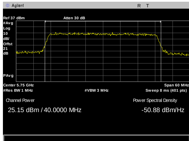
Plot 79. Maximum Conducted Output Power, 40M, 5750, 2Panel, Port 1
