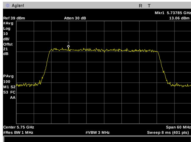
Plot 199. Power Spectral Density, 40M, 5750MHz, 2Para, Port 1
