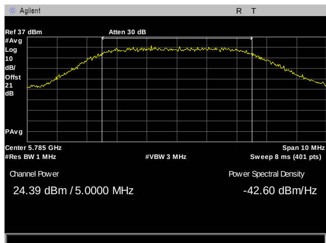
Plot 87. Maximum Conducted Output Power, 5M, 5785, 3Para, Port 1
