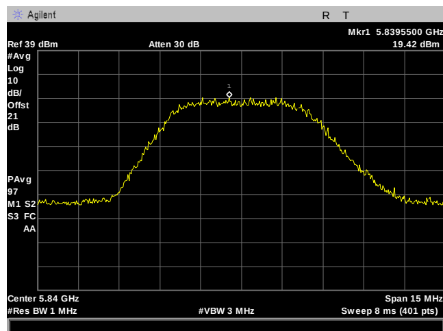
Plot 119. Power Spectral Density, 10M, 5840MHz, 8Omni, Port 1
