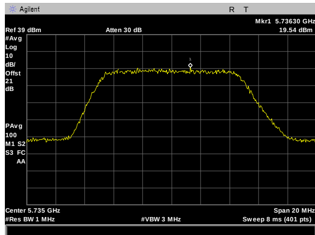
Plot 187. Power Spectral Density, 10M, 5735MHz, 2Para, Port 1
