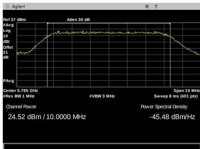
Plot 69. Maximum Conducted Output Power, 10M, 5785, 2Panel, Port 1
