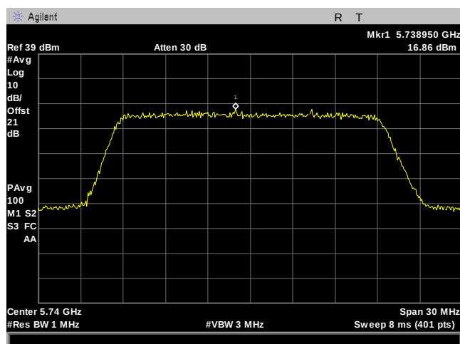
Plot 170. Power Spectral Density, 20M, 5740MHz, 2Panel, Port 2
