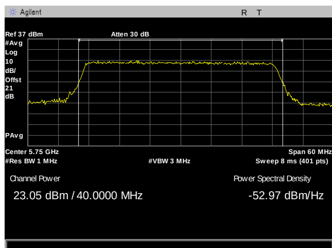
Plot 32. Maximum Conducted Output Power, 40M, 5750, 8Omni, Port 2
