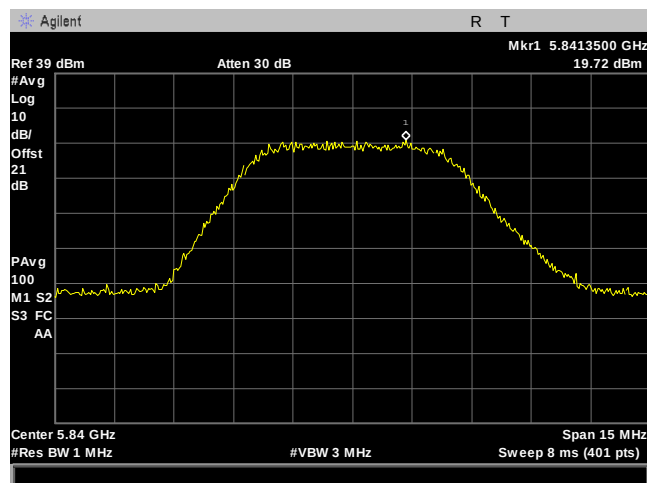
Plot 120. Power Spectral Density, 10M, 5840MHz, 8Omni, Port 2
