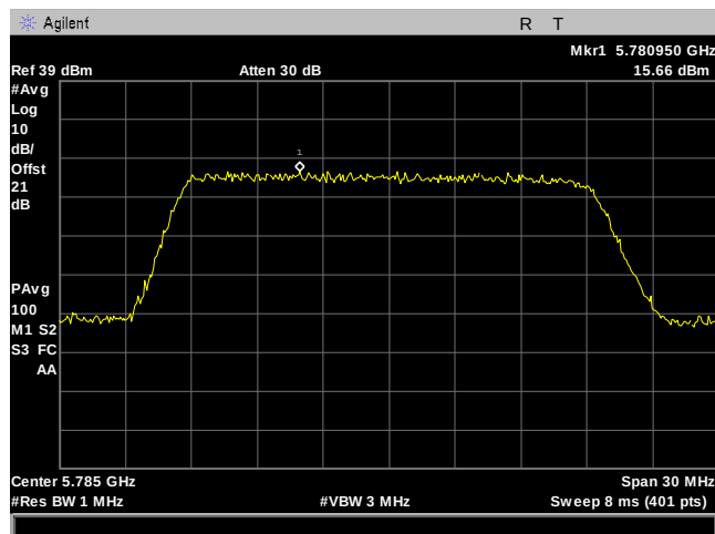
Plot 196. Power Spectral Density, 20M, 5785MHz, 2Para, Port 2
