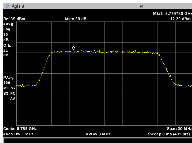
Plot 147. Power Spectral Density, 20M, 5785MHz, 90Sector, Port 1
