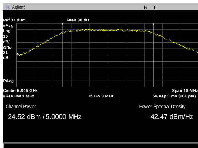
Plot 90. Maximum Conducted Output Power, 5M, 5845, 3Para, Port 2
