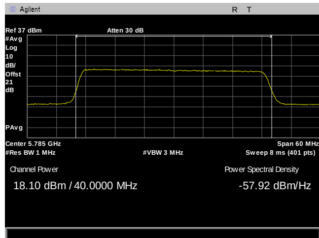
Plot 58. Maximum Conducted Output Power, 40M, 5785, 90Sector, Port 2
