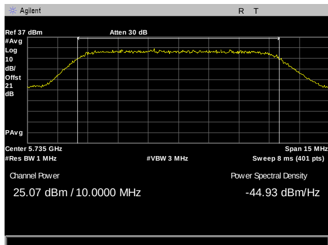
Plot 92. Maximum Conducted Output Power, 10M, 5735, 3Para, Port 2
