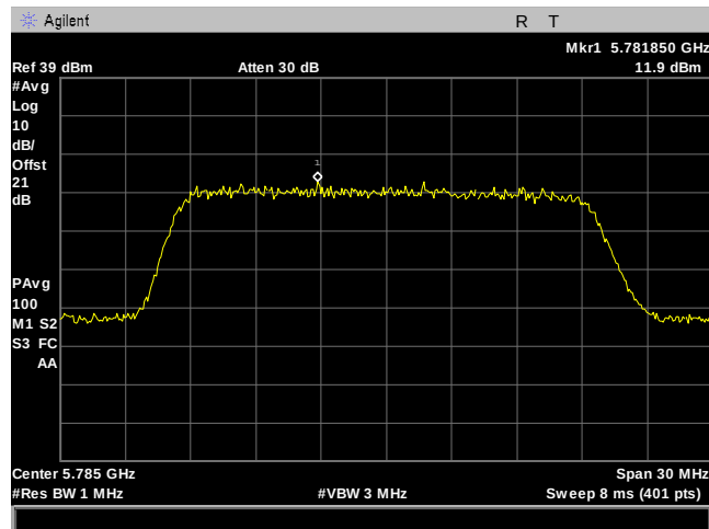
Plot 148. Power Spectral Density, 20M, 5785MHz, 90Sector, Port 2
