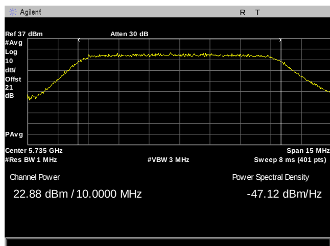
Plot 20. Maximum Conducted Output Power, 10M, 5735, 8Omni, Port 2
