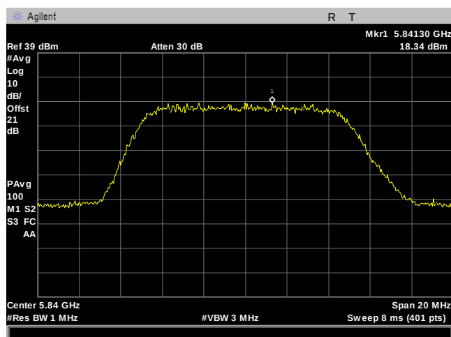
Plot 191. Power Spectral Density, 10M, 5840MHz, 2Para, Port 1
