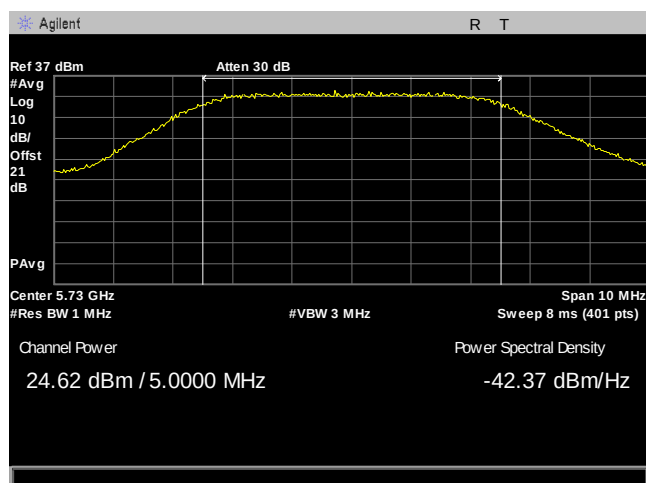
Plot 62. Maximum Conducted Output Power, 5M, 5730, 2Panel, Port 2
