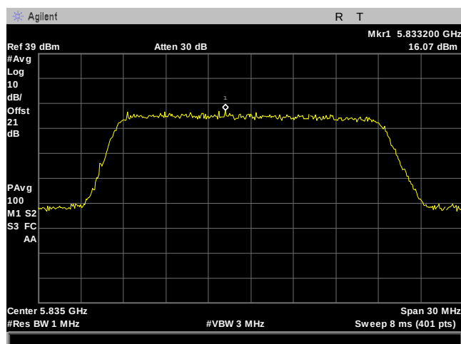
Plot 198. Power Spectral Density, 20M, 5835MHz, 2Para, Port 2
