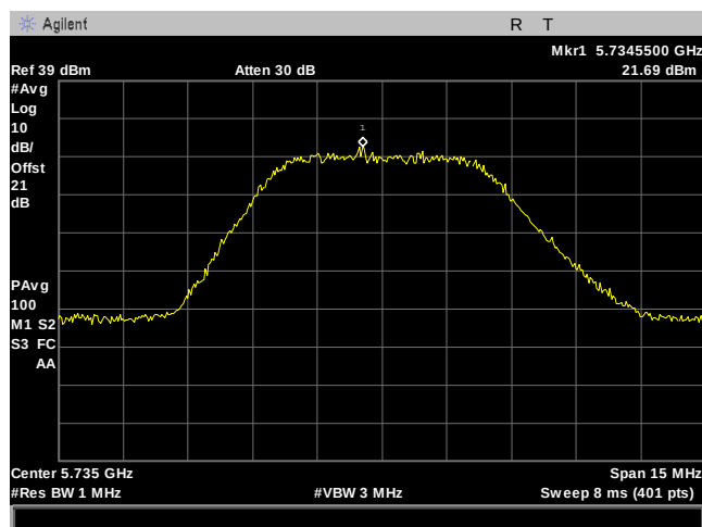
Plot 116. Power Spectral Density, 10M, 5735MHz, 8Omni, Port 2
