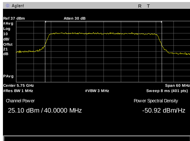
Plot 104. Maximum Conducted Output Power, 40M, 5750, 3Para, Port 2
