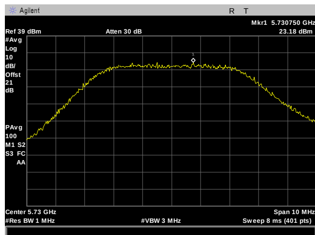
Plot 158. Power Spectral Density, 5M, 5730MHz, 2Panel, Port 2
