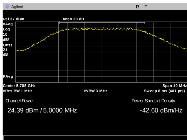
Plot 63. Maximum Conducted Output Power, 5M, 5785, 2Panel, Port 1
