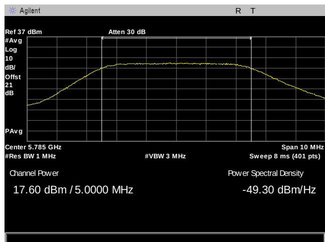
Plot 39. Maximum Conducted Output Power, 5M, 5785, 90Sector, Port 1
