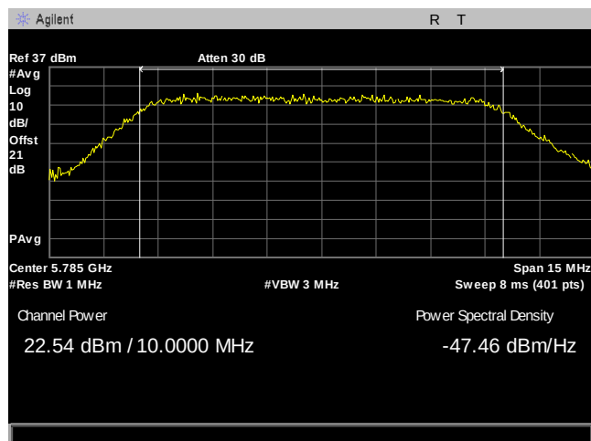
Plot 21. Maximum Conducted Output Power, 10M, 5785, 8Omni, Port 1
