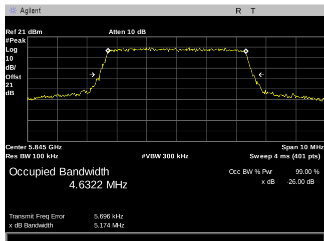
Plot 3. 26 dB Occupied Bandwidth, BW 5MHz, 5845MHz
