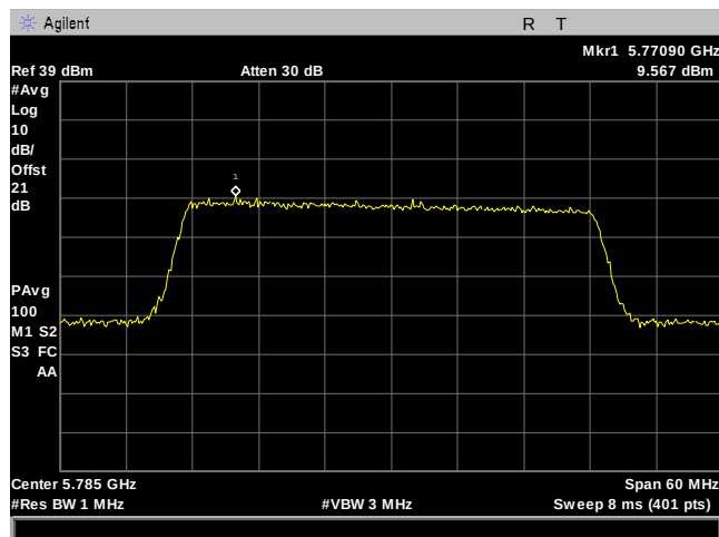
Plot 154. Power Spectral Density, 40M, 5785MHz, 90Sector, Port 2
