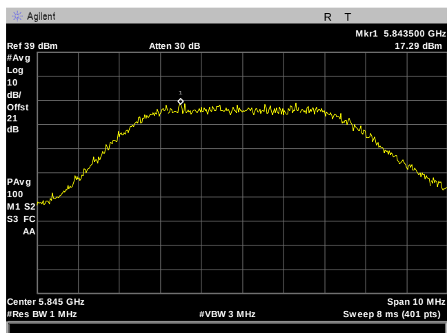
Plot 137. Power Spectral Density, 5M, 5845MHz, 90Sector, Port 1
