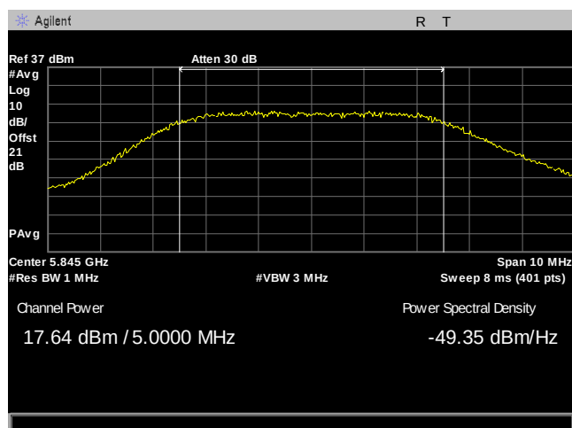
Plot 41. Maximum Conducted Output Power, 5M, 5845, 90Sector, Port 1
