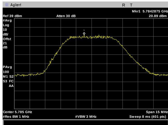
Plot 118. Power Spectral Density, 10M, 5785MHz, 8Omni, Port 2
