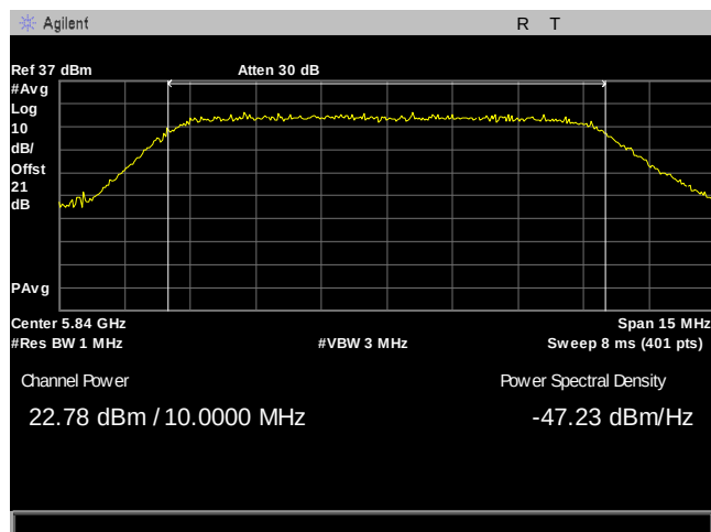
Plot 24. Maximum Conducted Output Power, 10M, 5840, 8Omni, Port 2
