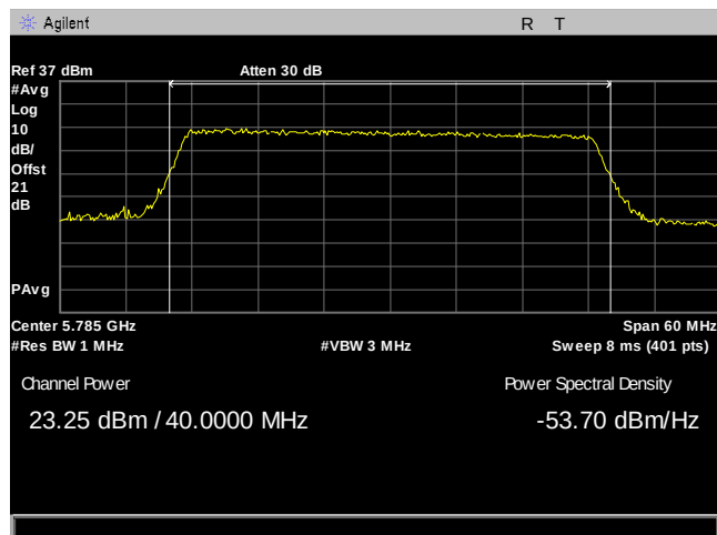
Plot 34. Maximum Conducted Output Power, 40M, 5785, 8Omni, Port 2
