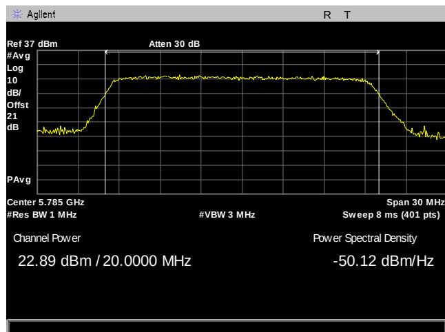
Plot 28. Maximum Conducted Output Power, 20M, 5785, 8Omni, Port 2
