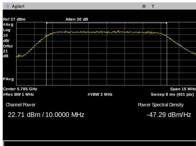
Plot 22. Maximum Conducted Output Power, 10M, 5785, 8Omni, Port 2
