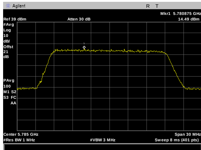
Plot 124. Power Spectral Density, 20M, 5785MHz, 8Omni, Port 2
