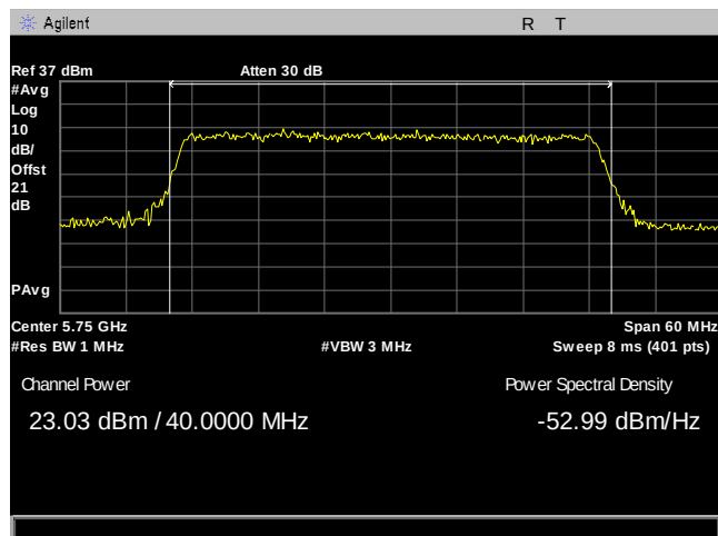
Plot 31. Maximum Conducted Output Power, 40M, 5750, 8Omni, Port 1
