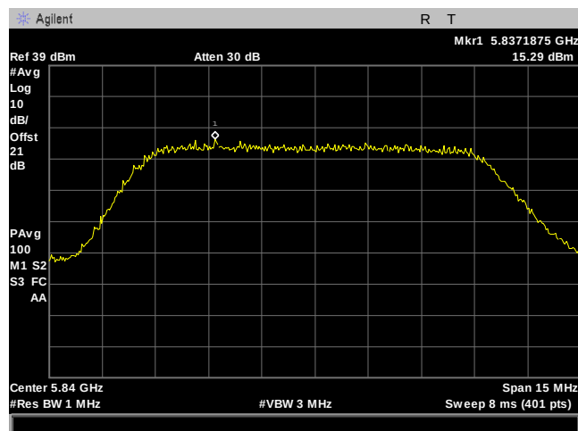
Plot 144. Power Spectral Density, 10M, 5840MHz, 90Sector, Port 2
