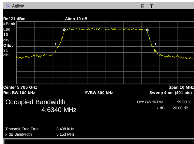
Plot 2. 26 dB Occupied Bandwidth, BW 5MHz, 5785MHz
