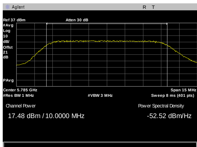
Plot 45. Maximum Conducted Output Power, 10M, 5785, 90Sector, Port 1
