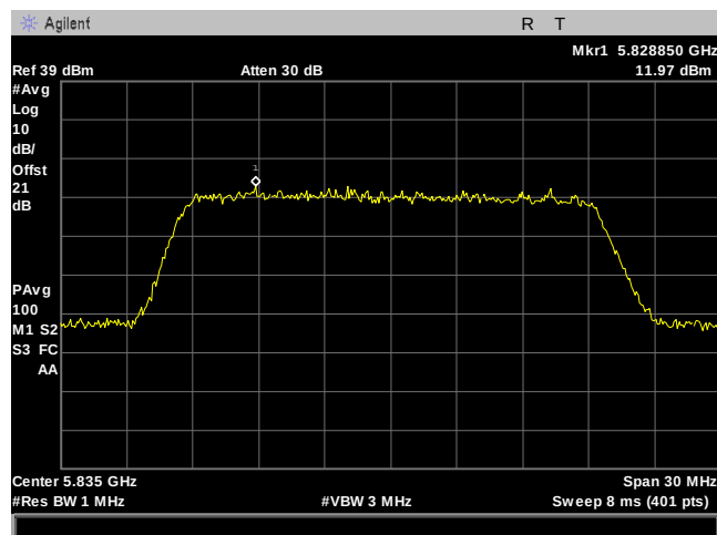
Plot 150. Power Spectral Density, 20M, 5835MHz, 90Sector, Port 2
