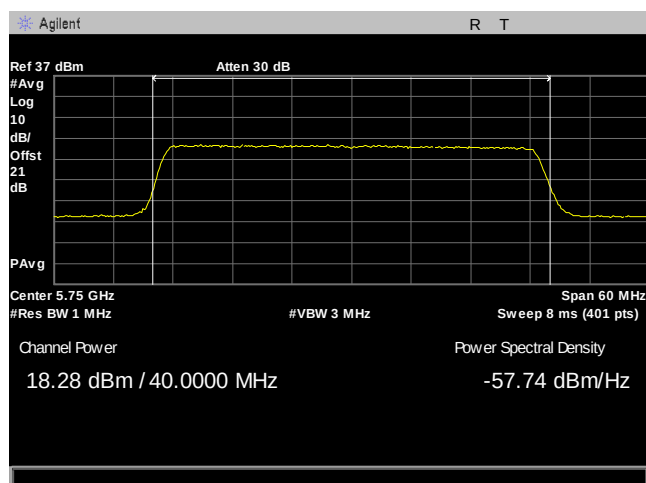
Plot 56. Maximum Conducted Output Power, 40M, 5750, 90Sector, Port 2
