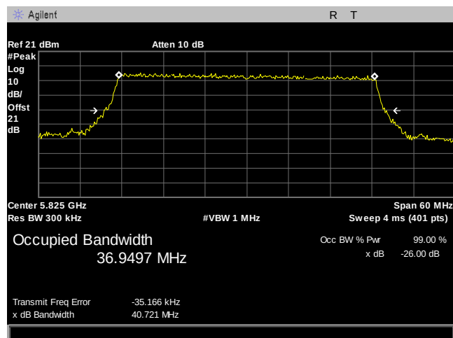
Plot 12. 26 dB Occupied Bandwidth, BW 40MHz, 5825MHz
