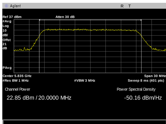
Plot 30. Maximum Conducted Output Power, 20M, 5835, 8Omni, Port 2
