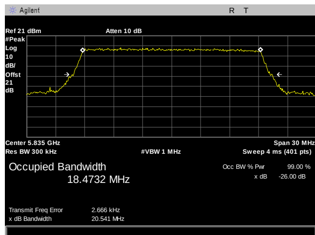
Plot 9. 26 dB Occupied Bandwidth, BW 20MHz, 5835MHz
