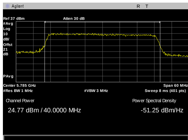
Plot 105. Maximum Conducted Output Power, 40M, 5785, 3Para, Port 1
