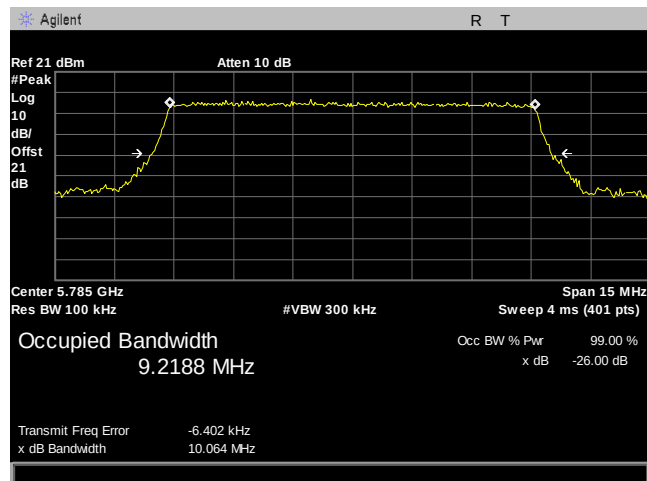
Plot 5. 26 dB Occupied Bandwidth, BW 10MHz, 5785MHz
