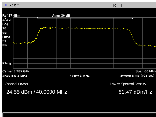
Plot 82. Maximum Conducted Output Power, 40M, 5785, 2Panel, Port 2
