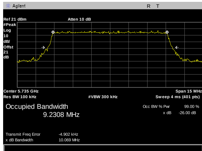
Plot 4. 26 dB Occupied Bandwidth, BW 10MHz, 5735MHz
