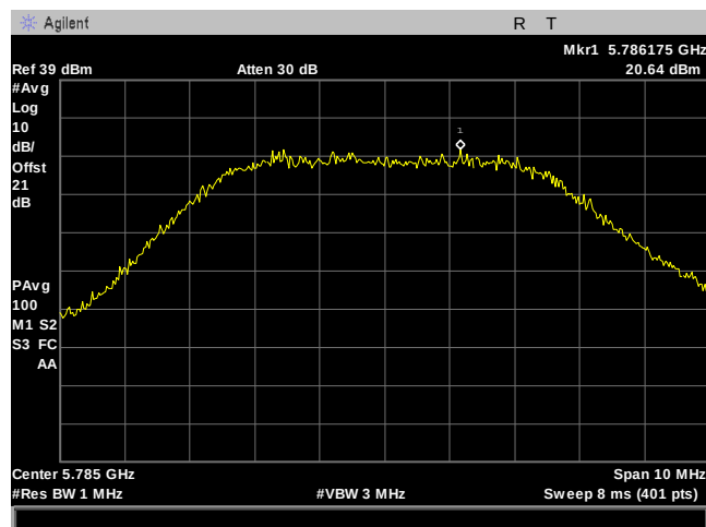
Plot 111. Power Spectral Density, 5M, 5785MHz, 8Omni, Port 1
