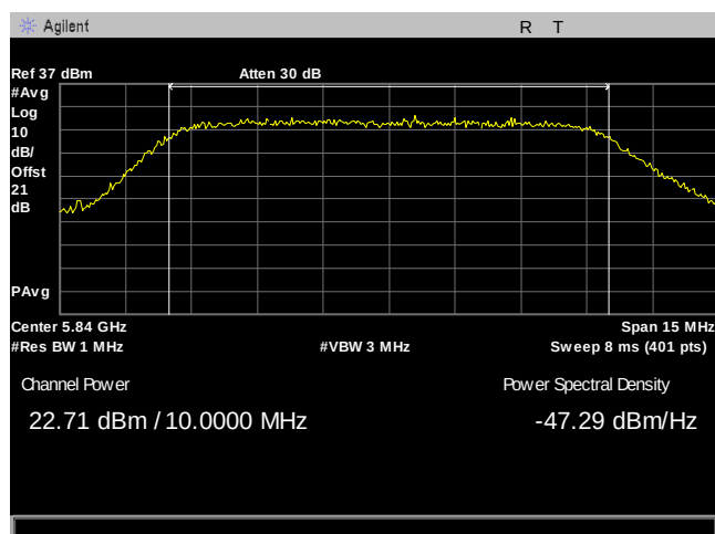
Plot 23. Maximum Conducted Output Power, 10M, 5840, 8Omni, Port 1
