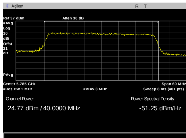
Plot 81. Maximum Conducted Output Power, 40M, 5785, 2Panel, Port 1
