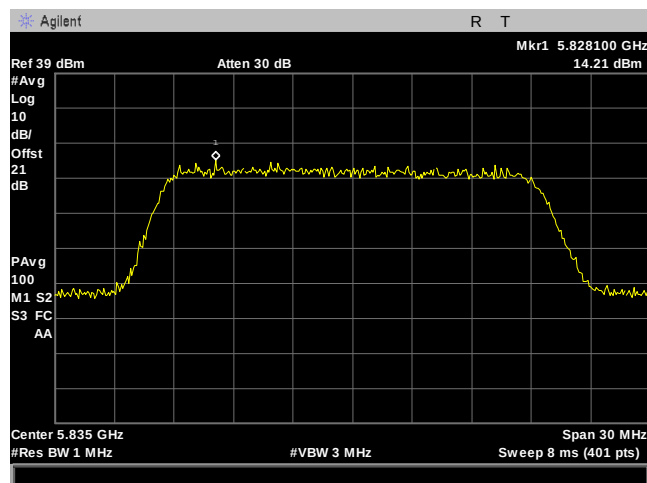
Plot 126. Power Spectral Density, 20M, 5835MHz, 8Omni, Port 2
