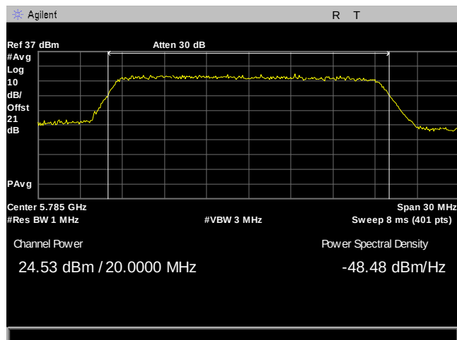
Plot 100. Maximum Conducted Output Power, 20M, 5785, 3Para, Port 2
