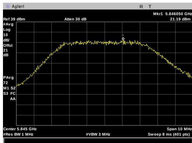
Plot 185. Power Spectral Density, 5M, 5845MHz, 2Para, Port 1
