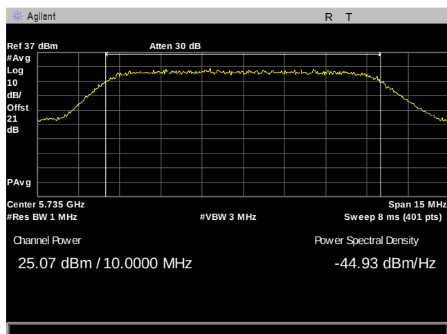
Plot 68. Maximum Conducted Output Power, 10M, 5735, 2Panel, Port 2
