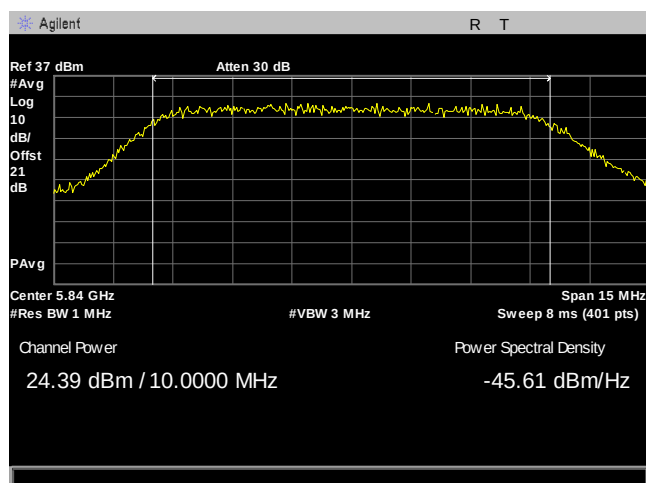
Plot 95. Maximum Conducted Output Power, 10M, 5840, 3Para, Port 1
