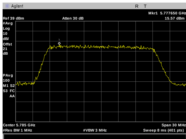
Plot 195. Power Spectral Density, 20M, 5785MHz, 2Para, Port 1
