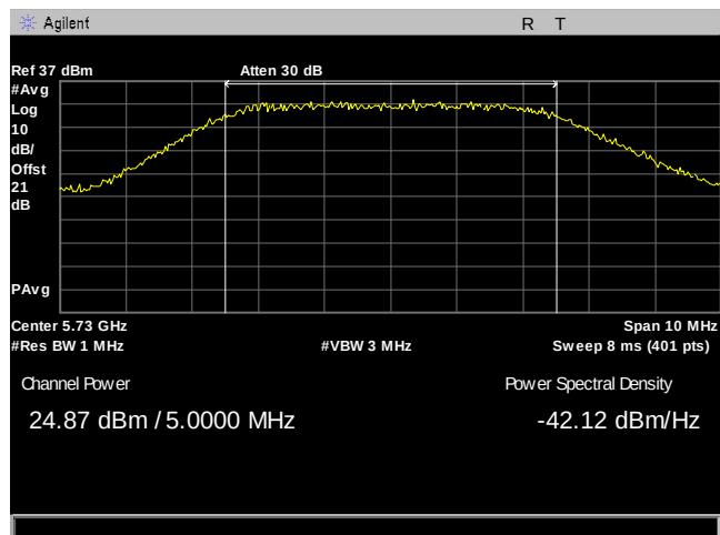
Plot 85. Maximum Conducted Output Power, 5M, 5730, 3Para, Port 1
