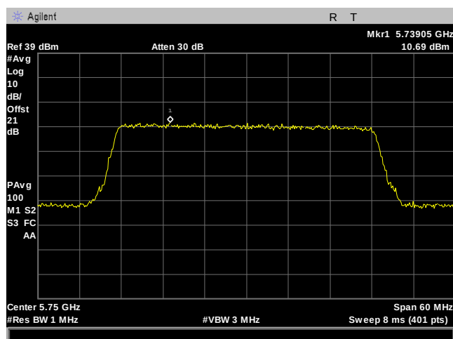
Plot 128. Power Spectral Density, 40M, 5750MHz, 8Omni, Port 2
