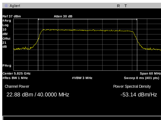
Plot 36. Maximum Conducted Output Power, 40M, 5825, 8Omni, Port 2
