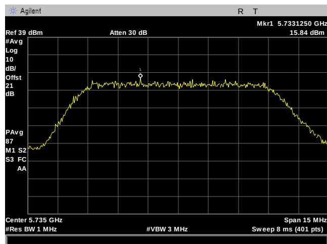
Plot 140. Power Spectral Density, 10M, 5735MHz, 90Sector, Port 2
