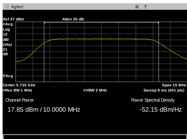
Plot 44. Maximum Conducted Output Power, 10M, 5735, 90Sector, Port 2
