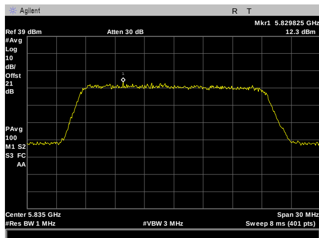
Plot 149. Power Spectral Density, 20M, 5835MHz, 90Sector, Port 1
