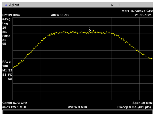
Plot 181. Power Spectral Density, 5M, 5730MHz, 2Para, Port 1
