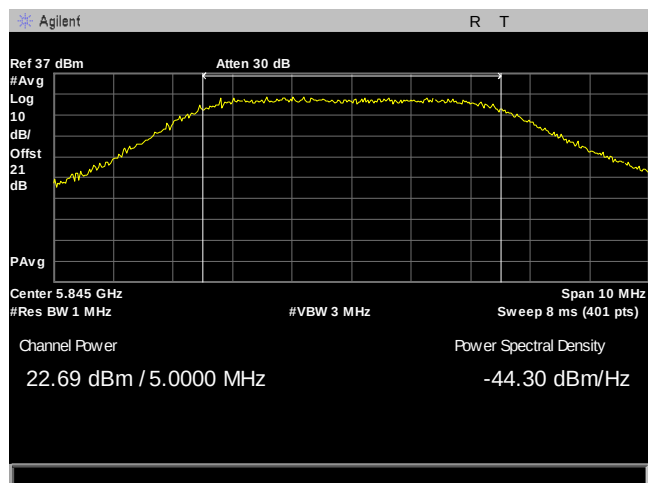
Plot 18. Maximum Conducted Output Power, 5M, 5845, 8Omni, Port 2
