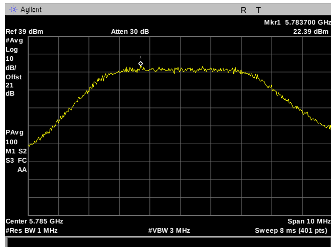
Plot 184. Power Spectral Density, 5M, 5785MHz, 2Para, Port 2
