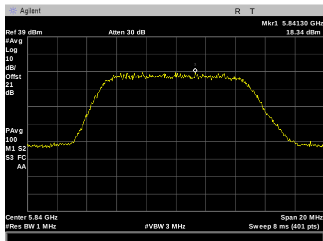
Plot 167. Power Spectral Density, 10M, 5840MHz, 2Panel, Port 1
