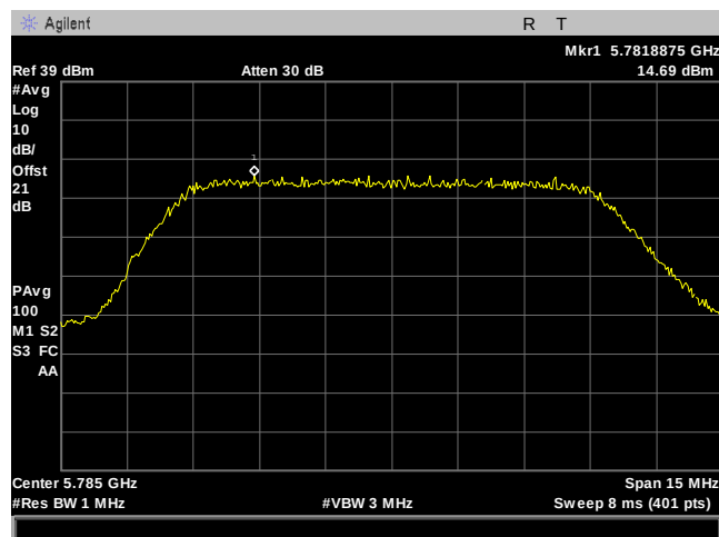
Plot 141. Power Spectral Density, 10M, 5785MHz, 90Sector, Port 1
