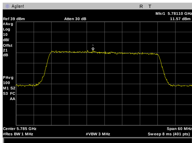
Plot 129. Power Spectral Density, 40M, 5785MHz, 8Omni, Port 1
