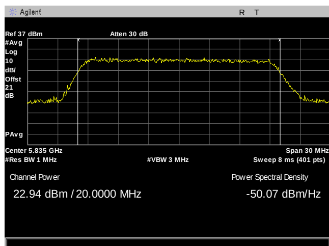
Plot 29. Maximum Conducted Output Power, 20M, 5835, 8Omni, Port 1
