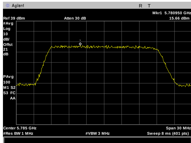
Plot 172. Power Spectral Density, 20M, 5785MHz, 2Panel, Port 2
