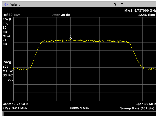
Plot 145. Power Spectral Density, 20M, 5740MHz, 90Sector, Port 1
