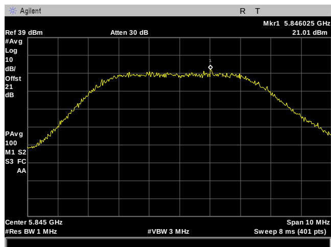
Plot 114. Power Spectral Density, 5M, 5845MHz, 8Omni, Port 2
