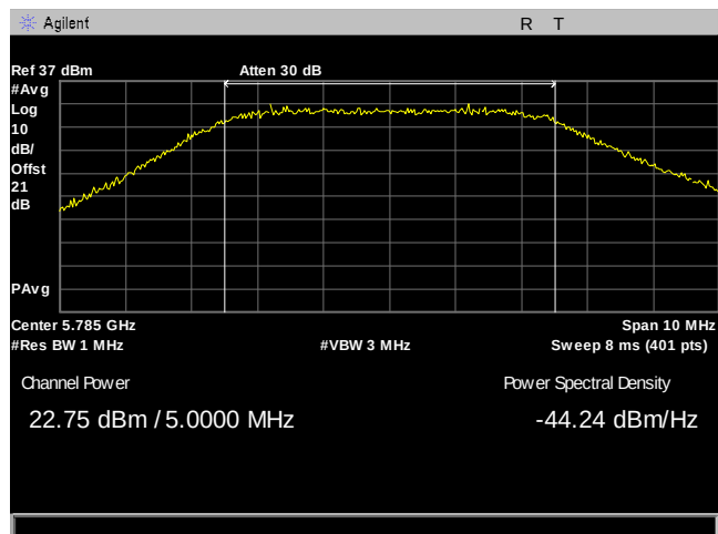
Plot 16. Maximum Conducted Output Power, 5M, 5785, 8Omni, Port 2
