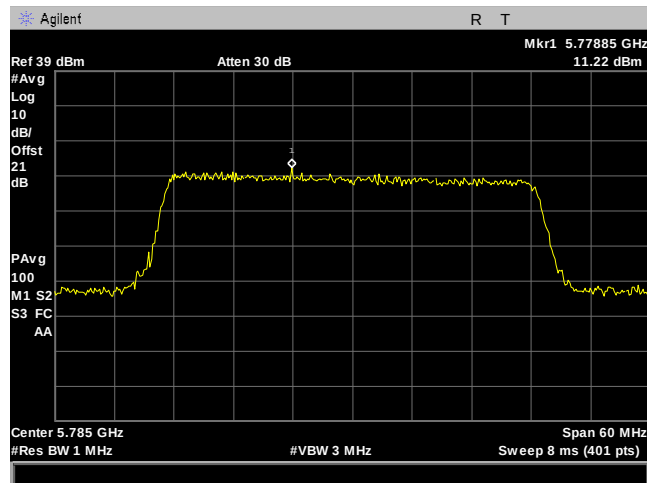
Plot 130. Power Spectral Density, 40M, 5785MHz, 8Omni, Port 2
