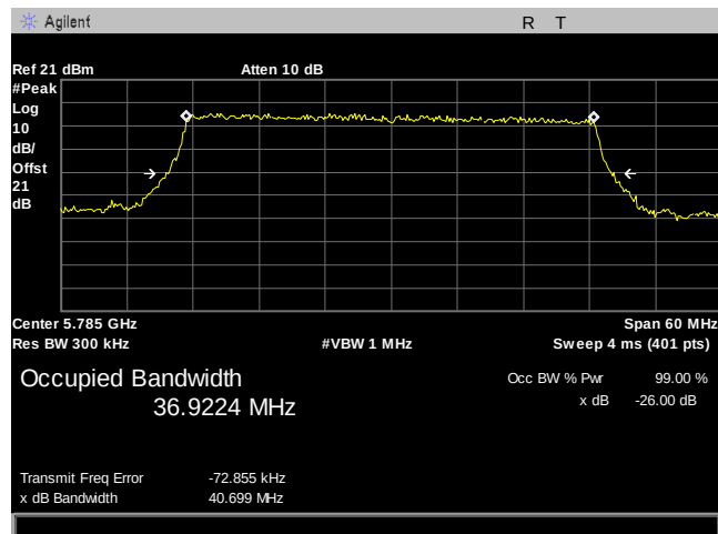
Plot 11. 26 dB Occupied Bandwidth, BW 40MHz, 5785MHz
