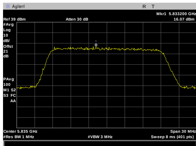
Plot 174. Power Spectral Density, 20M, 5835MHz, 2Panel, Port 2
