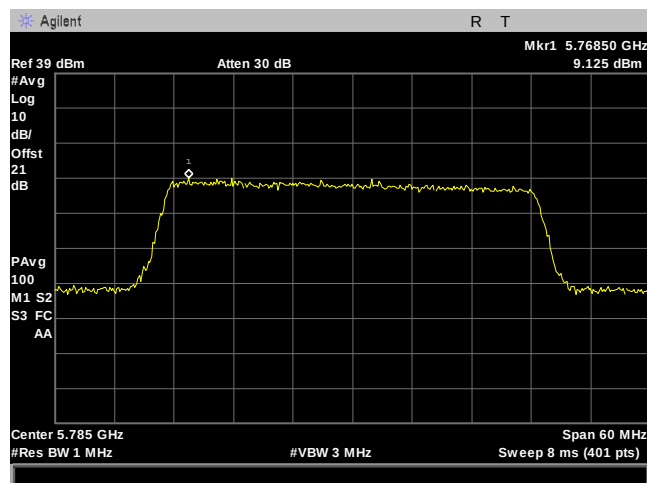
Plot 153. Power Spectral Density, 40M, 5785MHz, 90Sector, Port 1
