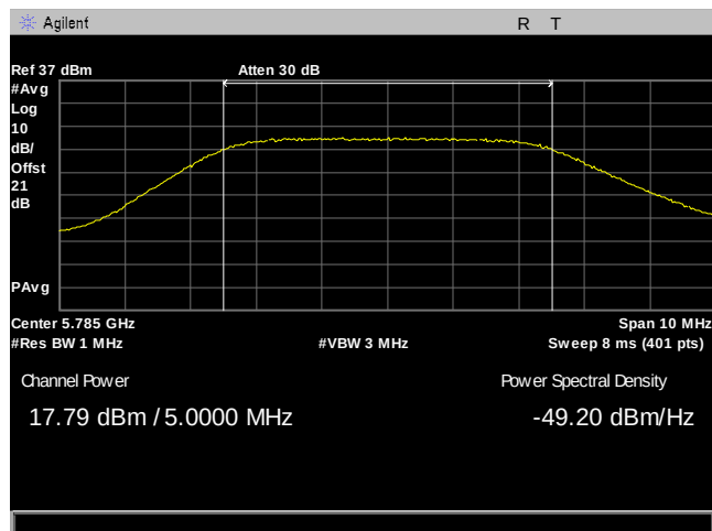
Plot 40. Maximum Conducted Output Power, 5M, 5785, 90Sector, Port 2
