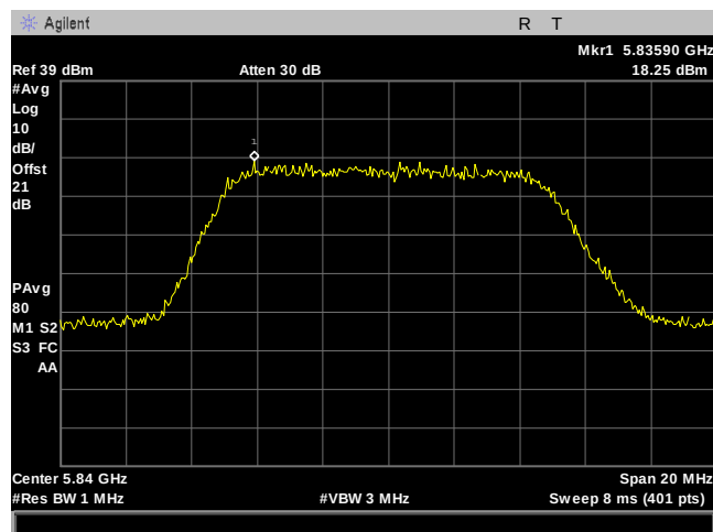
Plot 168. Power Spectral Density, 10M, 5840MHz, 2Panel, Port 2
