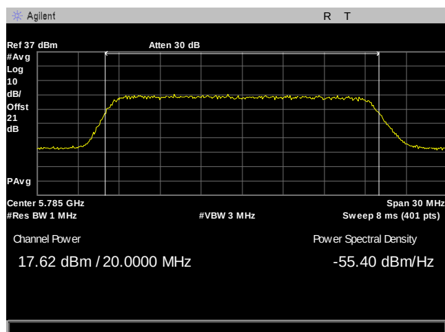
Plot 51. Maximum Conducted Output Power, 20M, 5785, 90Sector, Port 1
