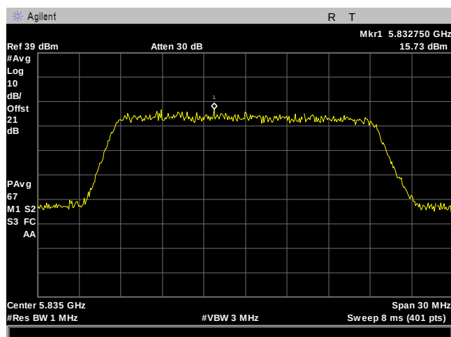
Plot 197. Power Spectral Density, 20M, 5835MHz, 2Para, Port 1
