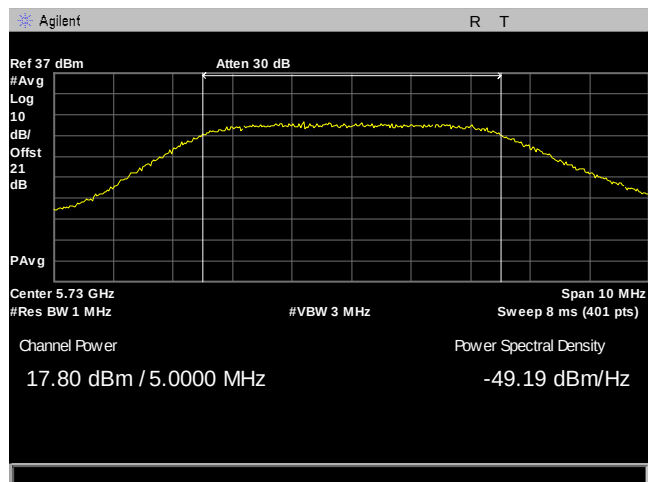
Plot 37. Maximum Conducted Output Power, 5M, 5730, 90Sector, Port 1
