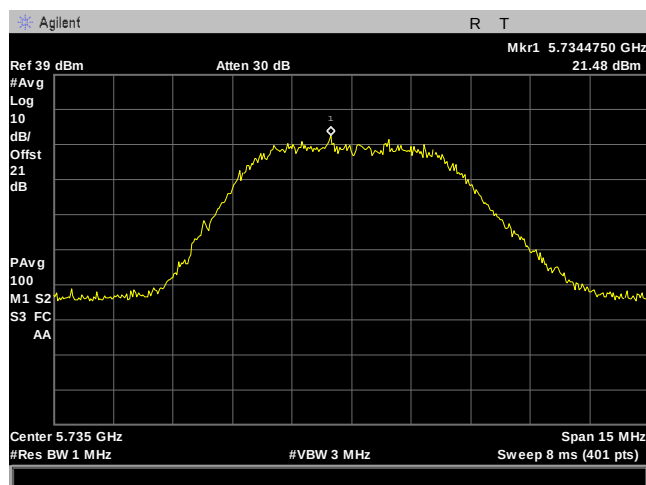
Plot 115. Power Spectral Density, 10M, 5735MHz, 8Omni, Port 1
