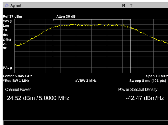
Plot 66. Maximum Conducted Output Power, 5M, 5845, 2Panel, Port 2
