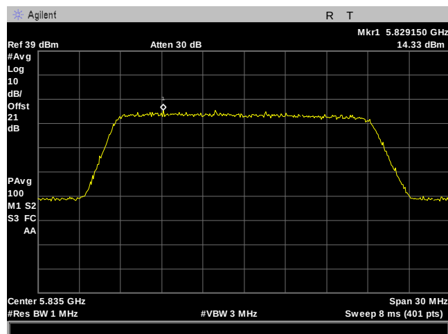
Plot 125. Power Spectral Density, 20M, 5835MHz, 8Omni, Port 1
