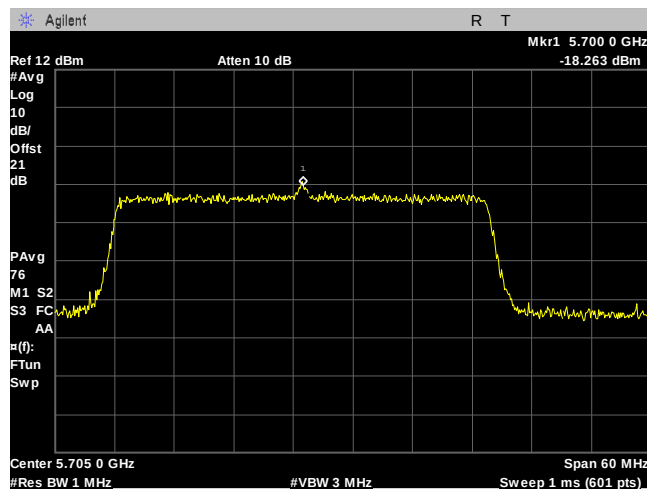
Plot 406. Power Spectral Density, 3 Para, 40MHz, 5700MHz, Port 1
