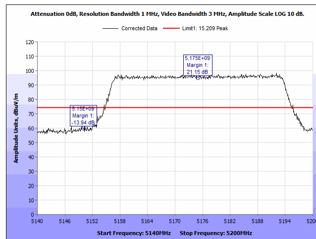
Plot 444. Radiated Band Edge, 5175MHz, BW40MHz, Peak, 90Sector Port1
