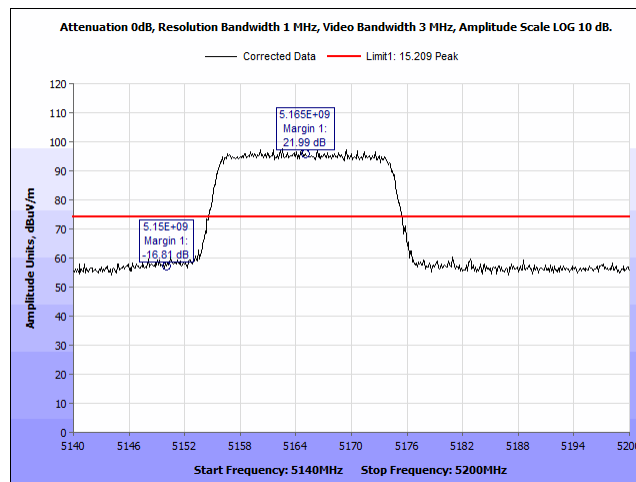
Plot 457. Radiated Band Edge, 5165MHz, BW20MHz, Peak, 2Panel Port2
