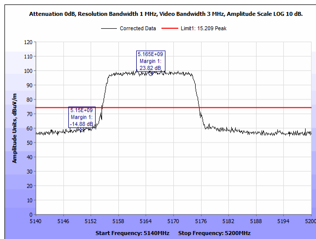
Plot 441. Radiated Band Edge, 5165MHz, BW20MHz, Peak, 90Sector Port2
