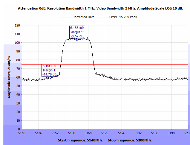
Plot 421. Radiated Band Edge, 5160MHz, BW10MHz, Peak, 3Para Port2
