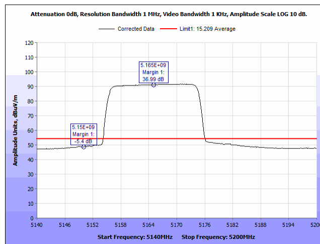
Plot 422. Radiated Band Edge, 5165MHz, BW20MHz, Average, 3Para Port1
