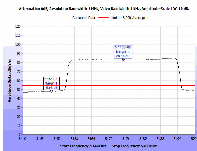
Plot 459. Radiated Band Edge, 5175MHz, BW40MHz, Average, 2Panel Port2
