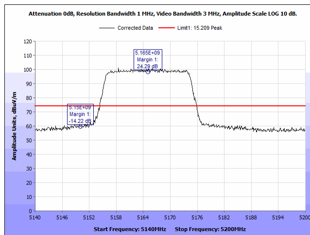
Plot 440. Radiated Band Edge, 5165MHz, BW20MHz, Peak, 90Sector Port1
