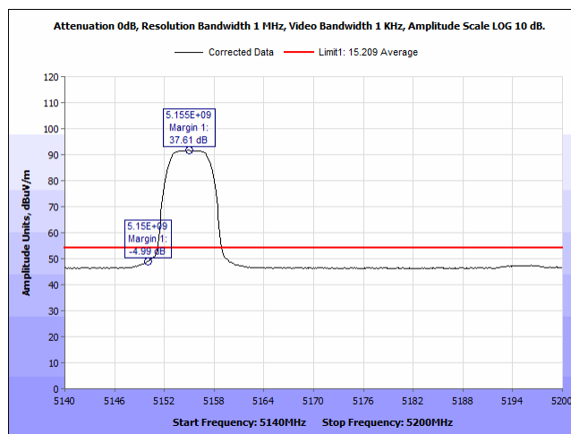
Plot 447. Radiated Band Edge, 5155MHz, BW5MHz, Average, 2Panel Port2
