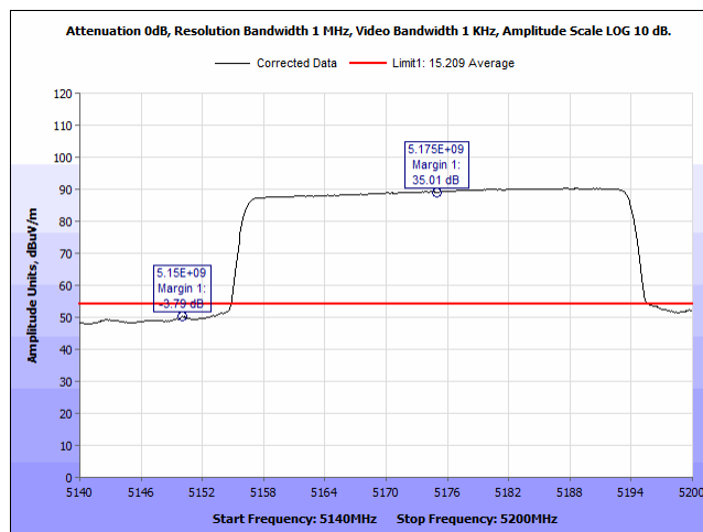
Plot 427. Radiated Band Edge, 5175MHz, BW40MHz, Average, 3Para Port2
