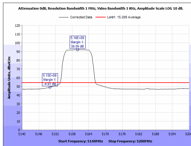
Plot 402. Radiated Band Edge, 5160MHz, BW10MHz, Average, 8Omni Port1
