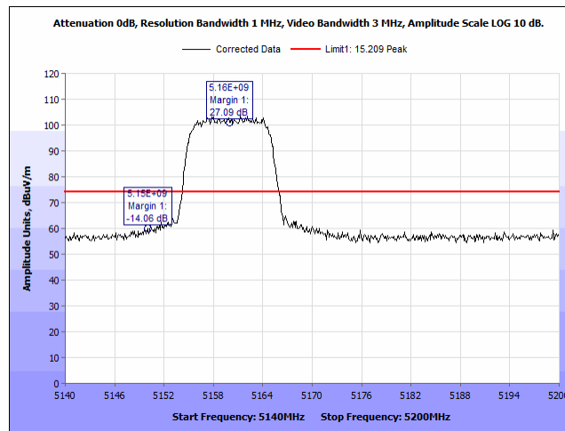
Plot 437. Radiated Band Edge, 5160MHz, BW10MHz, Peak, 90Sector Port2
