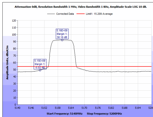
Plot 403. Radiated Band Edge, 5160MHz, BW10MHz, Average, 8Omni Port2
