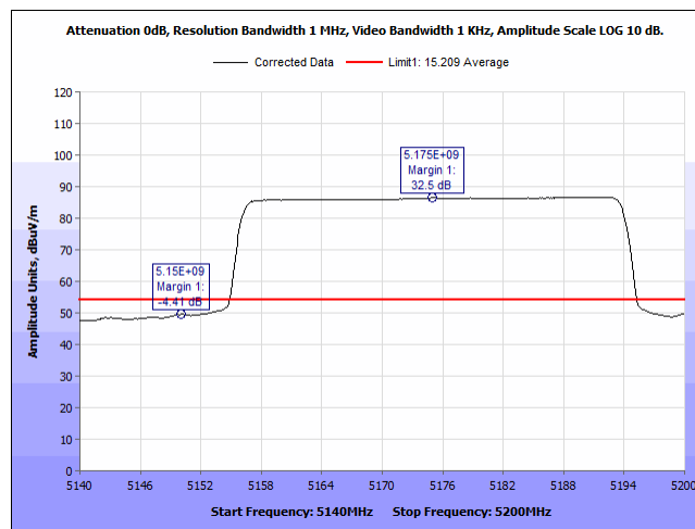
Plot 411. Radiated Band Edge, 5175MHz, BW40MHz, Average, 8Omni Port2
